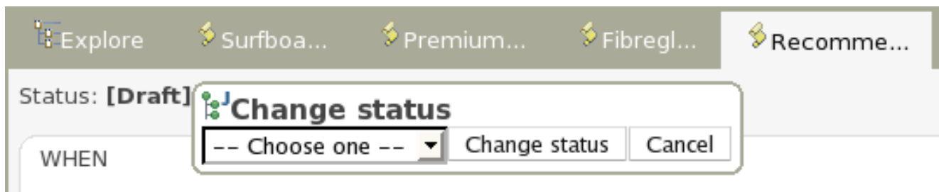
Figure 3.22. Asset status
