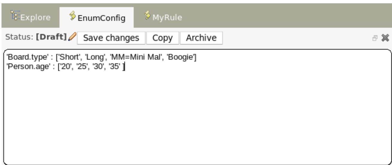
Figure 3.21. Data enumeration
