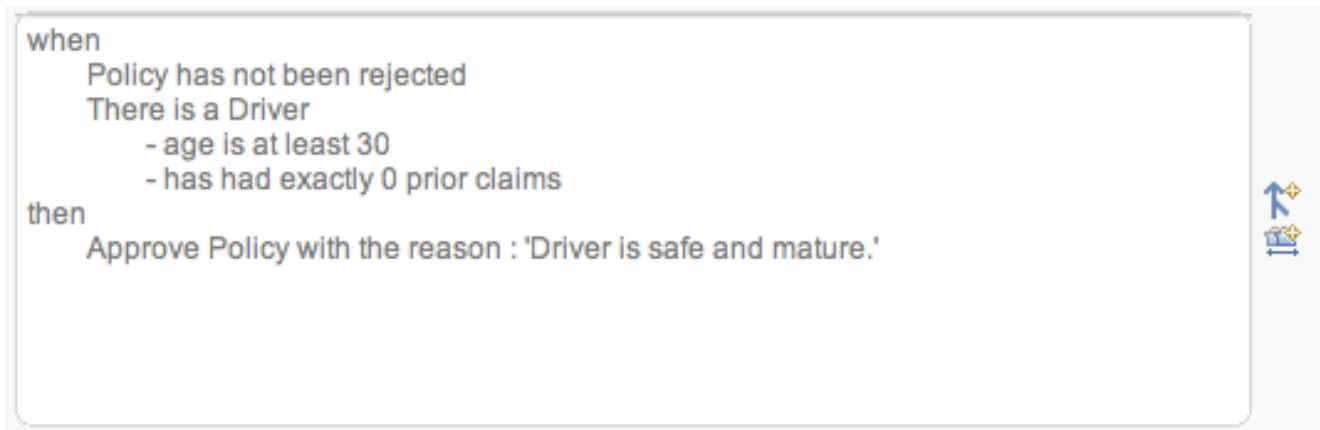
Figure 3.11. DSL rule
