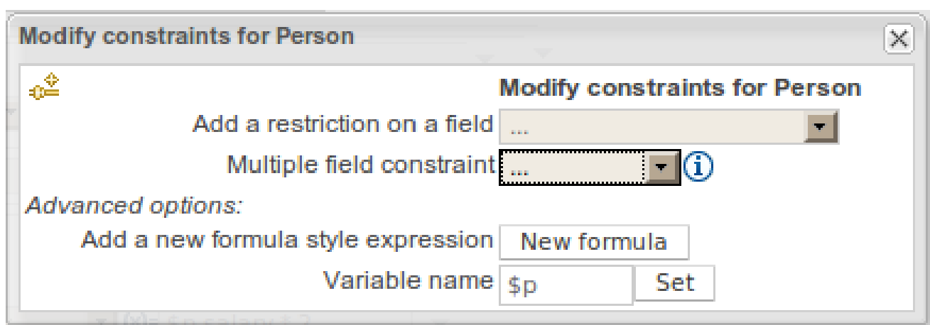
Figure 3.10. Adding constraints
