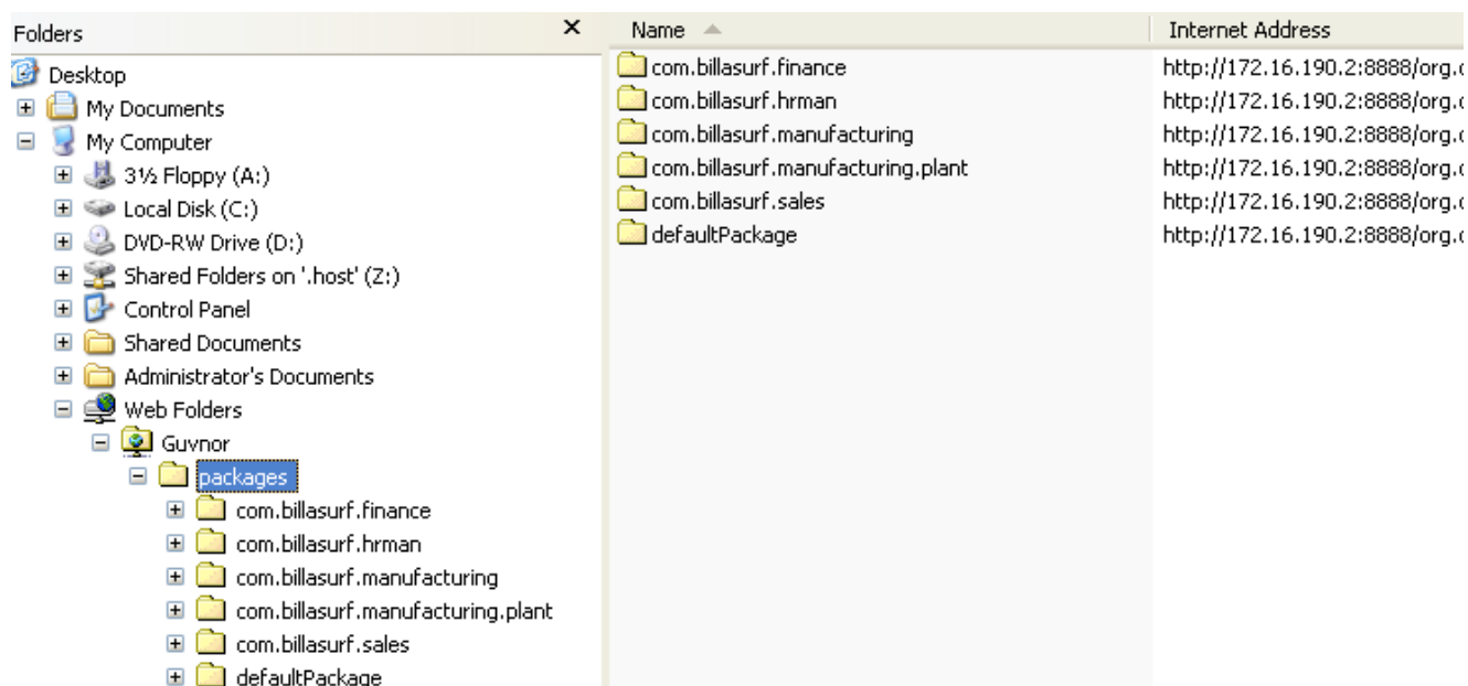
Figure 10.1. Windows webdav
