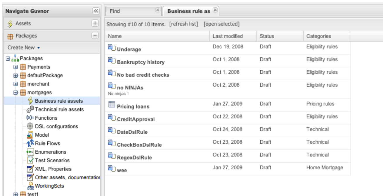
Figure 3.31. Package view
