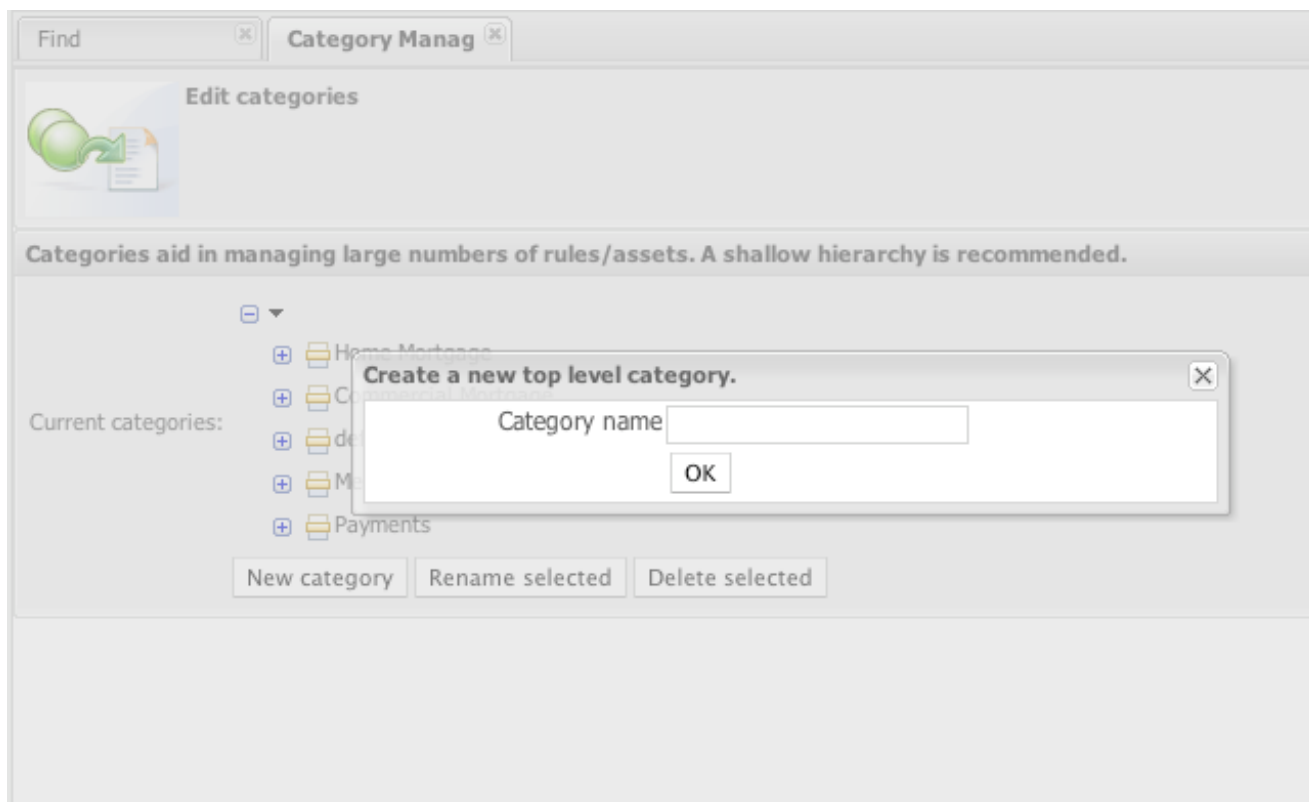
Figure 3.3. Creating categories
