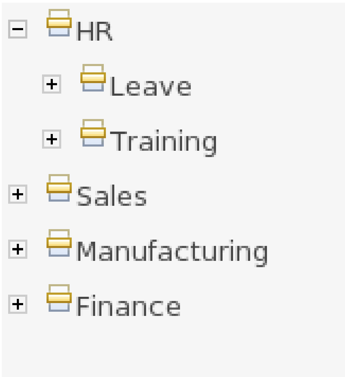
Figure 3.1. Categories
