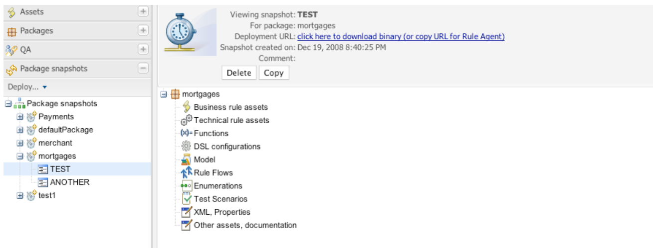
Figure 3.29. Deployment snapshots
