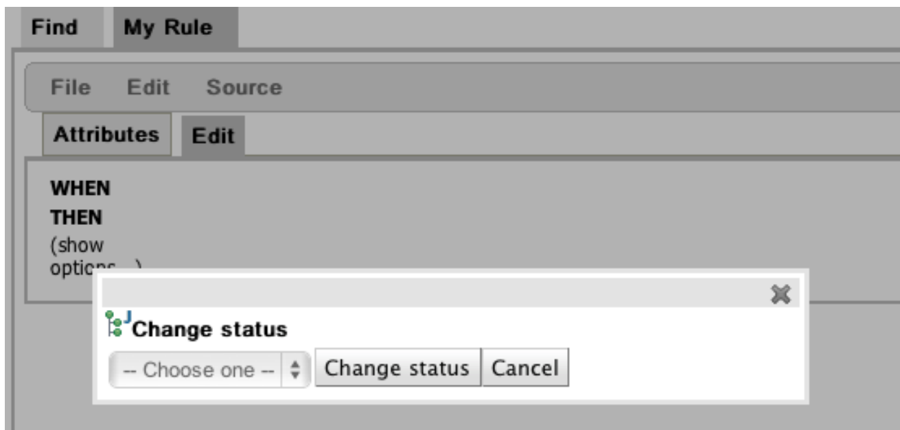
Figure 3.35. Asset status
