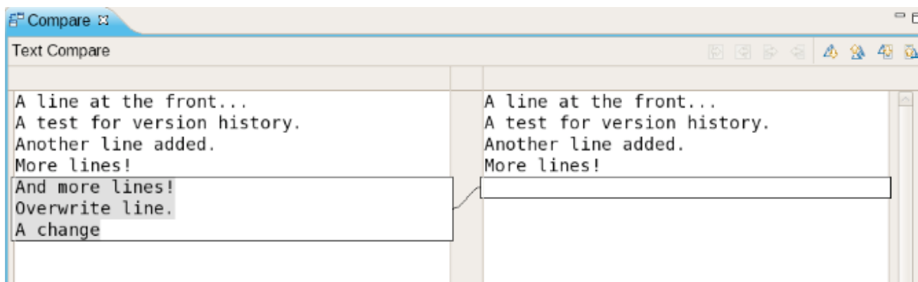
Figure 12.16. Compare
