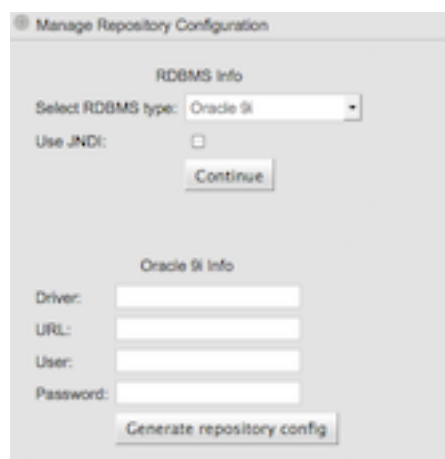
Figure 14.3. RDBMS information
