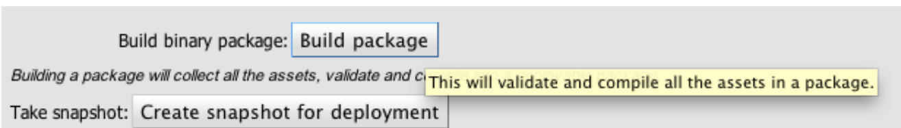
Figure 3.40. Package building
