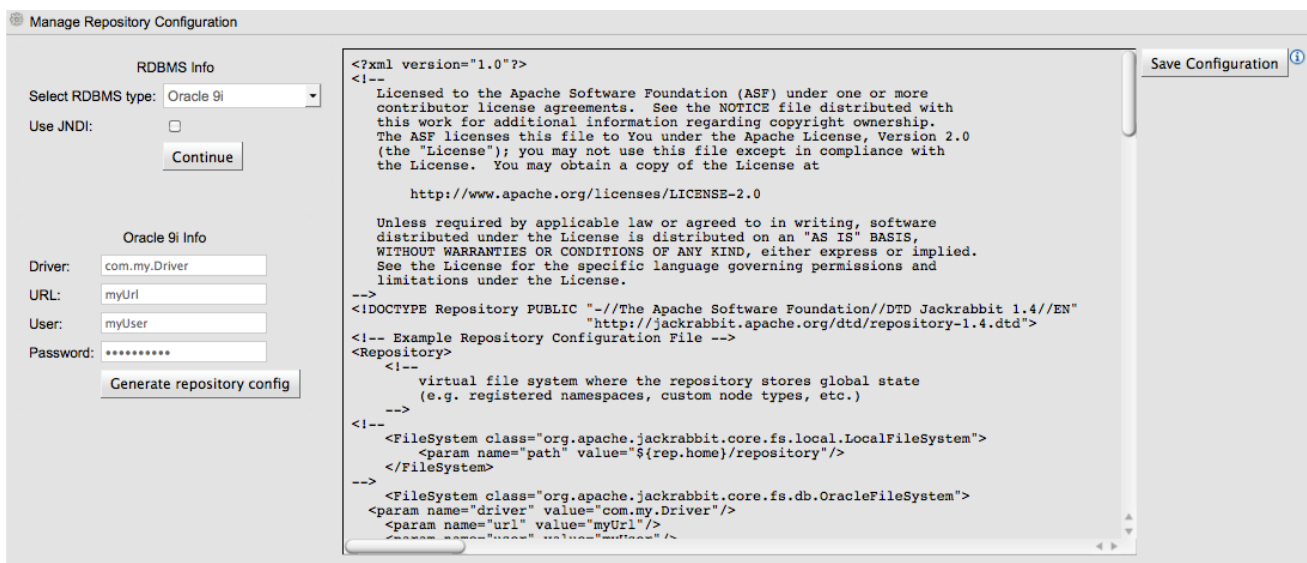
Figure 14.4. Generated repository.xml
