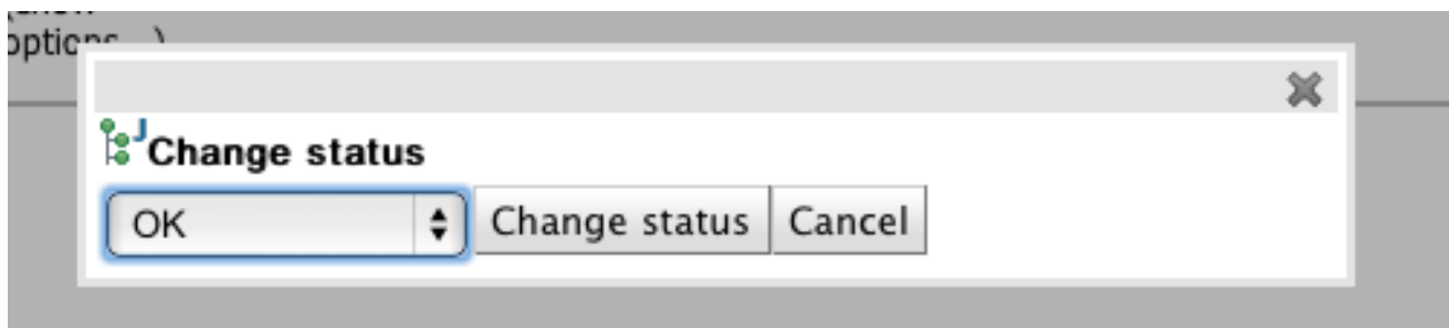
Figure 3.36. Asset status
