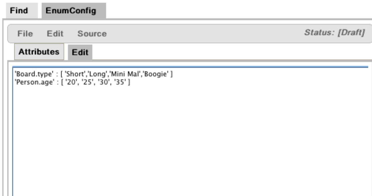
Figure 3.34. Data enumeration
