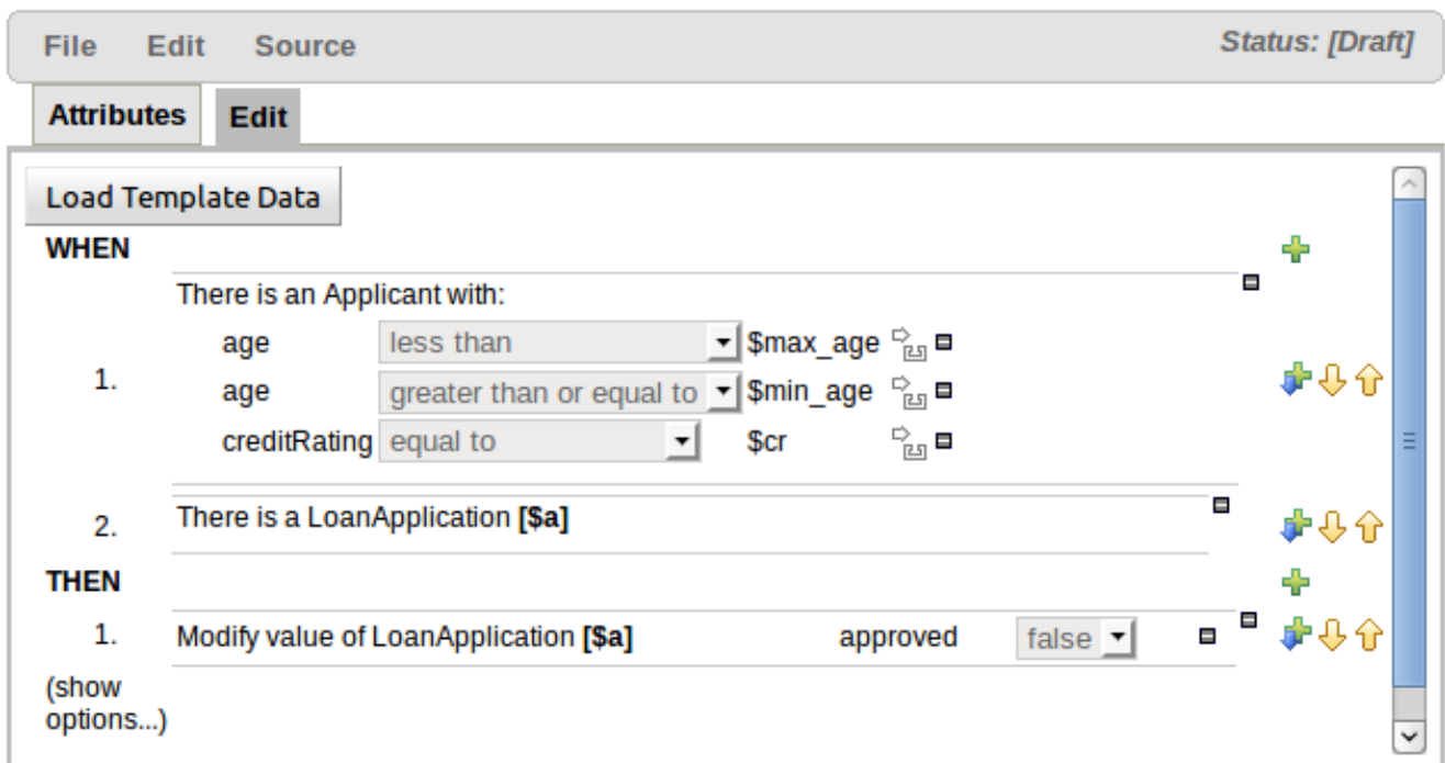
Figure 3.27. Rule template in the guided editor
