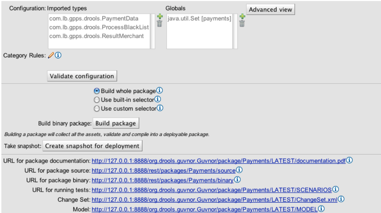
Figure 3.39. Package configuration
