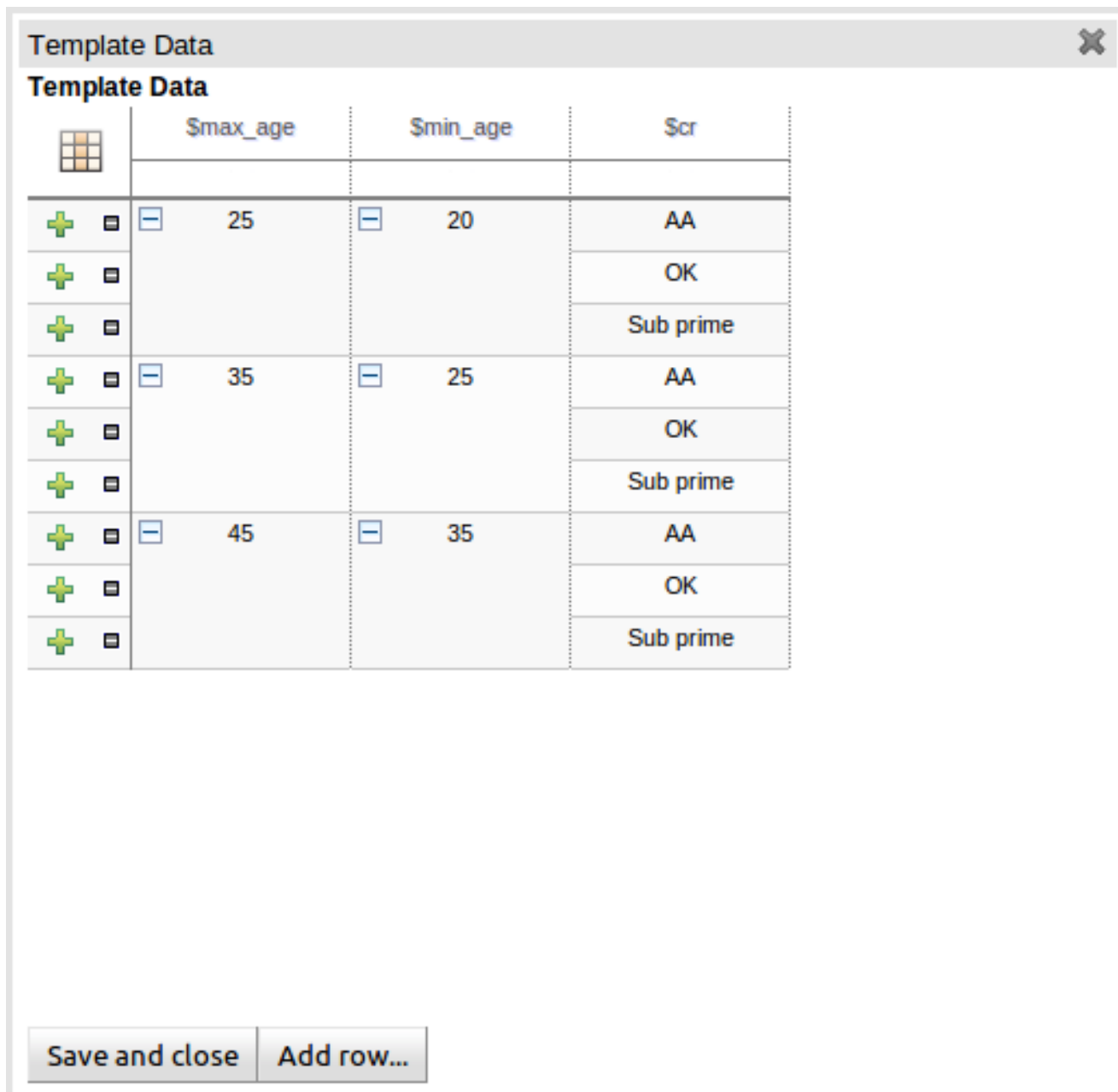
Figure 3.29. Cell merging
