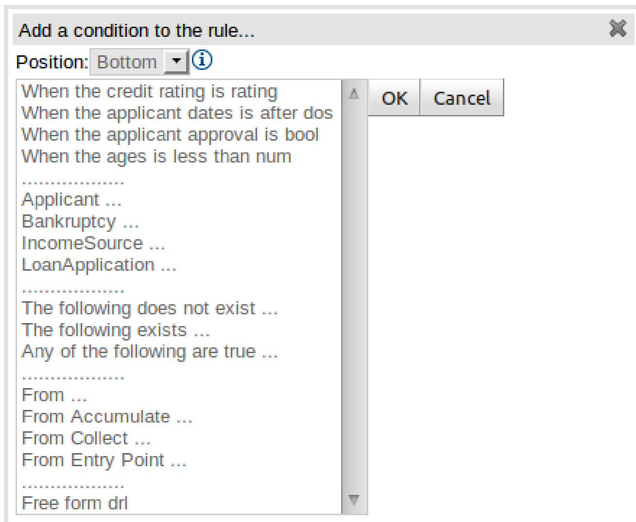
Figure 3.14. Adding Patterns
