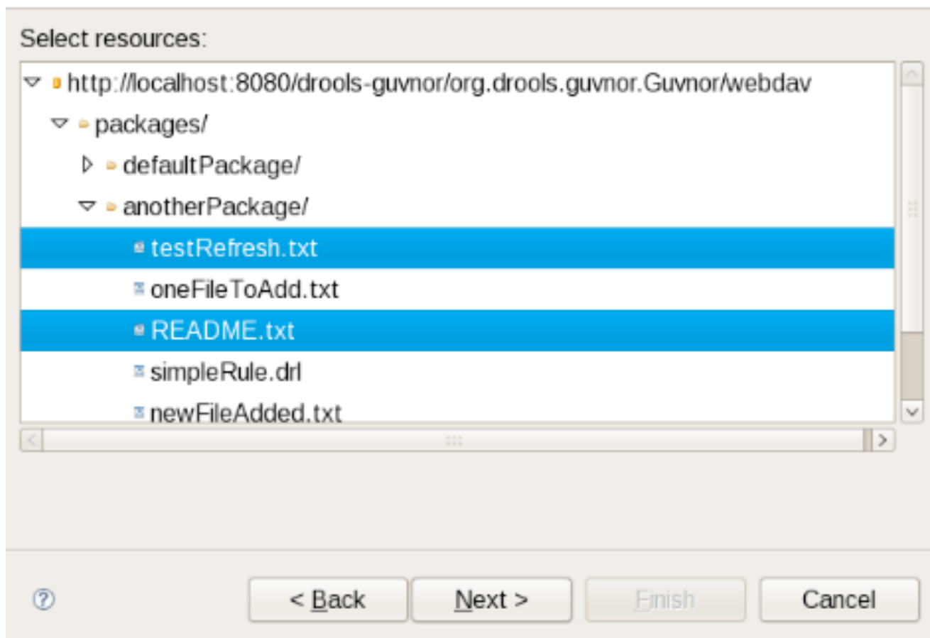
Figure 12.21. Import
