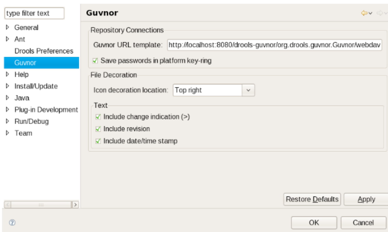
Figure 12.24. Preferences
