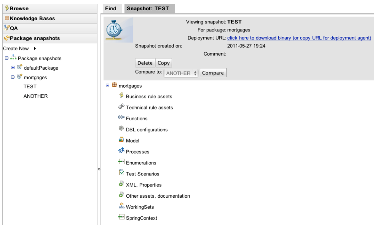
Figure 3.42. Deployment snapshots
