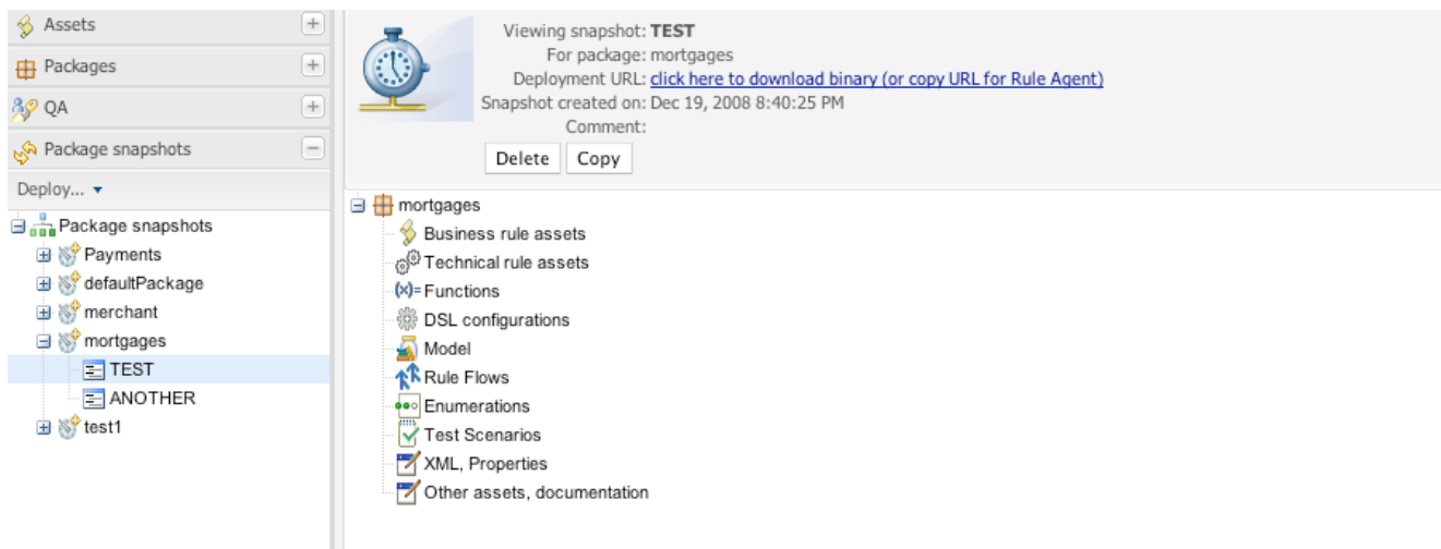
Figure 9.1. Snapshot deployment
