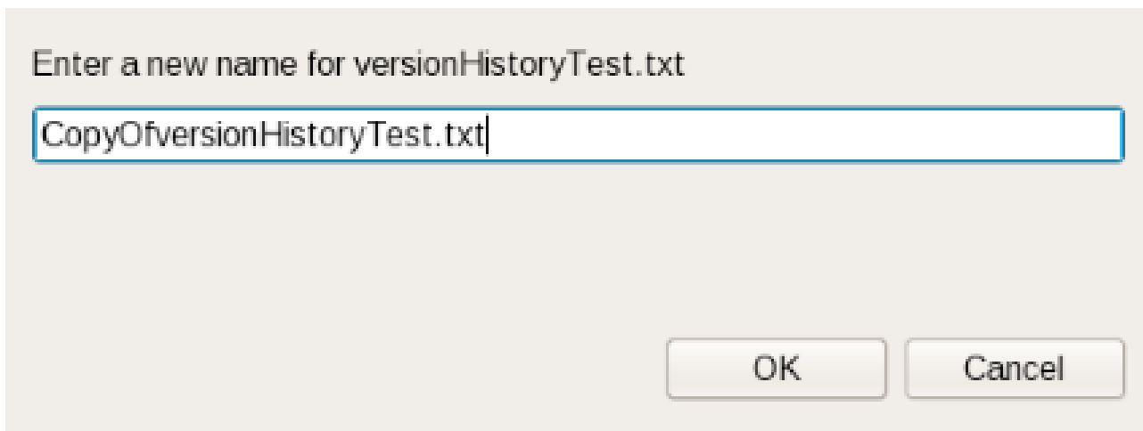
Figure 12.23. Copy
