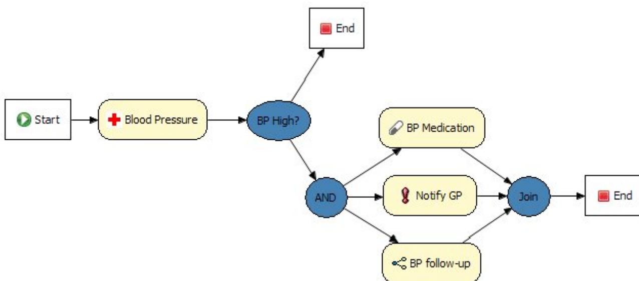
Figure 2.42. Work items
