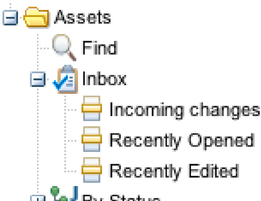
Figure 2.10. Inbox Categories
