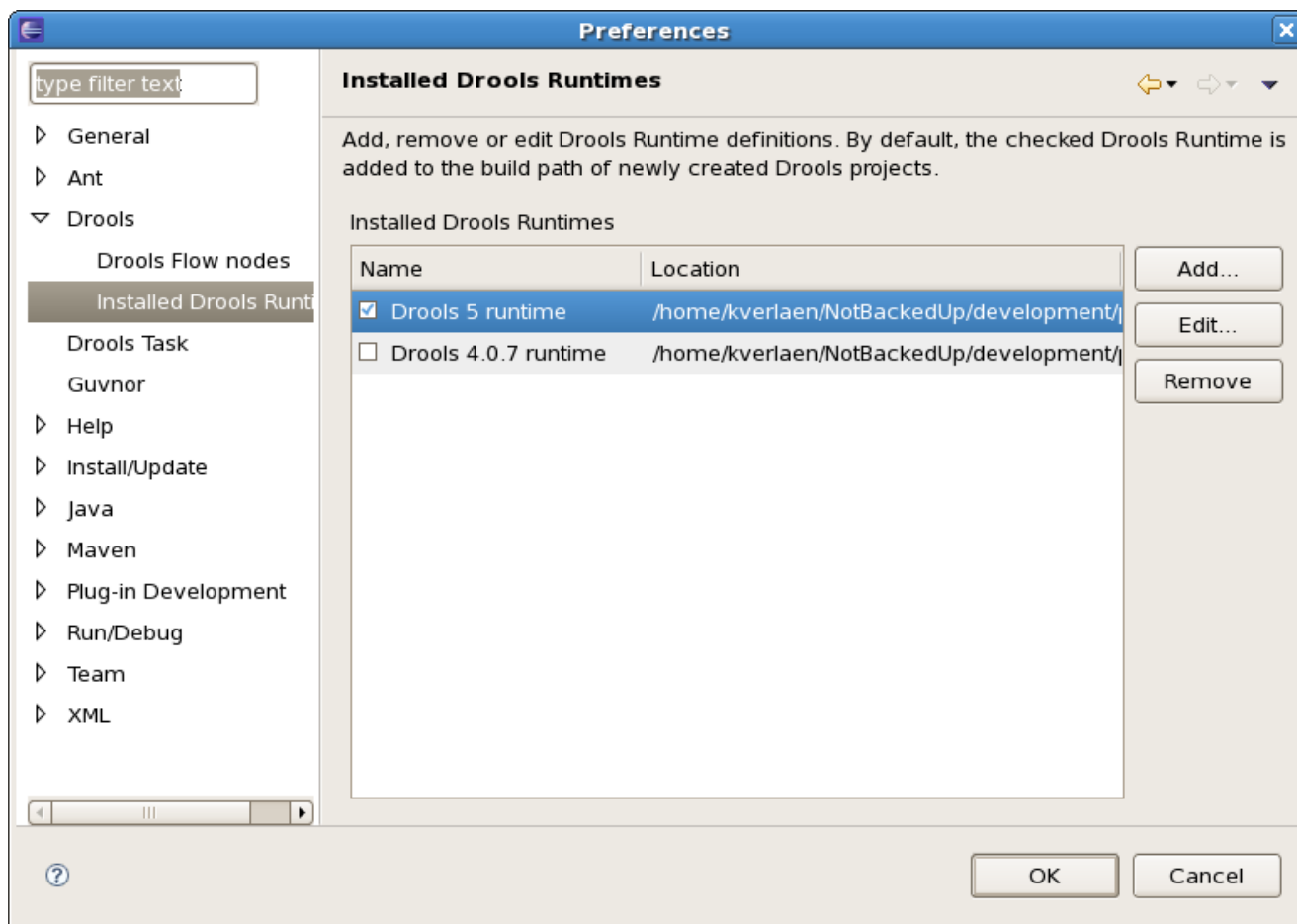
Figure 2.44. Run times
