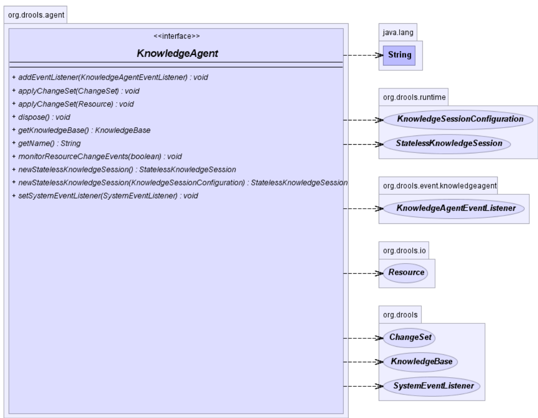
Figure 4.7. KnowledgeAgent
