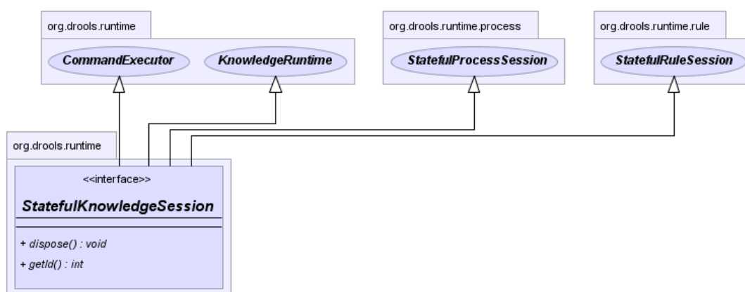
Figure 4.9. StatefulKnowledgeSession
