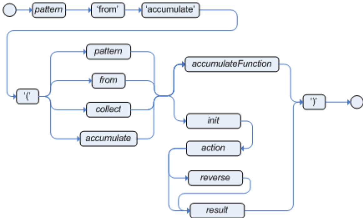
Figure 5.28. accumulate
