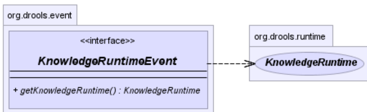
Figure 4.24. KnowledgeRuntimeEvent
