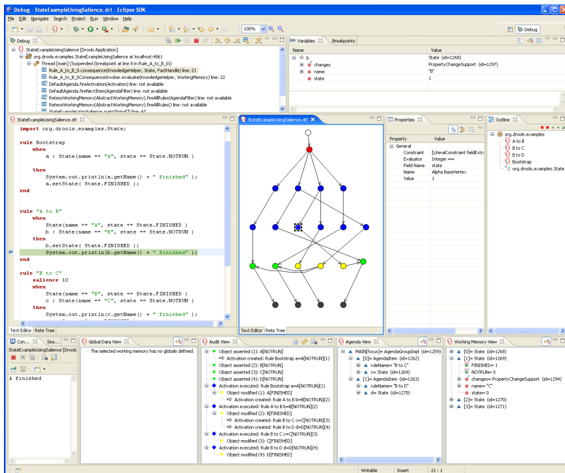
Figure 8.10. Debugging
