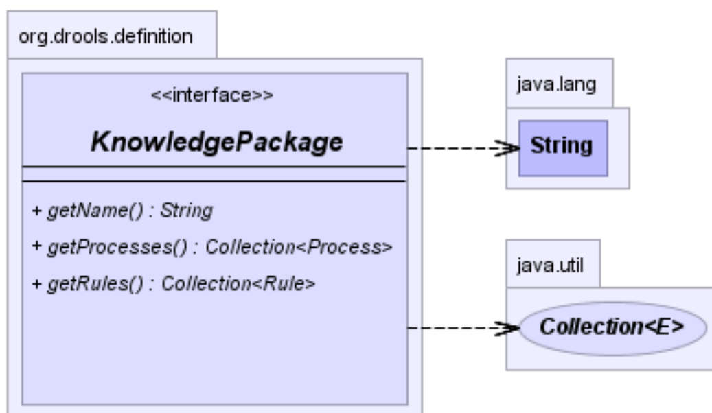
Figure 4.4. KnowledgePackage
