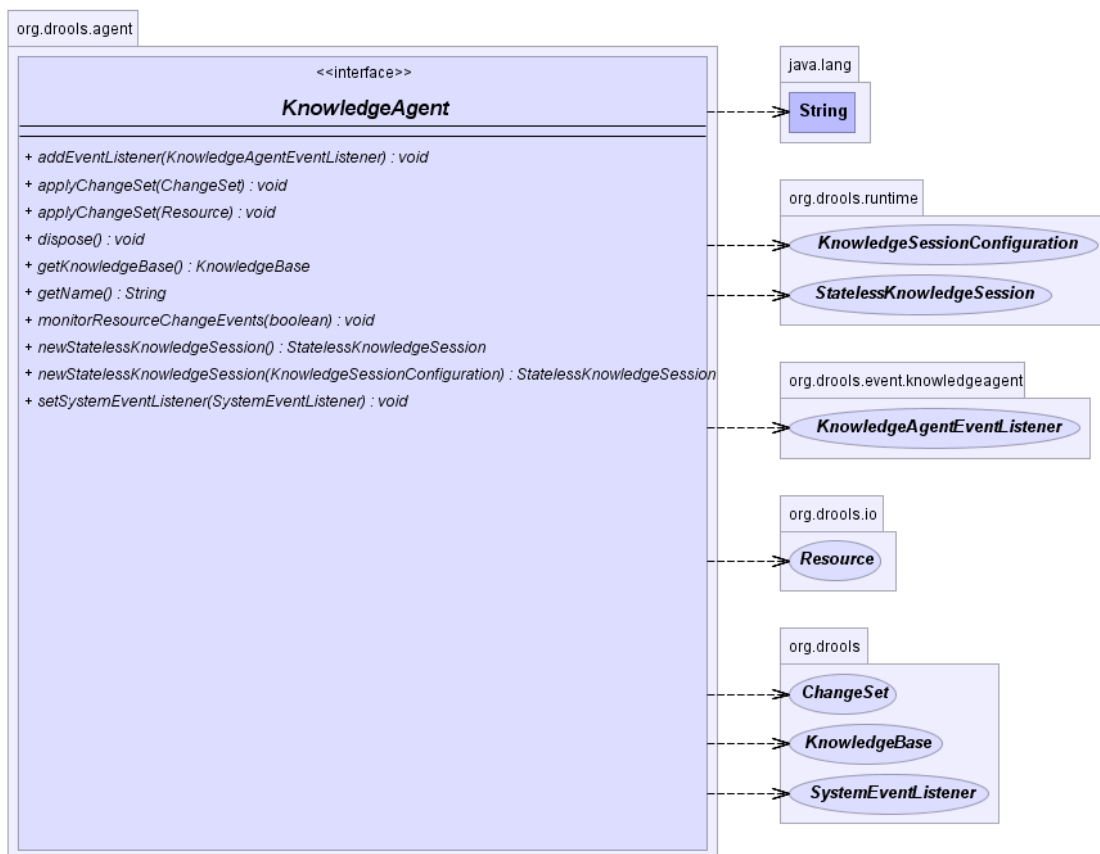
Figure 4.7. KnowledgeAgent
