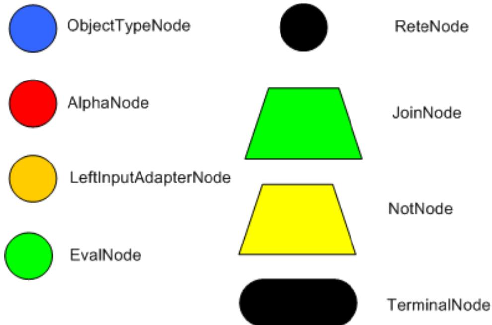
Figure 3.3. Rete Nodes
