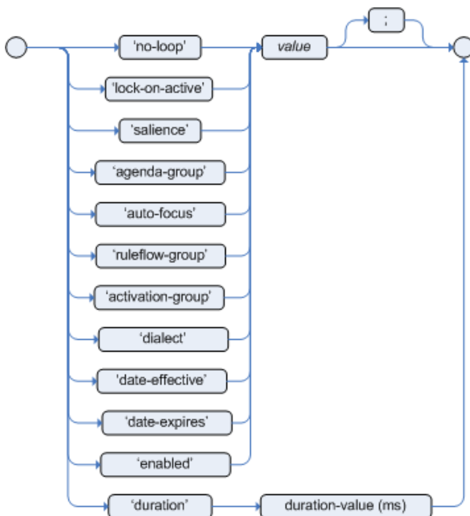
Figure 5.11. rule attributes
