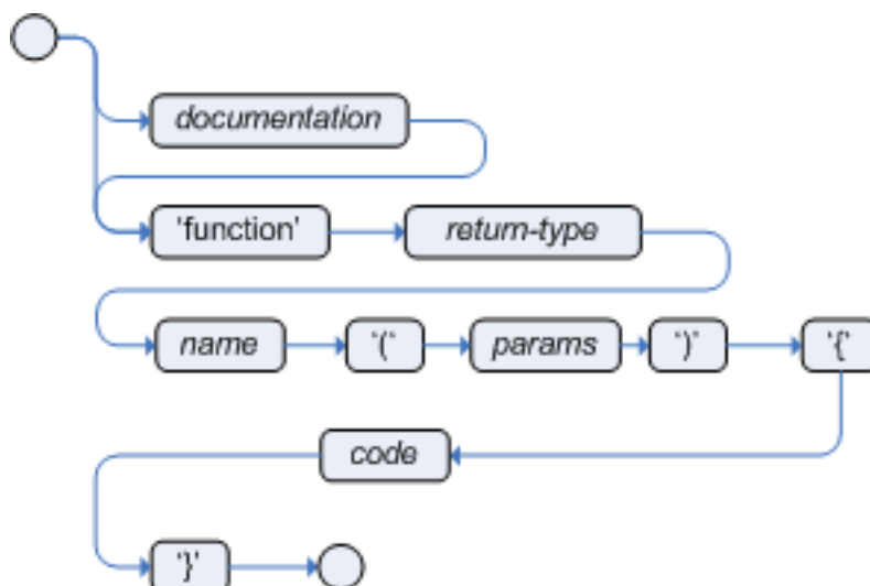
Figure 5.7. function
