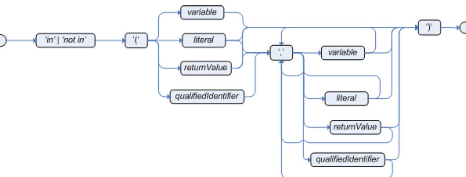
Figure 5.17. compoundValueRestriction
