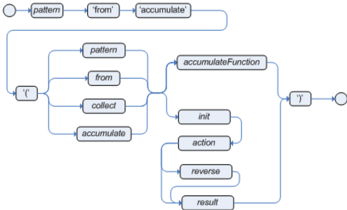
Figure 5.28. accumulate
