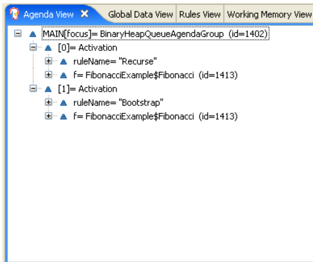
Figure 9.7. Fibonacci Example: "Recurse" Agenda View 1
