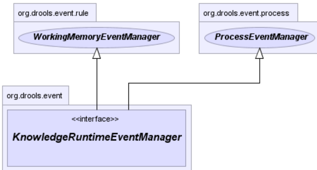
Figure 4.22. KnowledgeRuntimeEventManager
