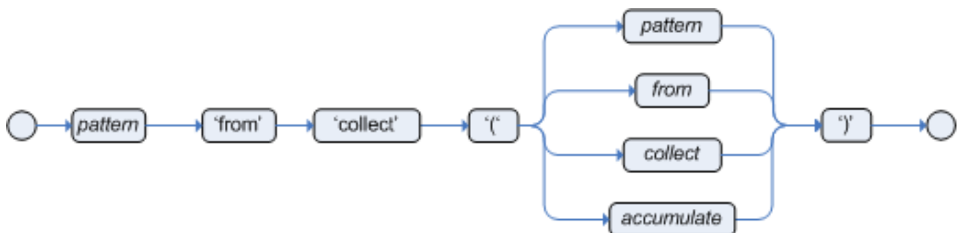
Figure 5.27. collect
