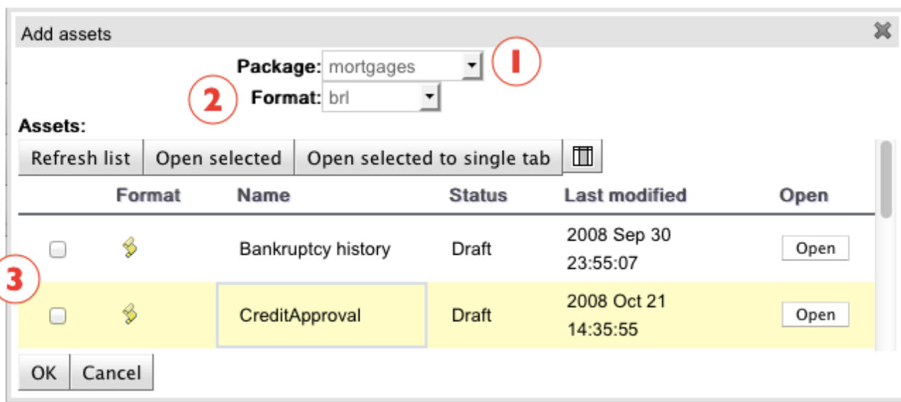
Figure 4.88. Adding Assets resources
