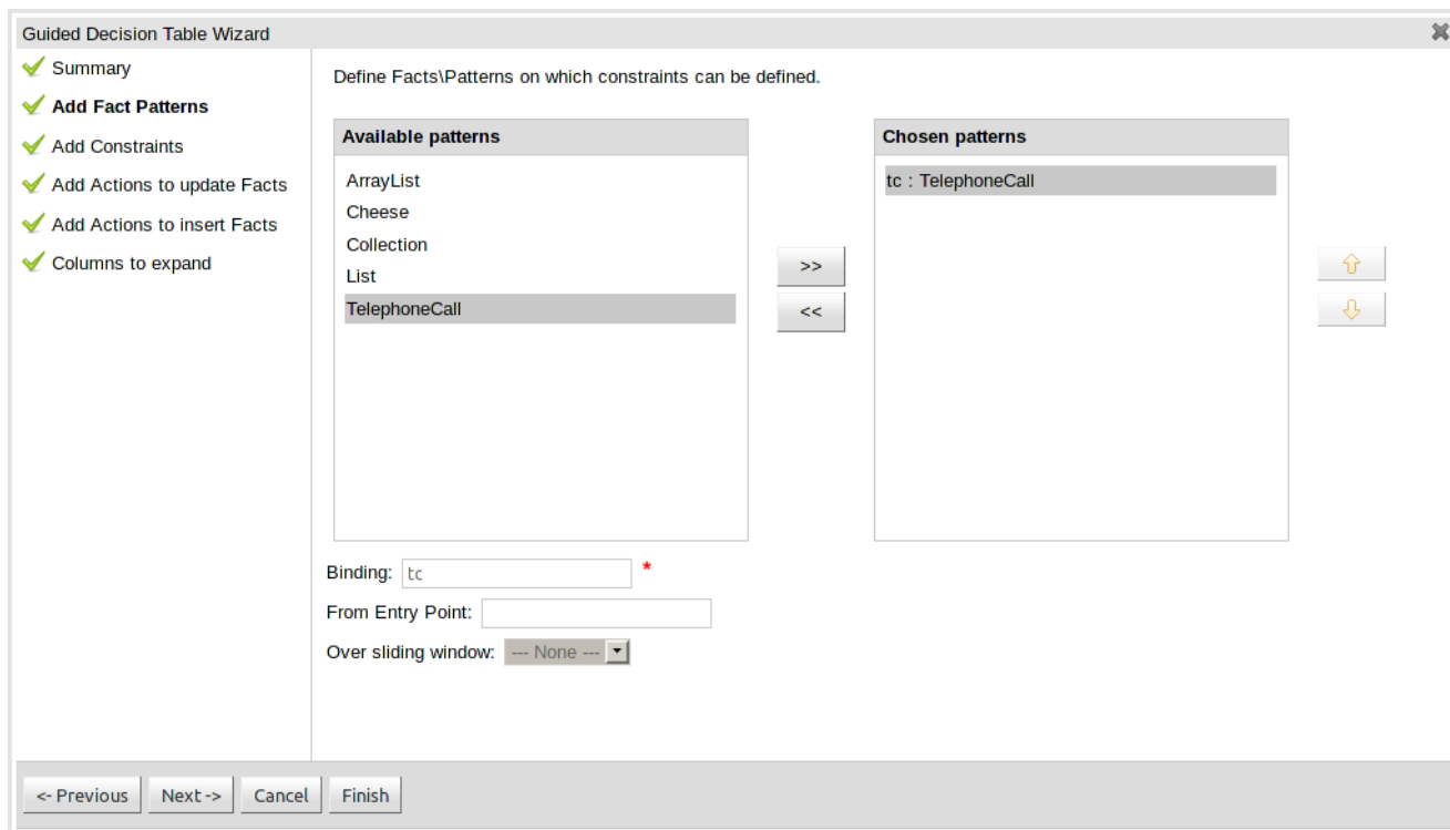
Figure 4.39. Add Fact Patterns page
