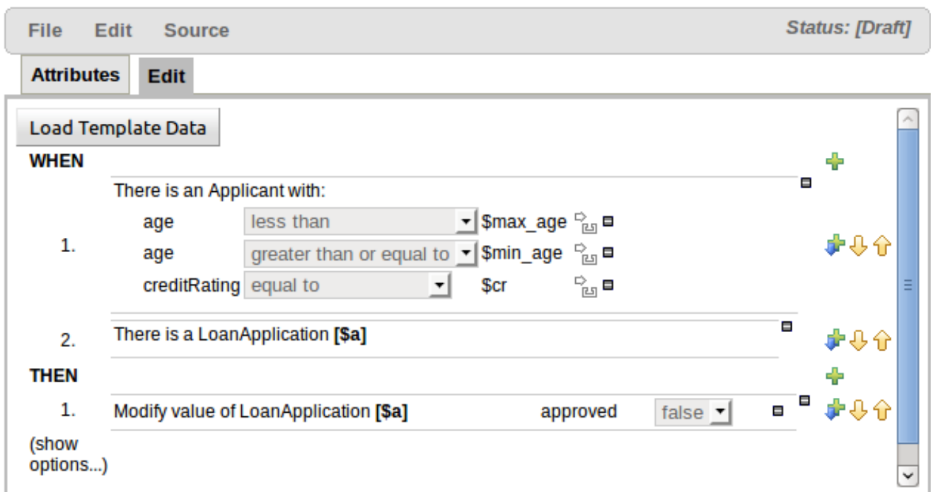
Figure 4.51. Rule template in the guided editor
