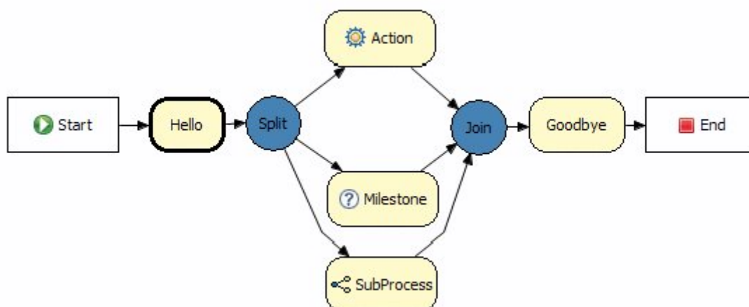
Figure 4.102. Current active nodes in a workflow in a specific breakpoint
