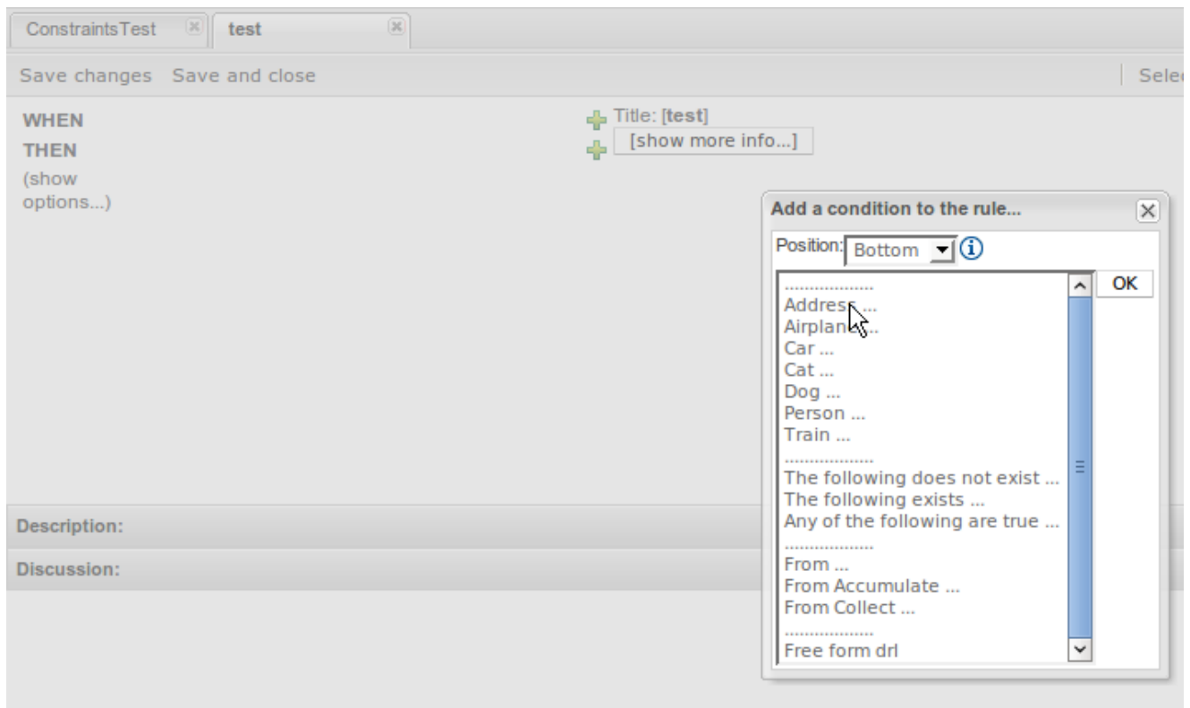
Figure 4.83. Without the Working Set all types are visible
