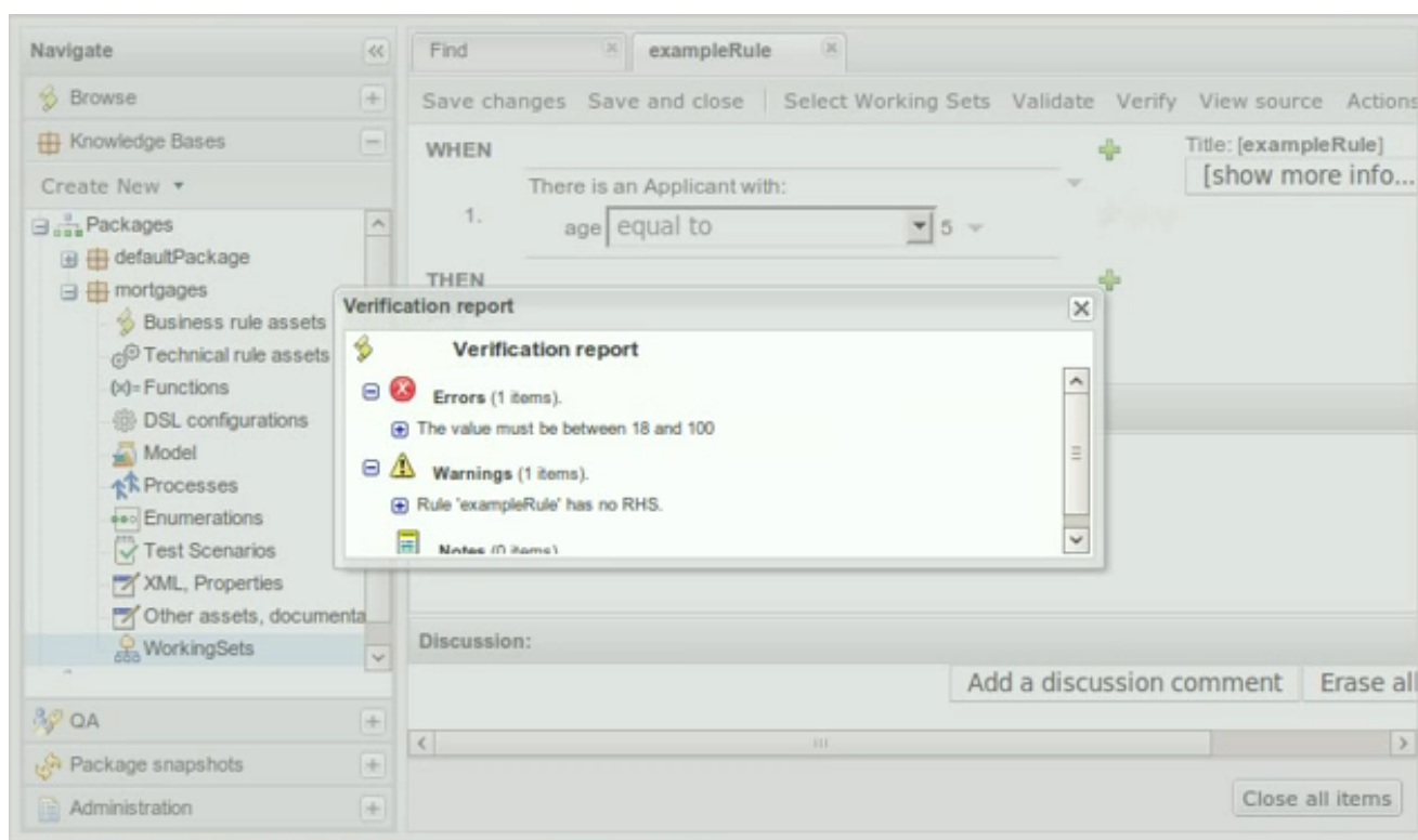
Figure 4.90. A age of 5 is invalid
