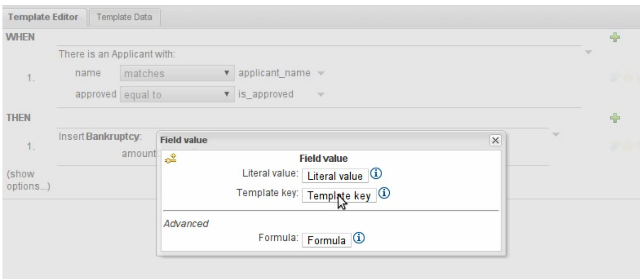
Figure 4.78. Adding a Template Key in the "THEN" Section
