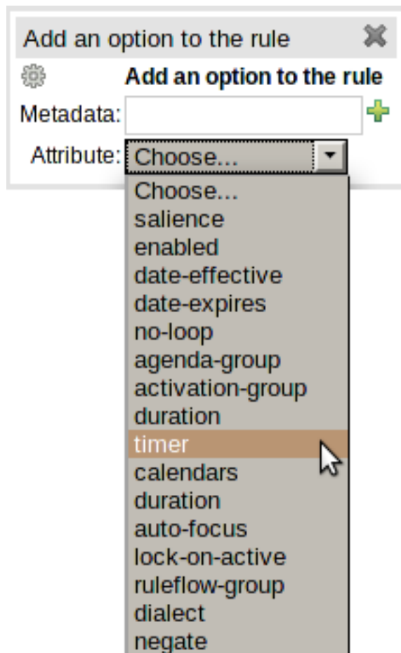
Figure 4.34. Timer and Calendar
