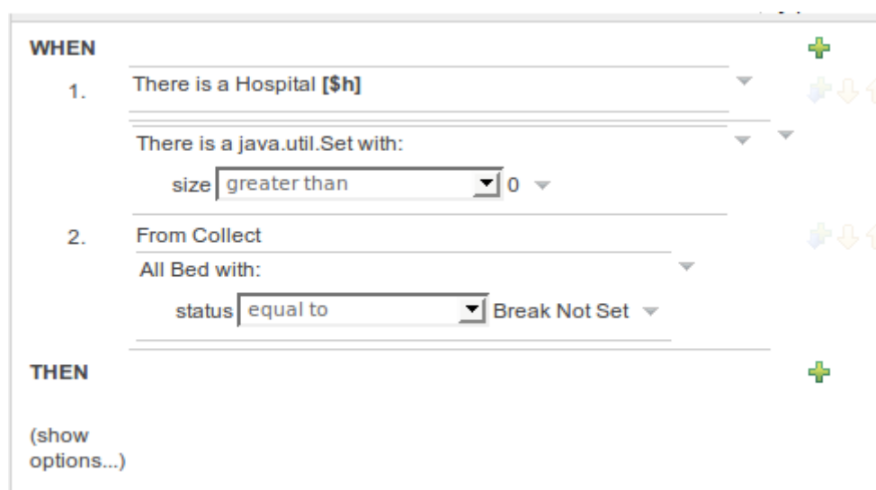
Figure 4.75. From Collect CE Builder
