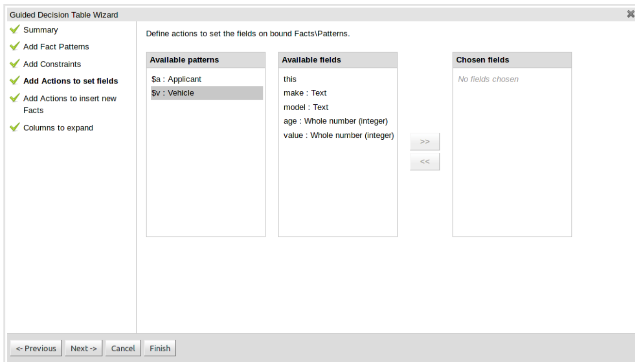
Figure 4.53. Add actions to set fields on bound facts
