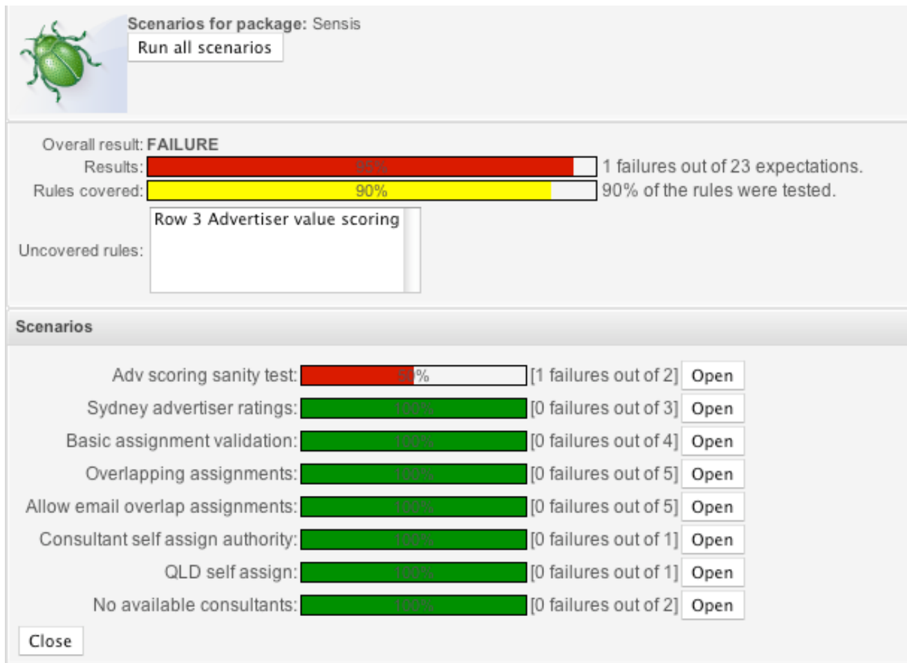
Figure 4.97. Running all scenarios
