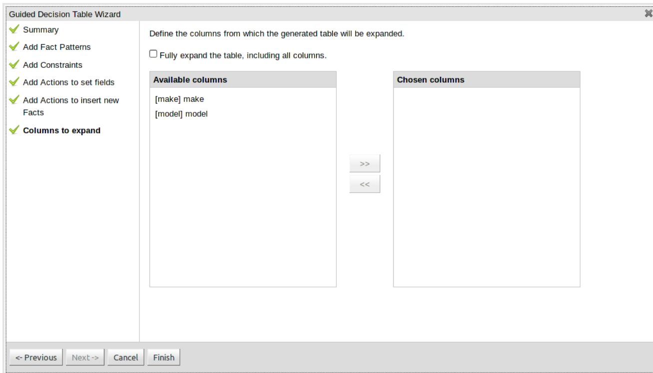
Figure 4.56. Choose how rows are created - select the columns you want to expand upon
