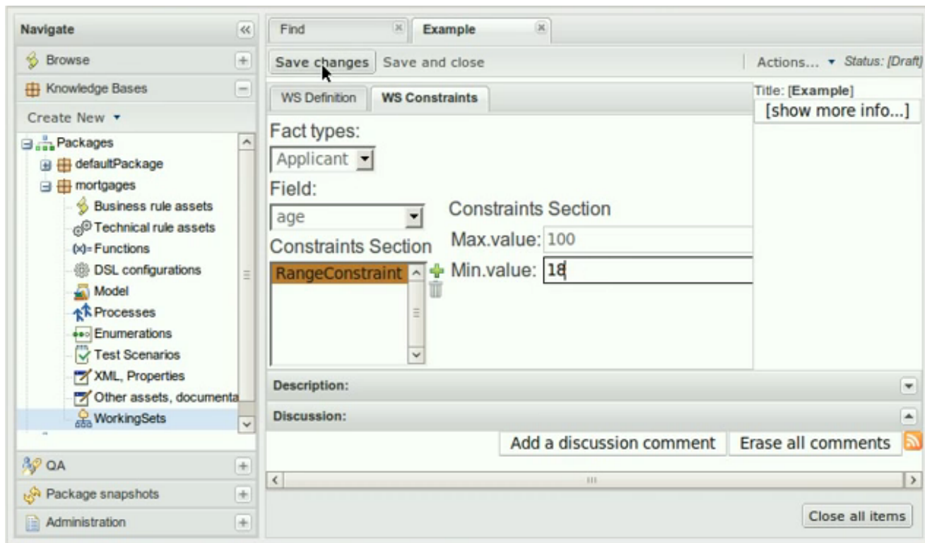
Figure 4.88. A example range constraint
