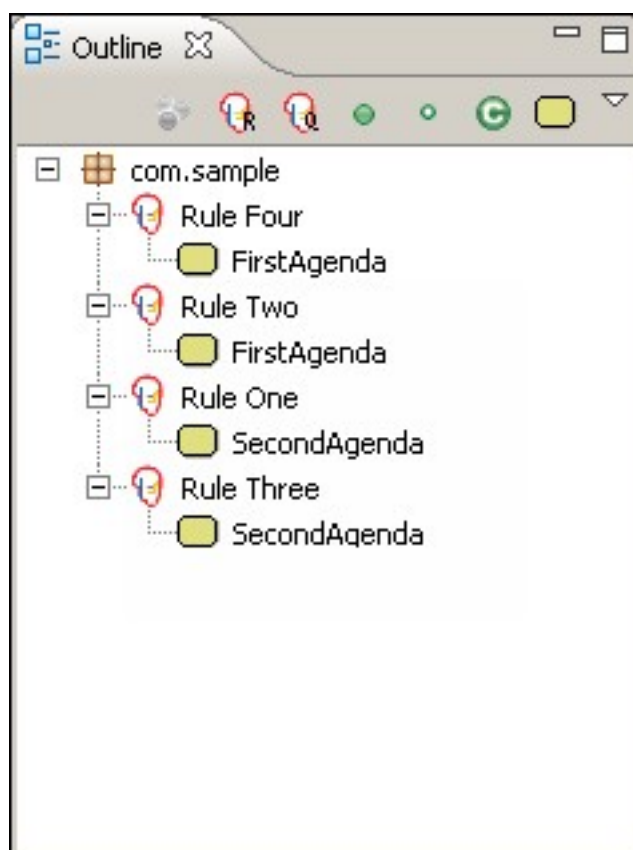
Figure 4.94. Sort by Agenda Group
