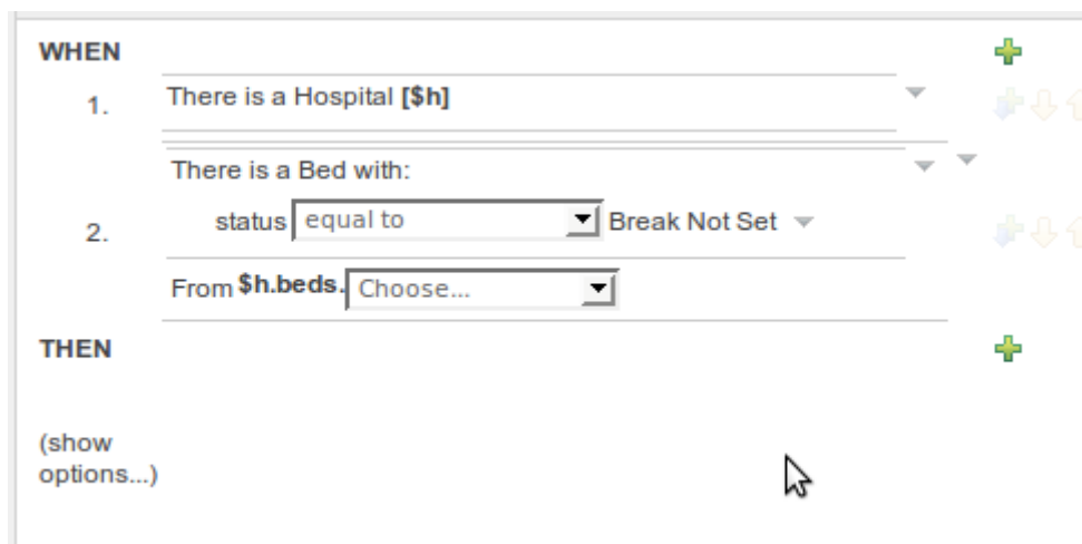
Figure 4.74. From CE Builder
