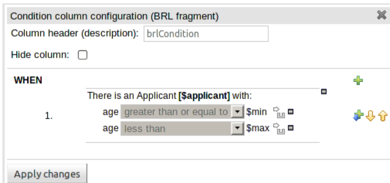
Figure 4.27. A Condition BRL fragment
