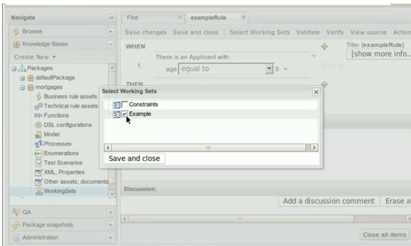
Figure 4.89. Select the working set to validate the age field
