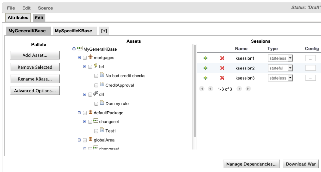
Figure 4.41. The new Service Editor
