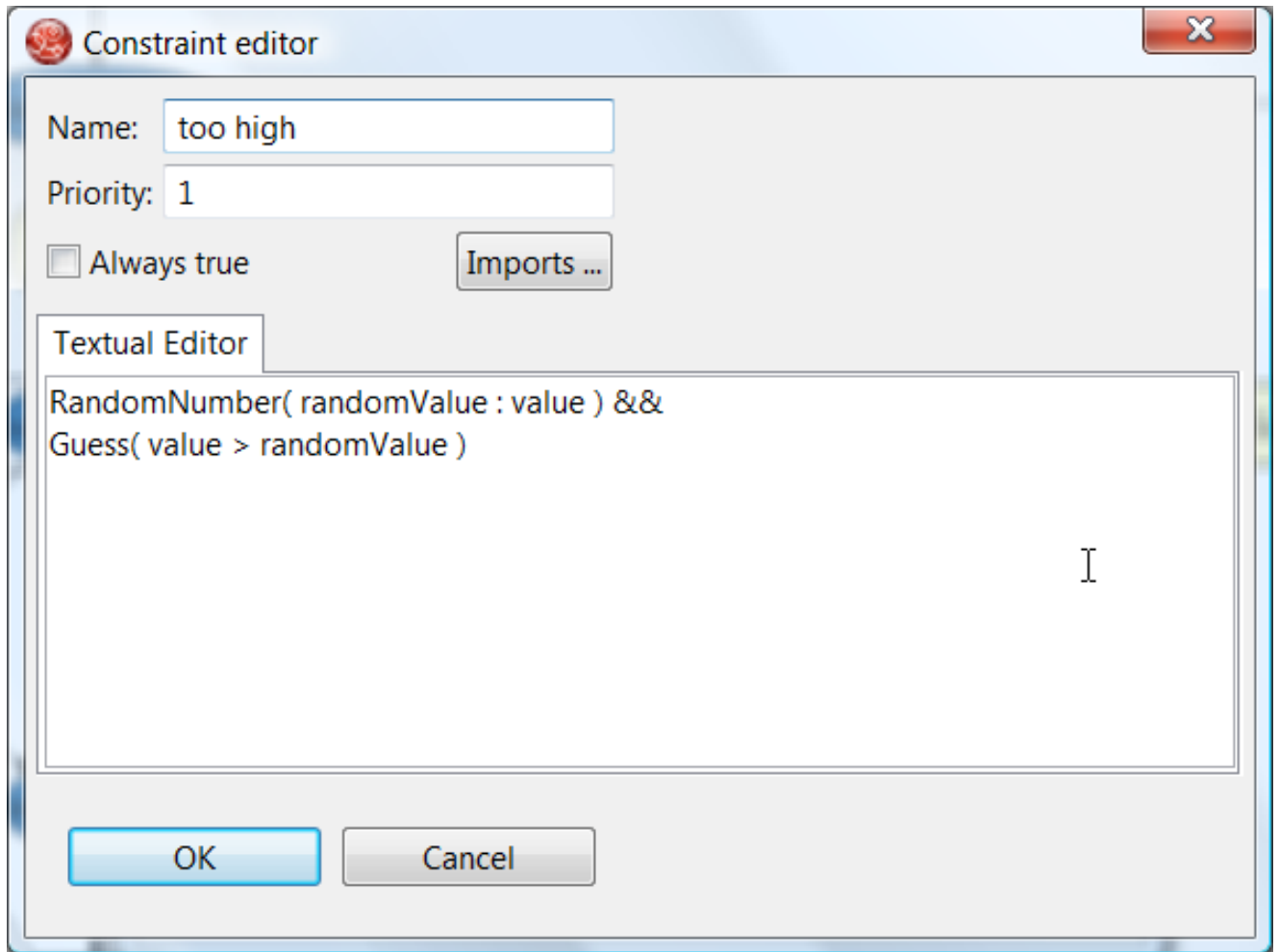
Figure 7.21. Constraint Editor for the "Guess Correct" Node: value too high
