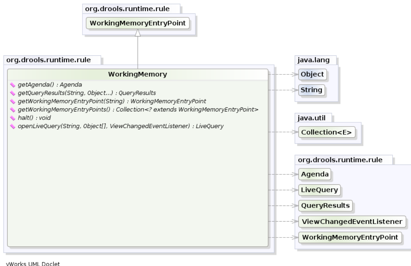
Figure 3.11. WorkingMemory
