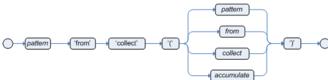
Figure 4.26. collect
