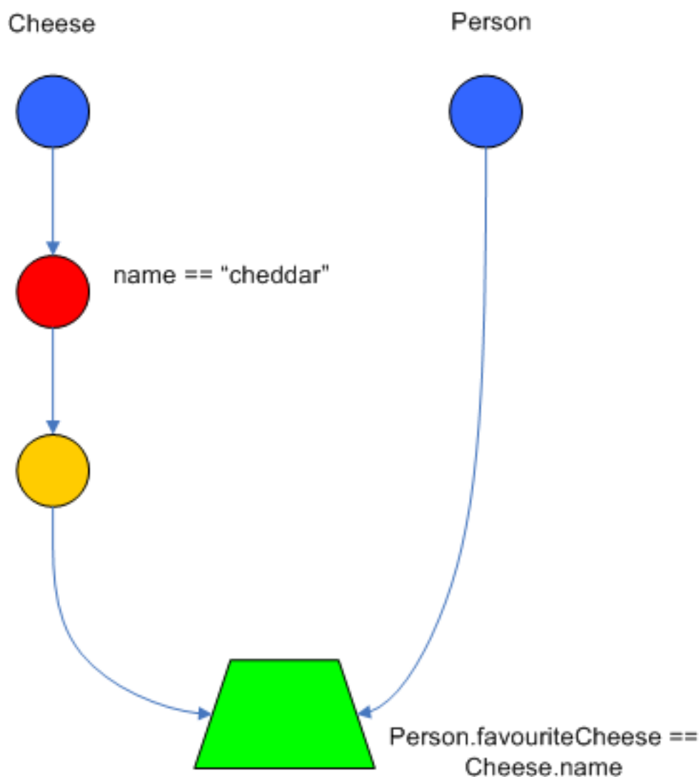
Figure 1.10. JoinNode
