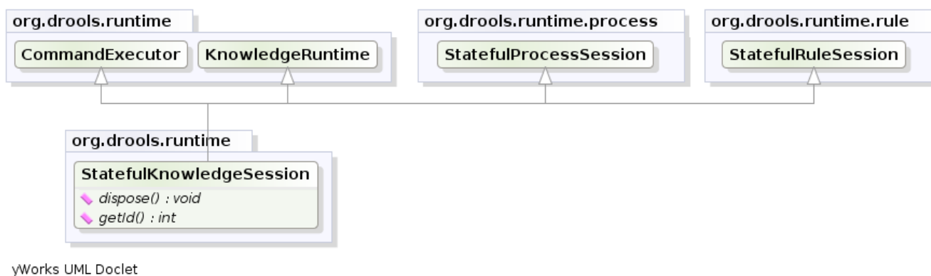
Figure 3.9. StatefulKnowledgeSession
