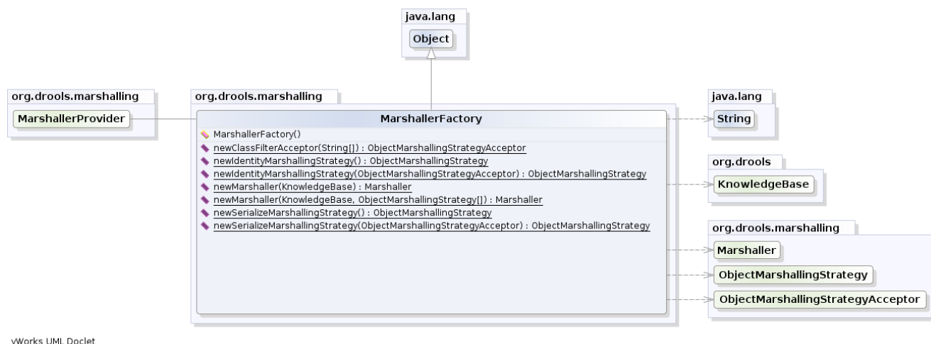
Figure 3.29. MarshallerFactory
