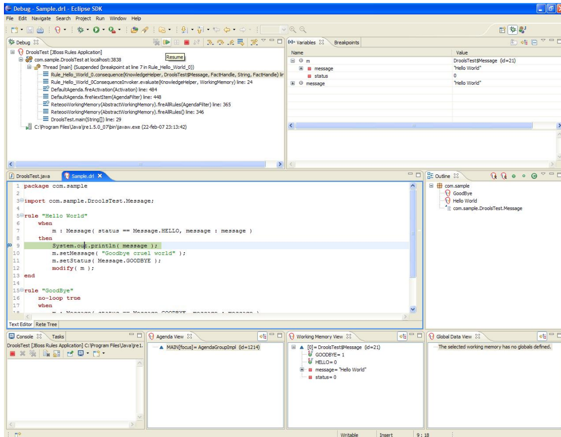
Figure 6.13. Debugging
