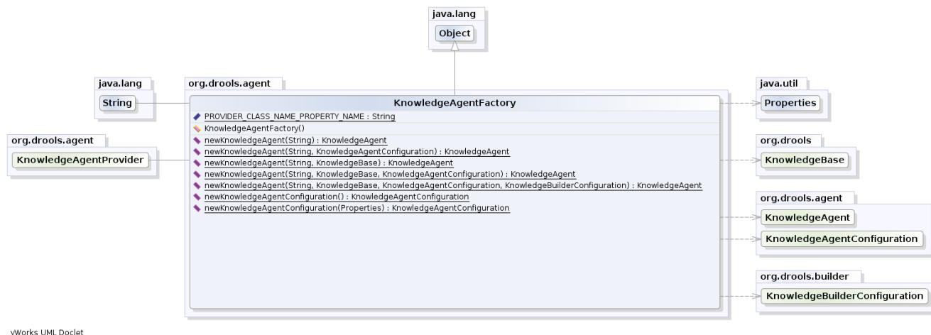
Figure 3.8. KnowledgeAgentFactory
