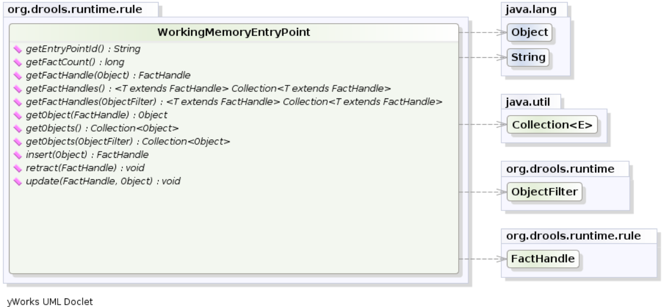
Figure 3.10. WorkingMemoryEntryPoint
