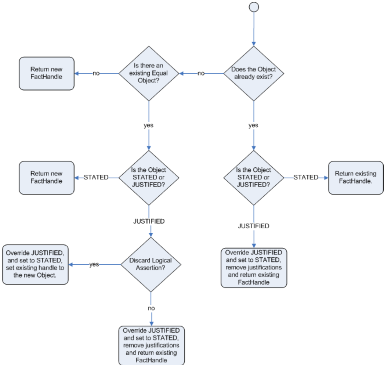
Figure 2.1. Stated Insertion
