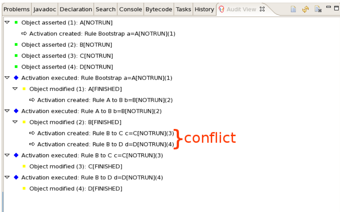
Figure 7.4. Saliency State Example Audit View
