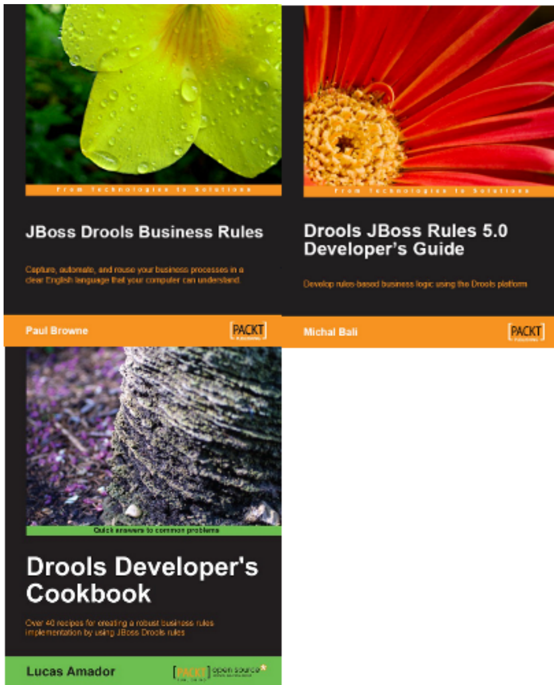
Figure 1.6. Recommended Reading
