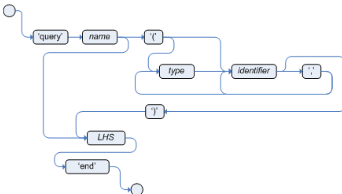
Figure 4.29. query
