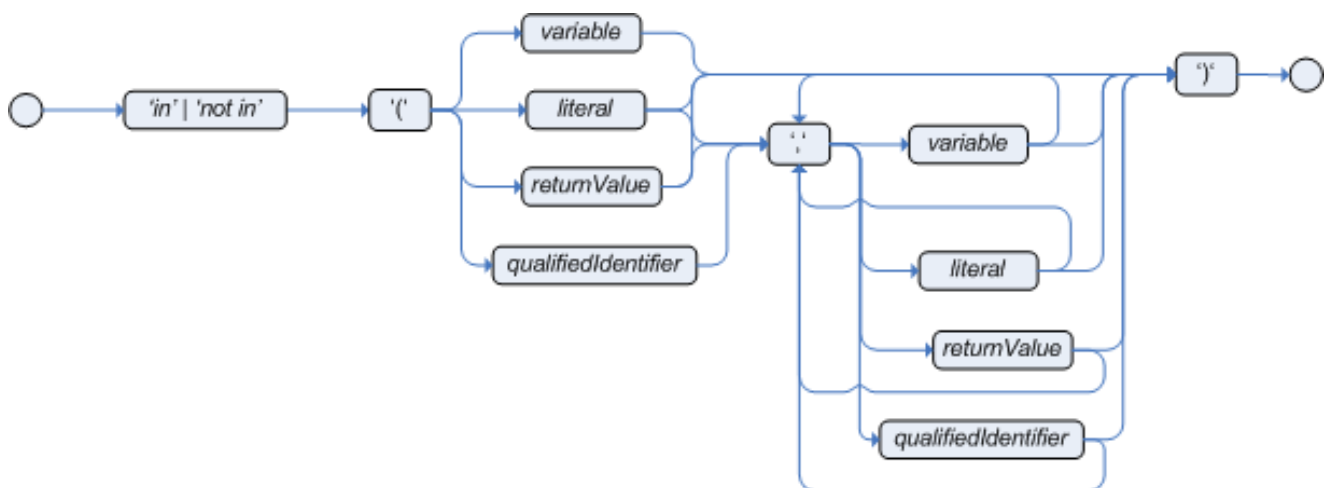
Figure 4.16. compoundValueRestriction
