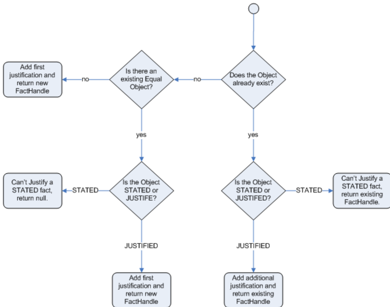
Figure 2.2. Logical Insertion
