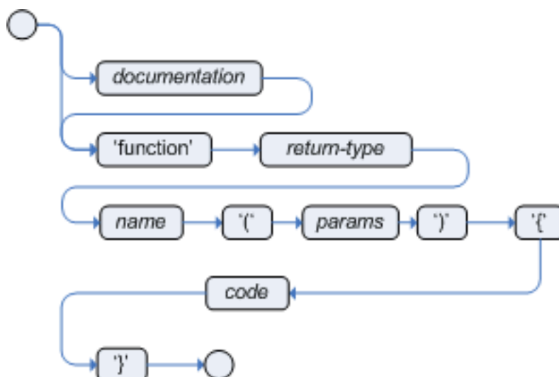
Figure 4.6. function
