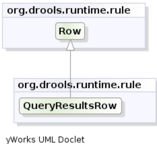
Figure 3.13. QueryResultsRow
