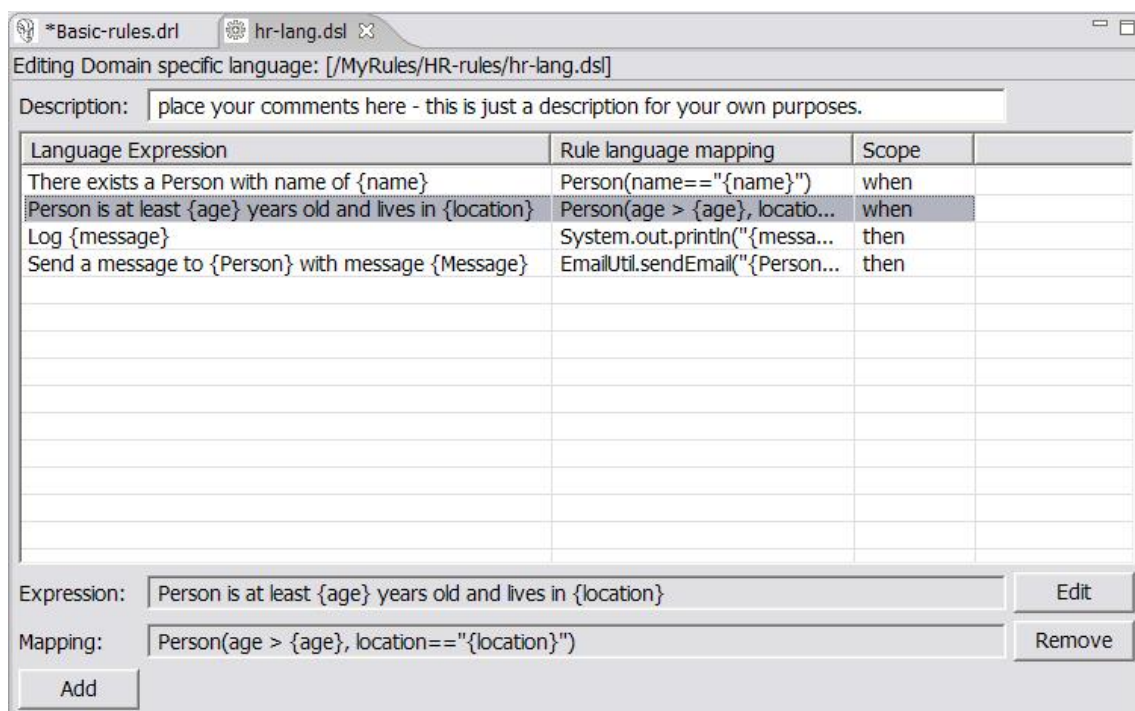
Figure 6.8. The Domain Specific Language editor
