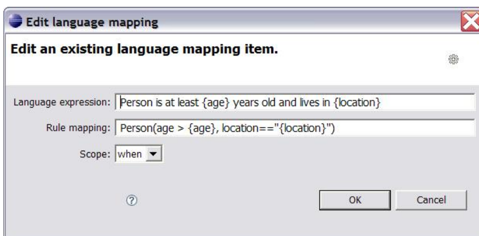
Figure 6.9. Language Mapping editor dialog
