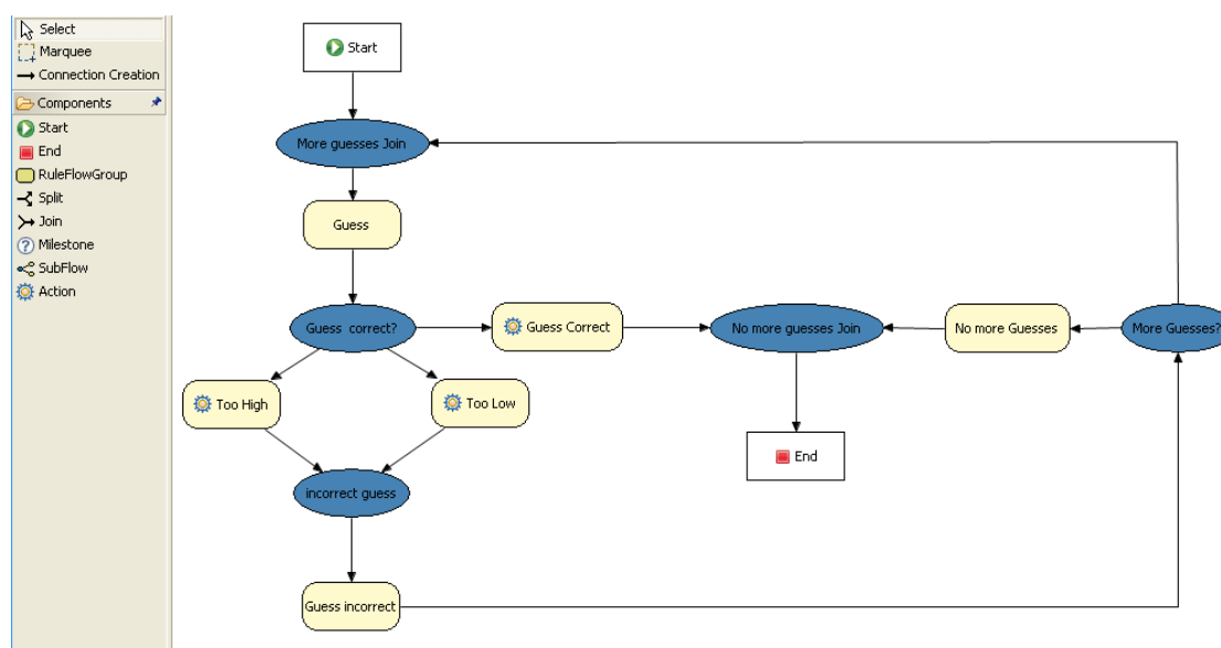
Figure 7.18. RuleFlow for the NumberGuess Example
