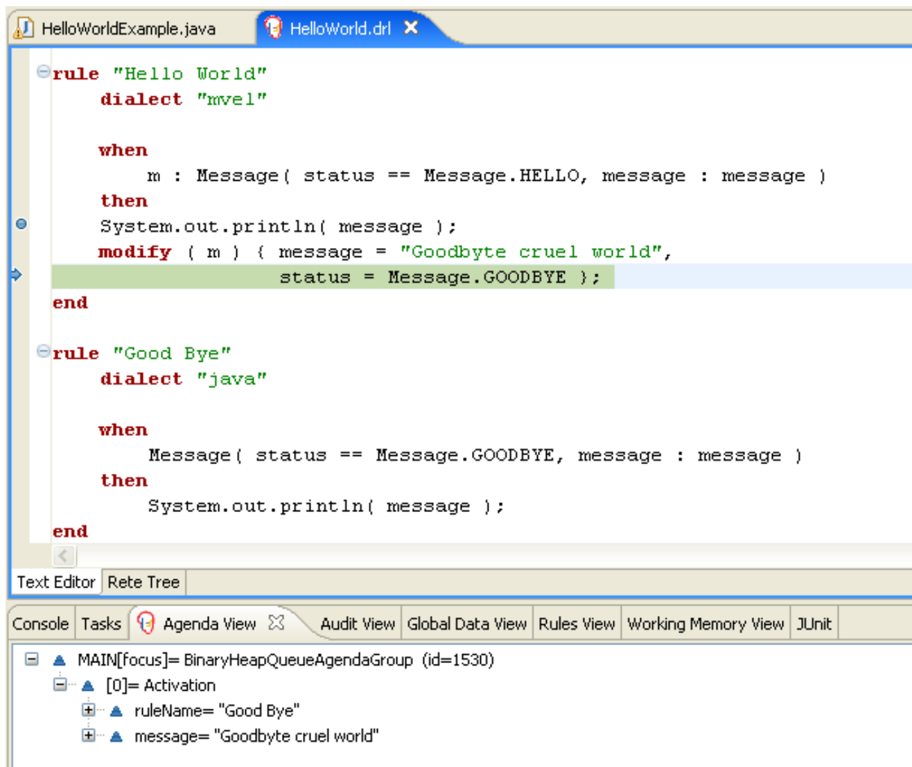
Figure 7.2. Hello World: rule "Hello World" Agenda View
