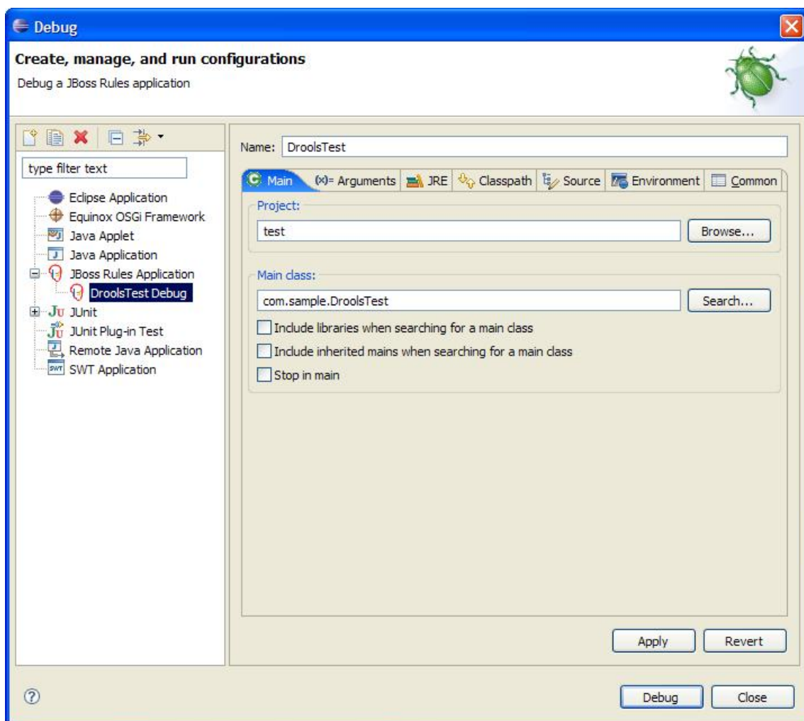
Figure 6.12. Debug as Drools Application Configuration
