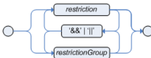
Figure 4.13. Abbreviated combined relation condition
