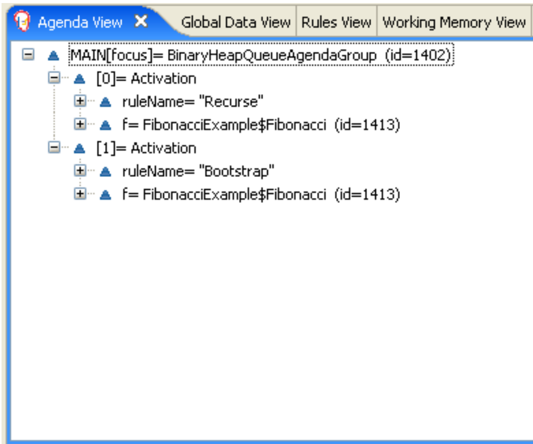
Figure 7.7. Fibonacci Example: "Recurse" Agenda View 1
