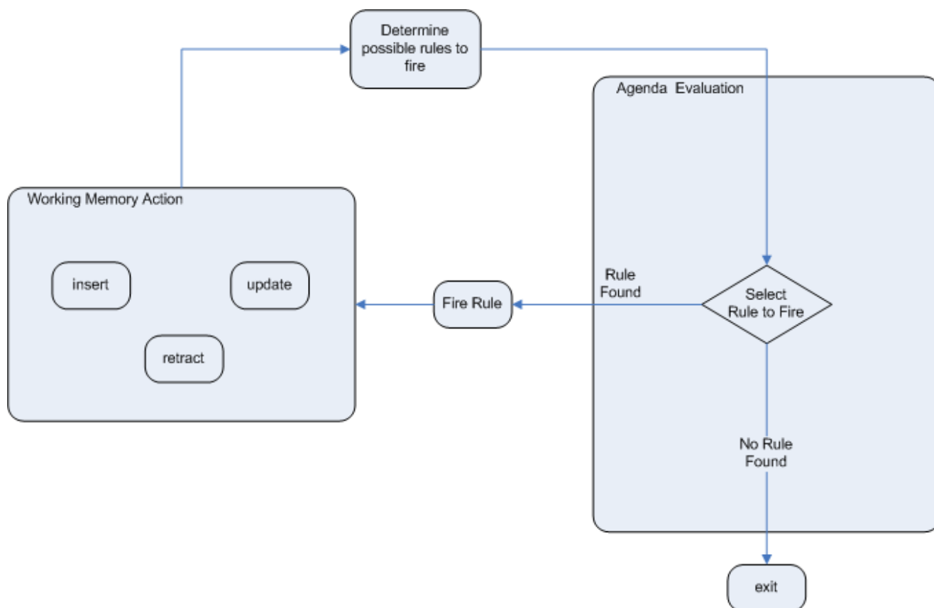
Figure 3.17. Two Phase Execution
