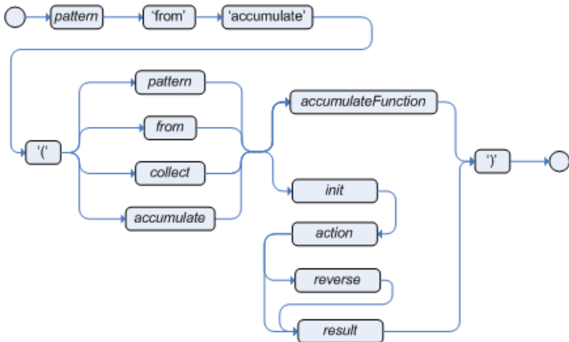
Figure 4.27. accumulate
