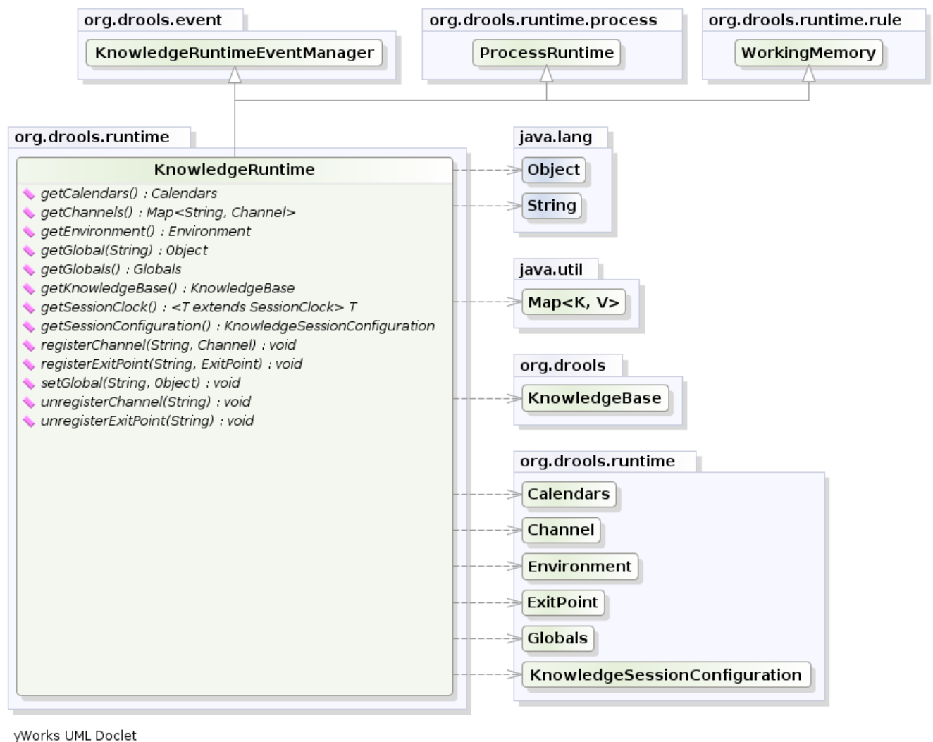
Figure 3.14. KnowledgeRuntime
