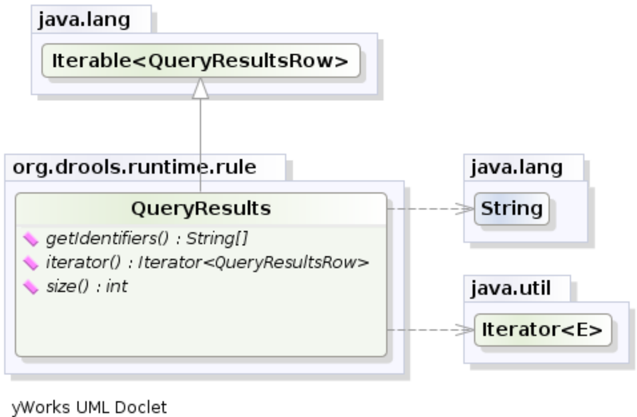
Figure 3.12. QueryResults
