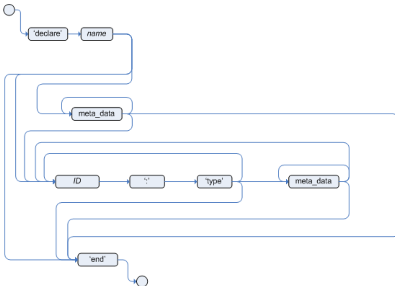
Figure 4.8. type_declaration
