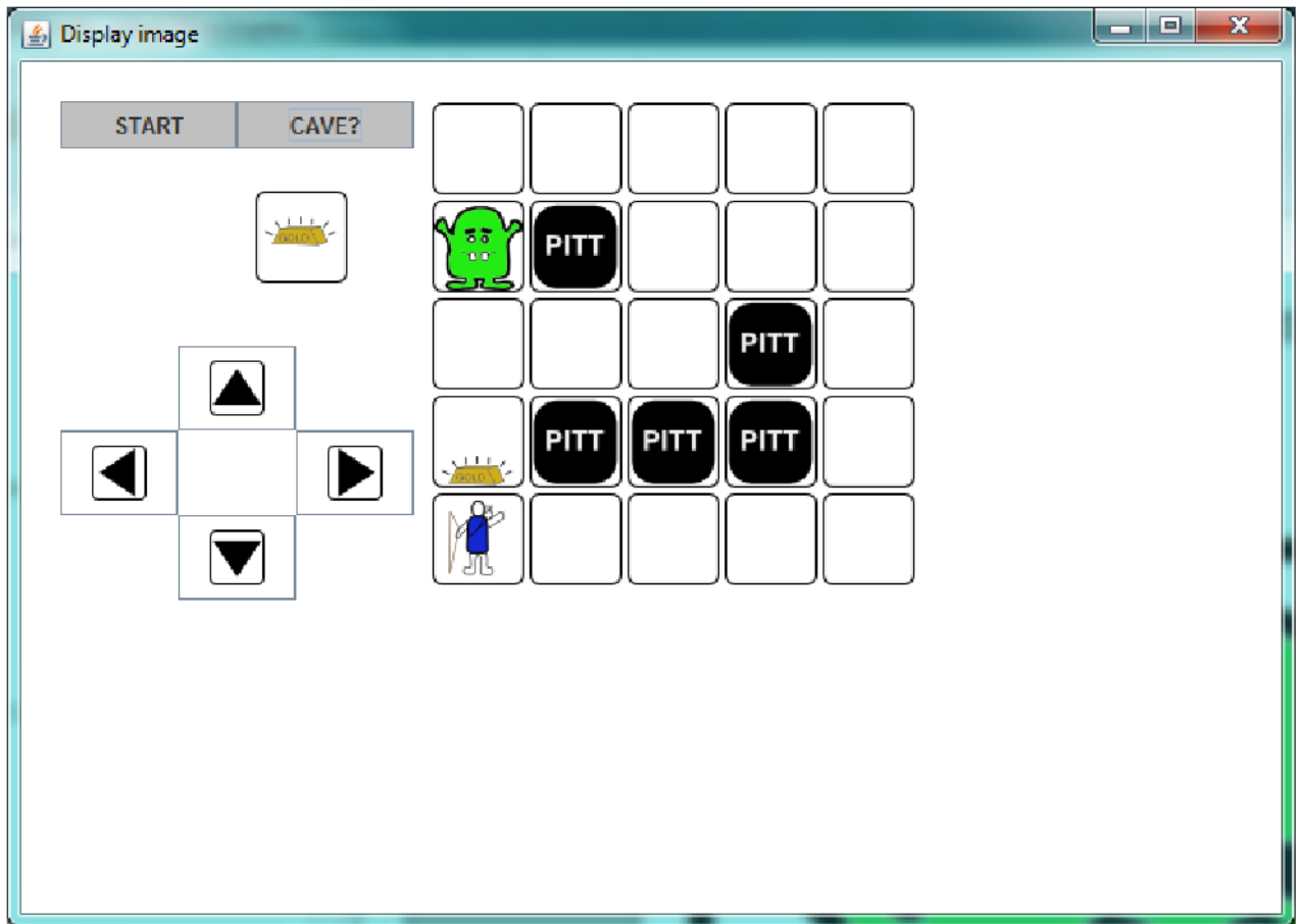
Figure 7.28. Cave Screenshot
