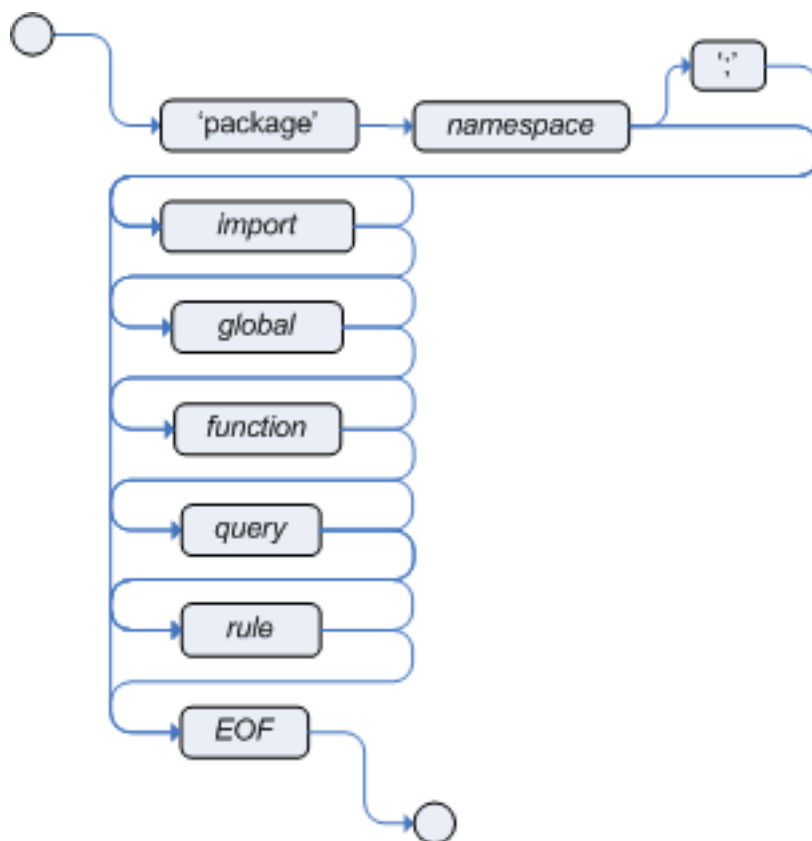
Figure 4.3. package
