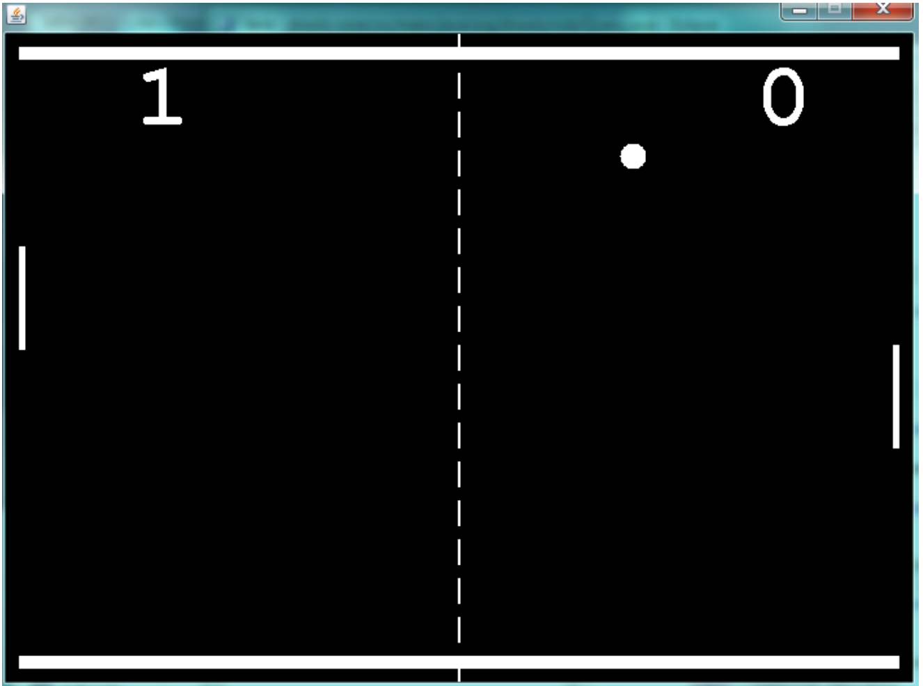
Figure 7.25. Pong Screenshot
