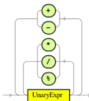
AdditiveExpr
