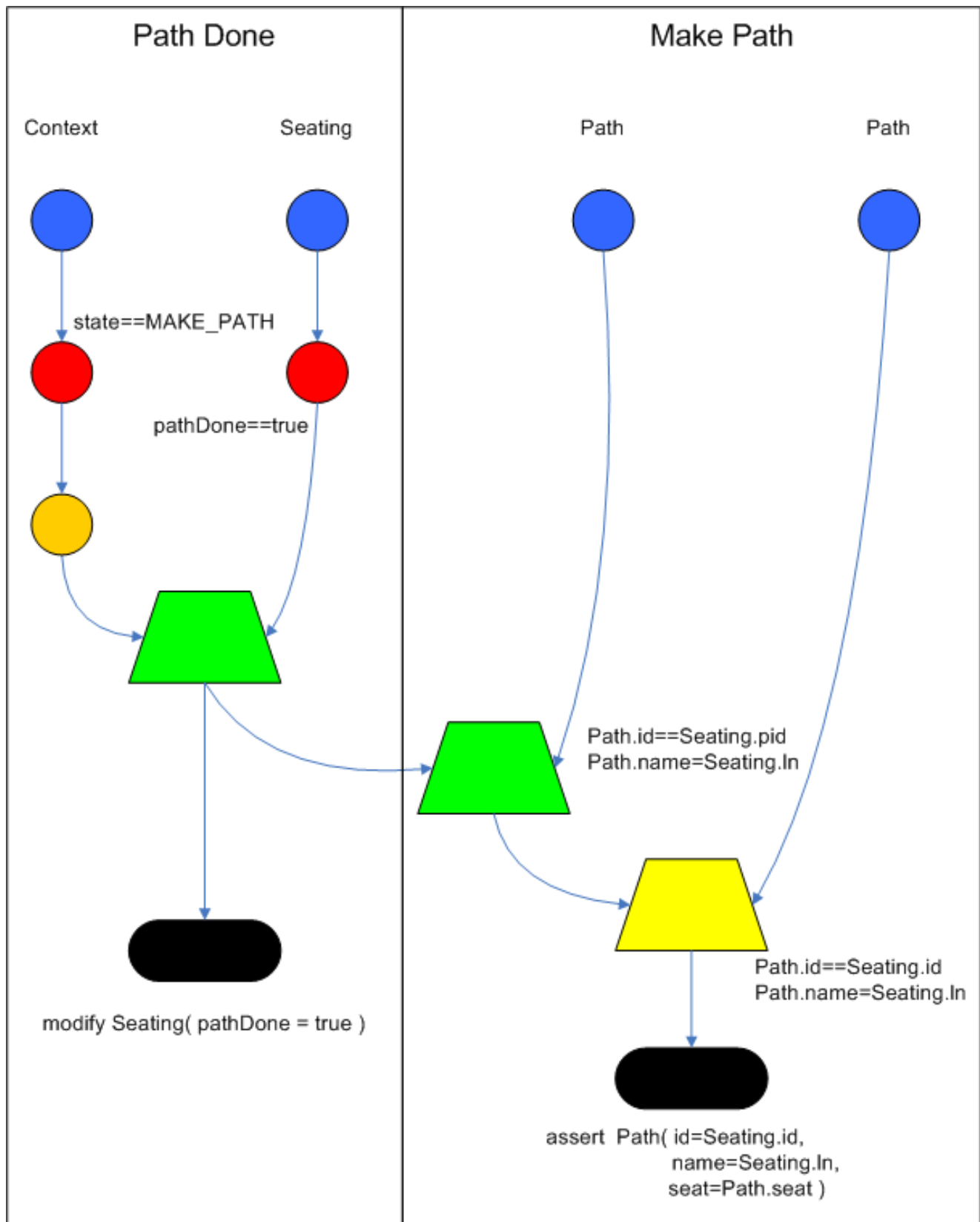
Figure 7.34. Rete Diagram
