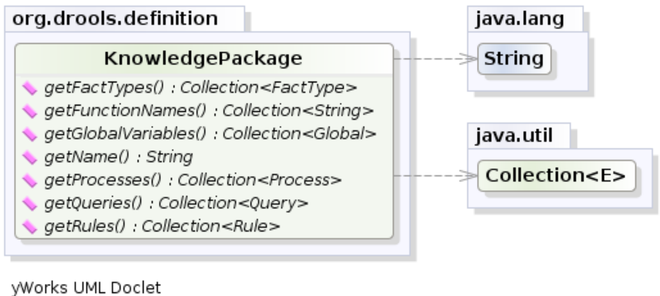
Figure 3.4. KnowledgePackage
