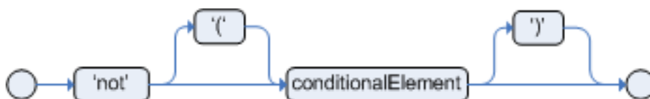
Figure 4.22. not
