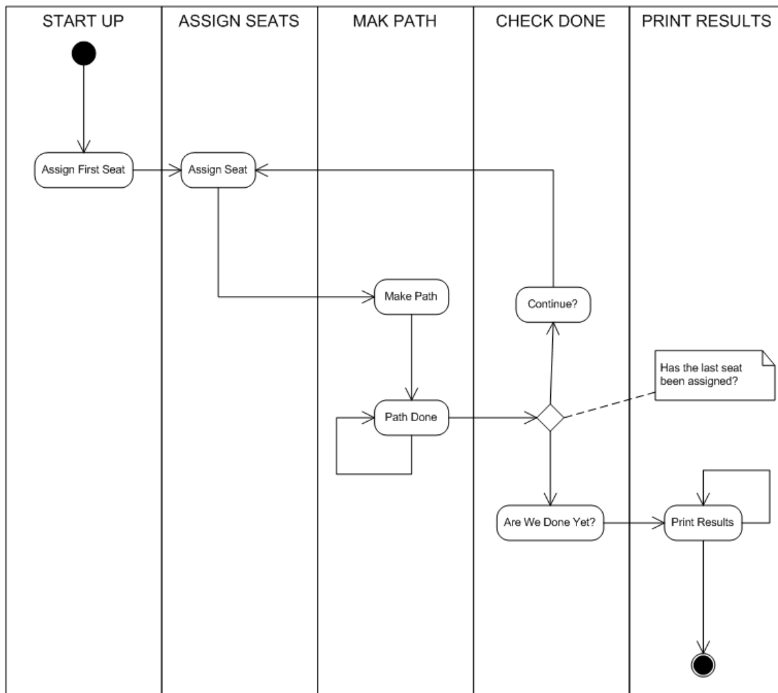
Figure 7.33. Manners Activity Diagram
