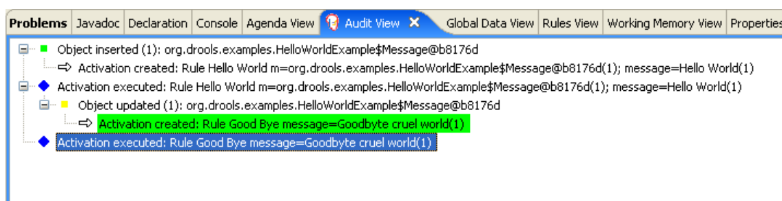
Figure 7.3. Hello World: Audit View
