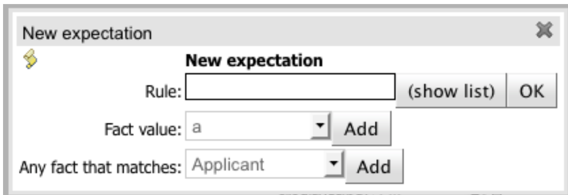
Figure 4.85. Expect popup
