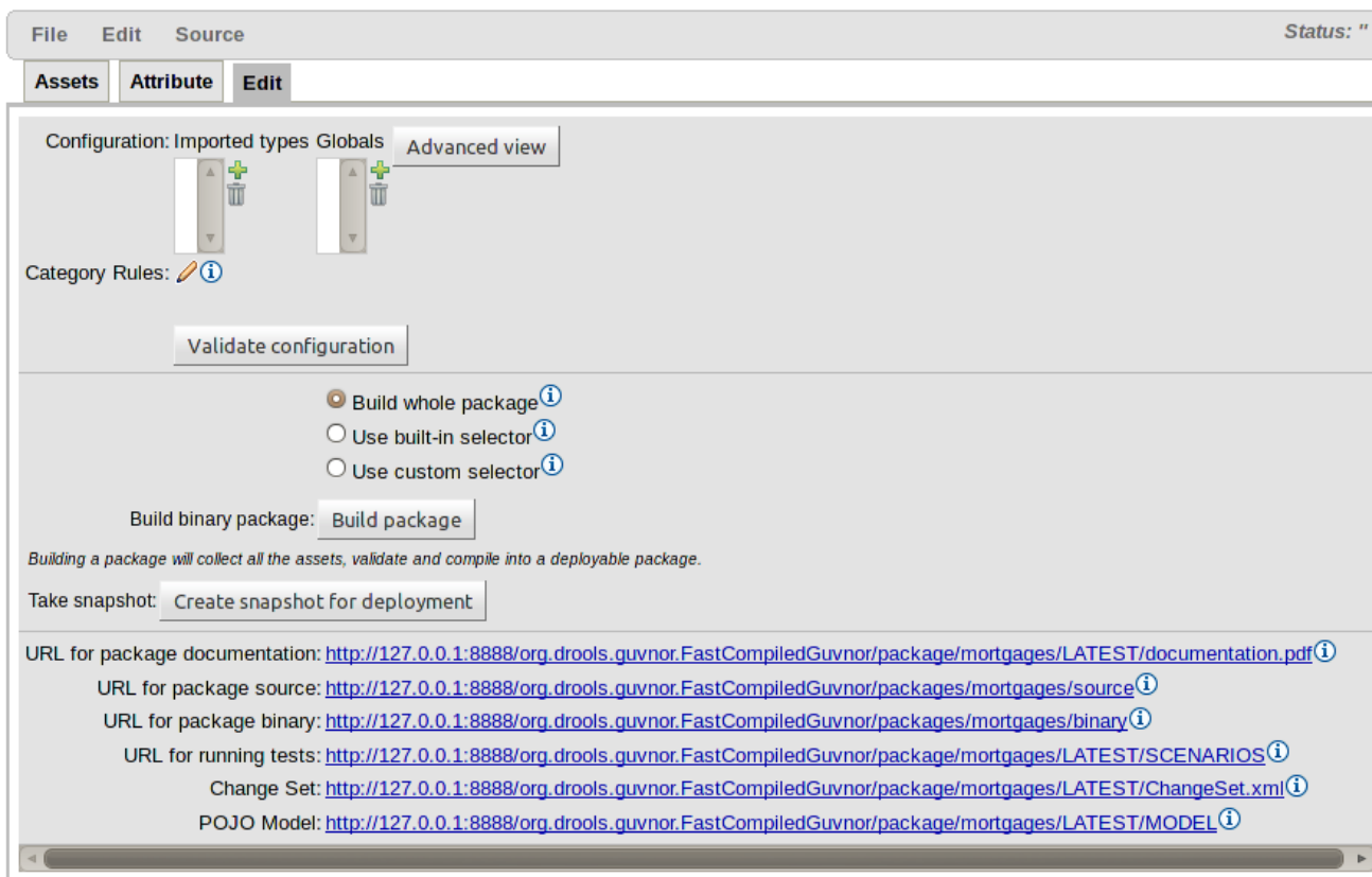
Figure 5.6. Package configuration
