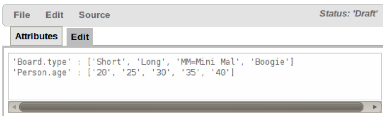
Figure 4.81. Data enumeration
