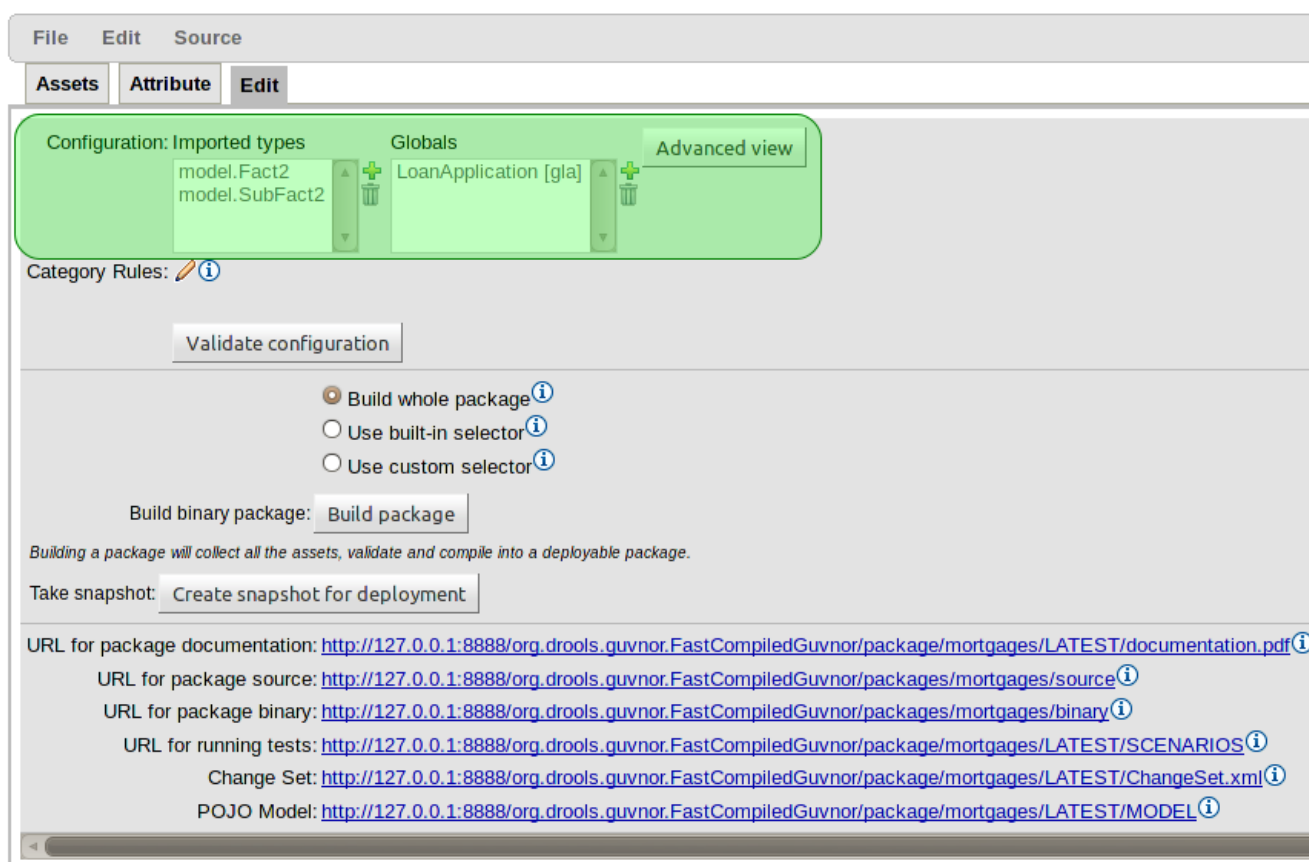
Figure 7.4. Imports and Globals configuration
