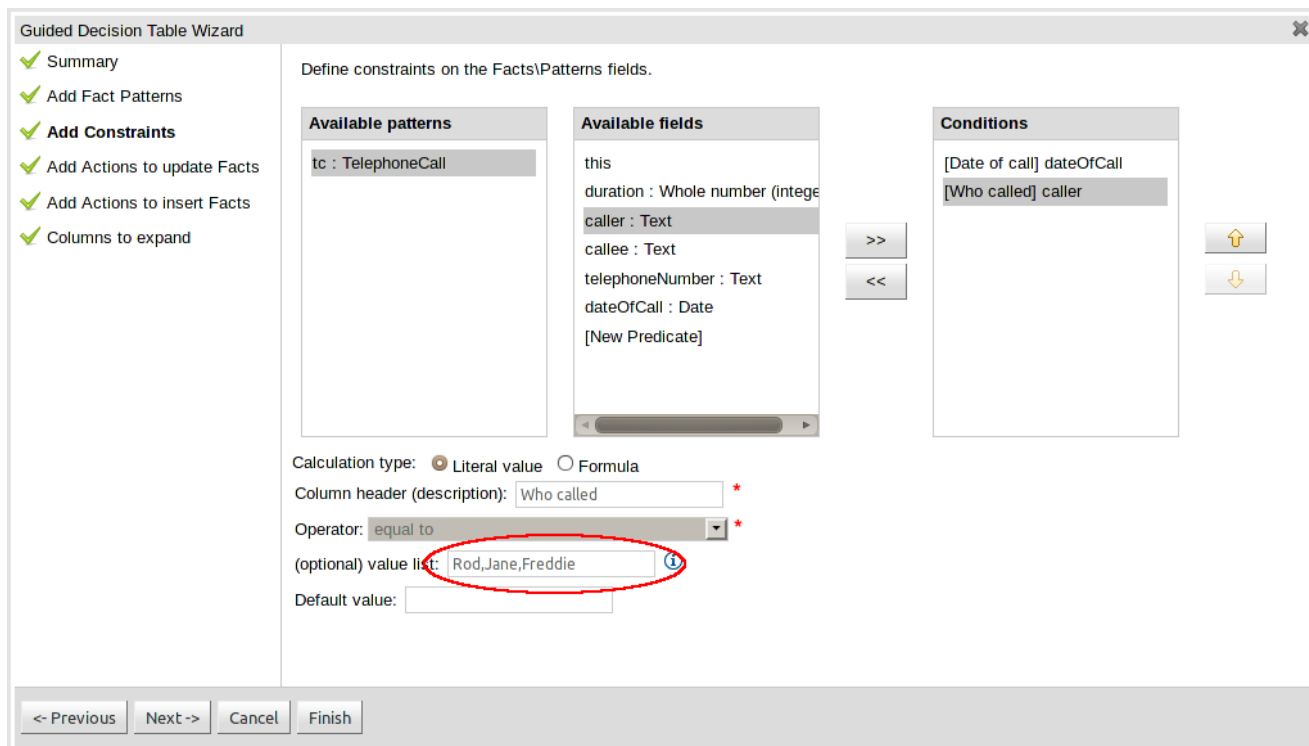
Figure 4.54. Example of a Condition column with optional values defined
