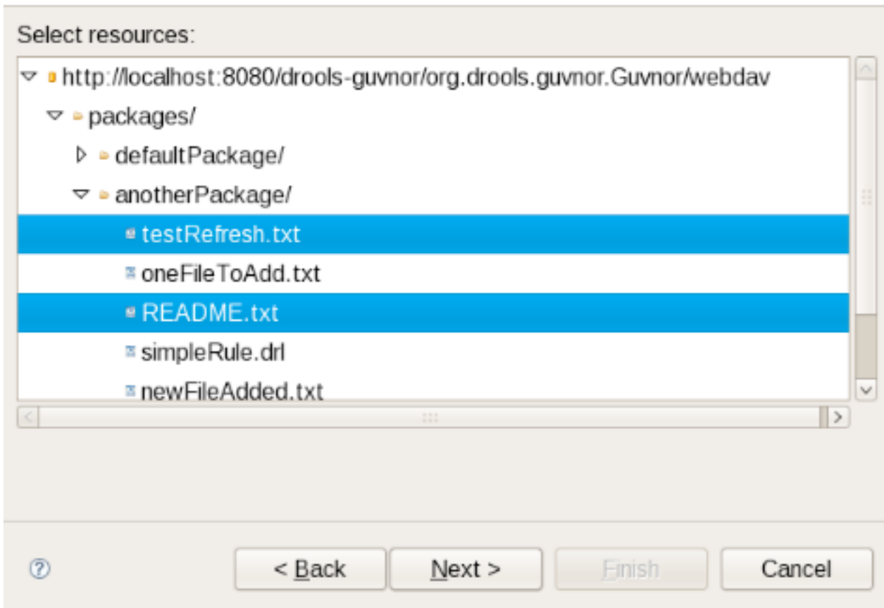
Figure 9.25. Import
