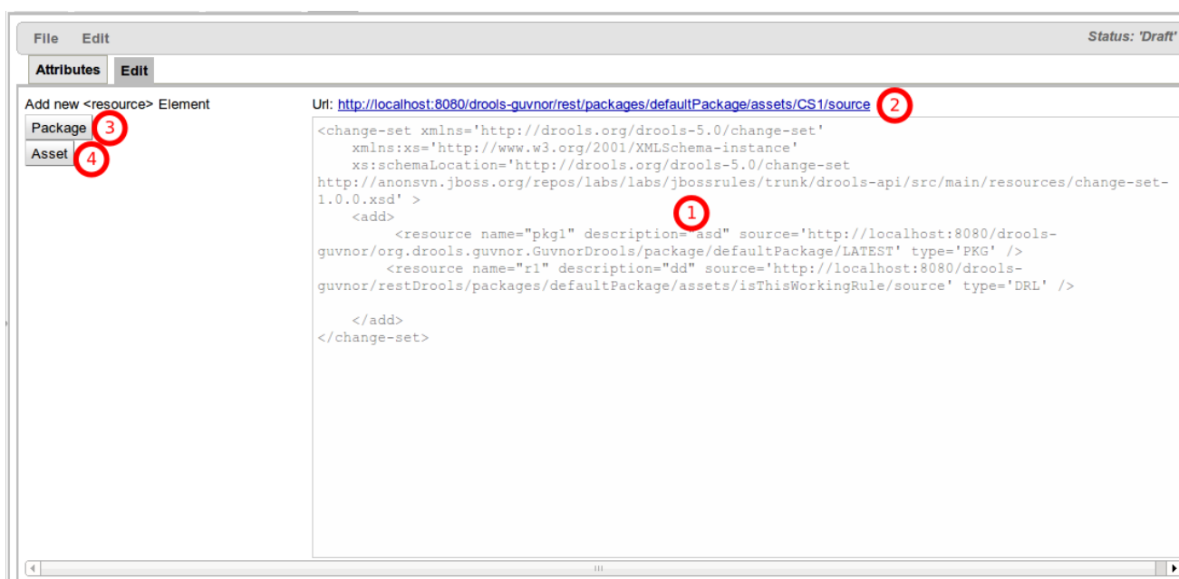
Figure 4.93. Change-Set Editor
