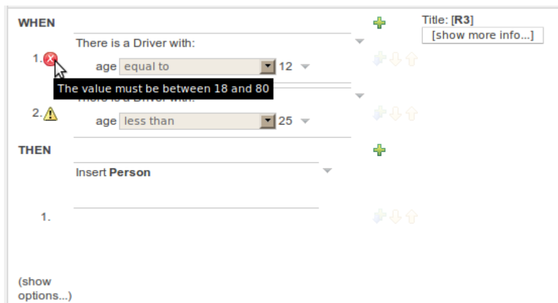
Figure 4.19. Real-Time Field Constraints validation
