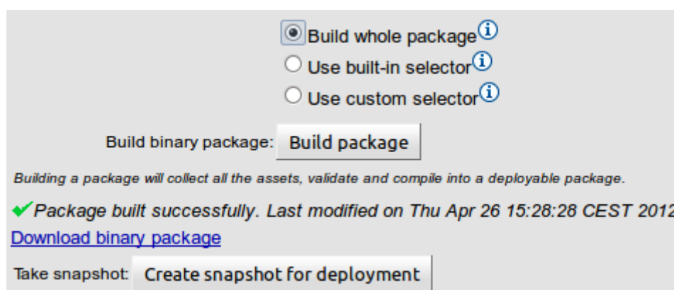
Figure 7.11. Package building
