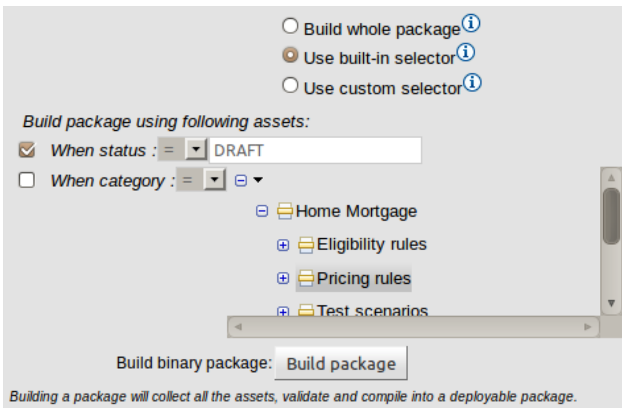
Figure 7.12. Built-in Selector
