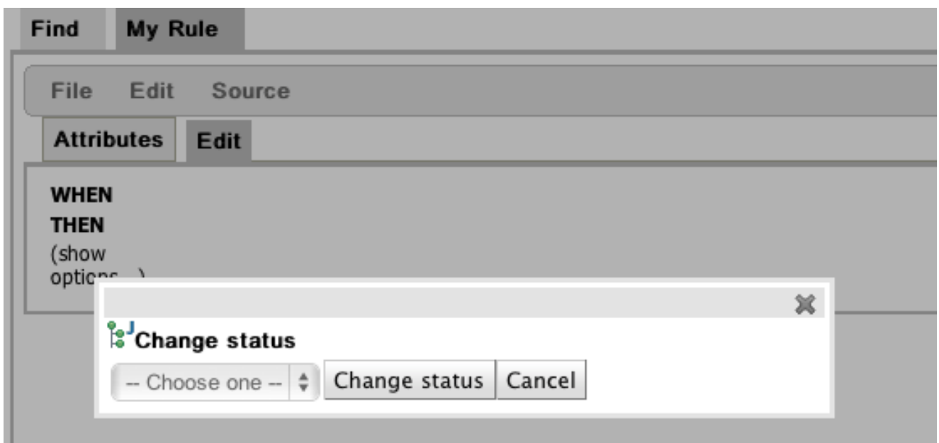
Figure 8.4. Asset status
