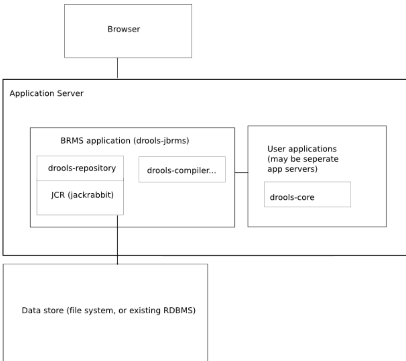
Figure 17.1. Architectural diagram
