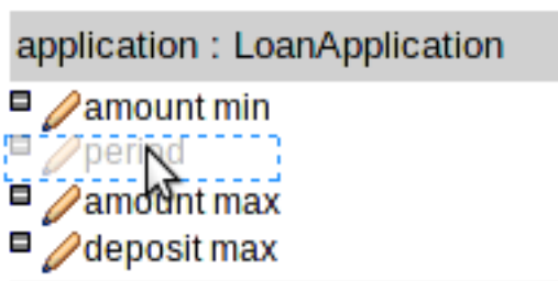
Figure 4.35. Re-arranging columns
