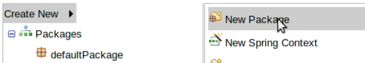
Figure 4.8. New Package
