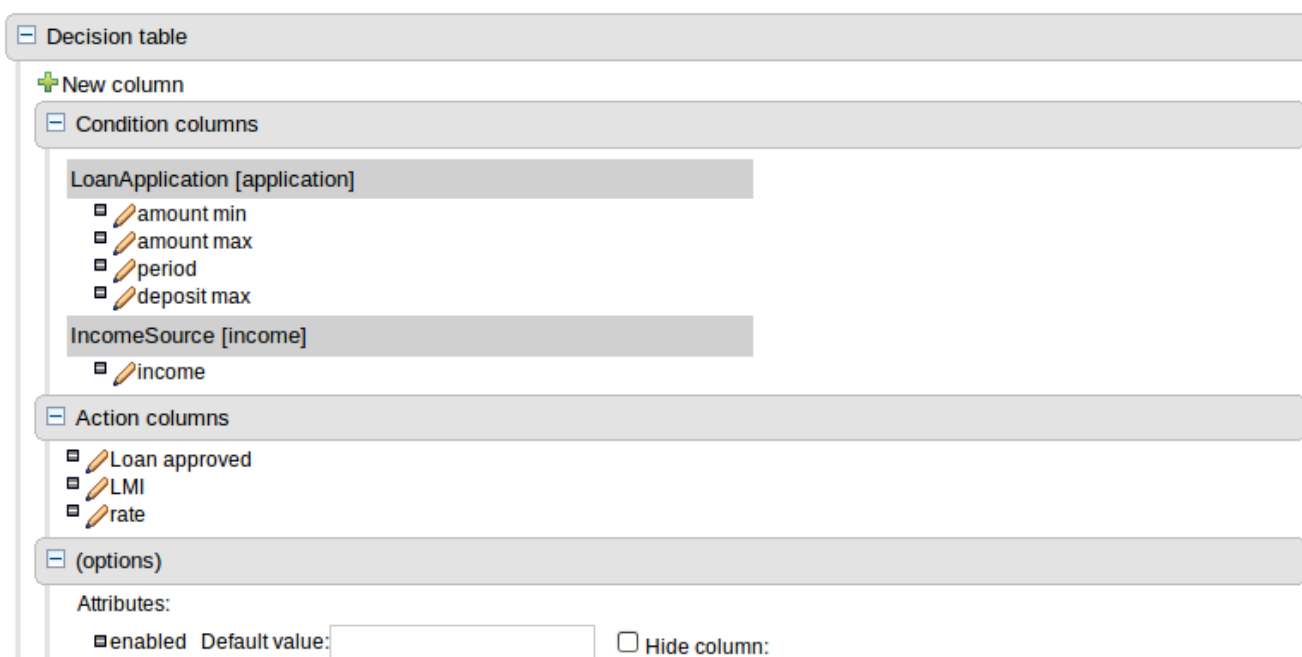
Figure 4.36. Column configuration
