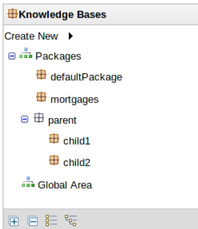
Figure 5.1. Hierarchical view
