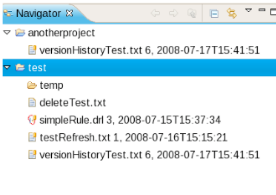
Figure 9.15. Navigator
