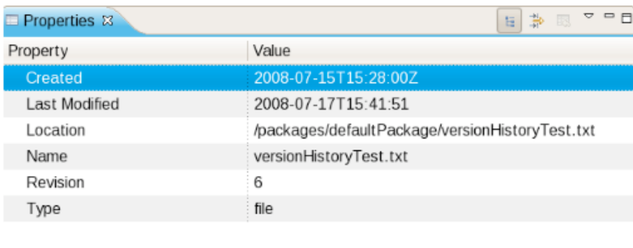
Figure 9.13. Properties
