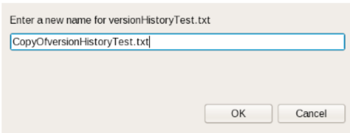
Figure 9.27. Copy
