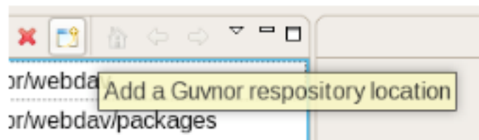
Figure 9.8. Connection wizard
