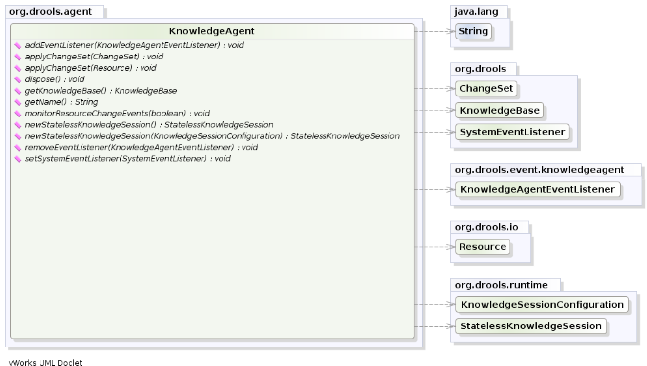
Figure 3.7. KnowledgeAgent
