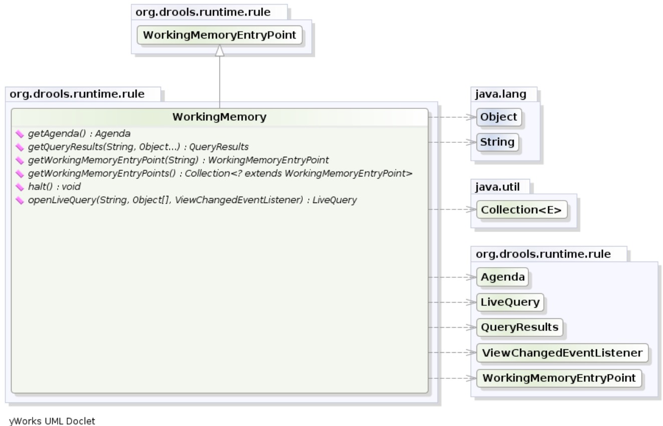
Figure 3.11. WorkingMemory
