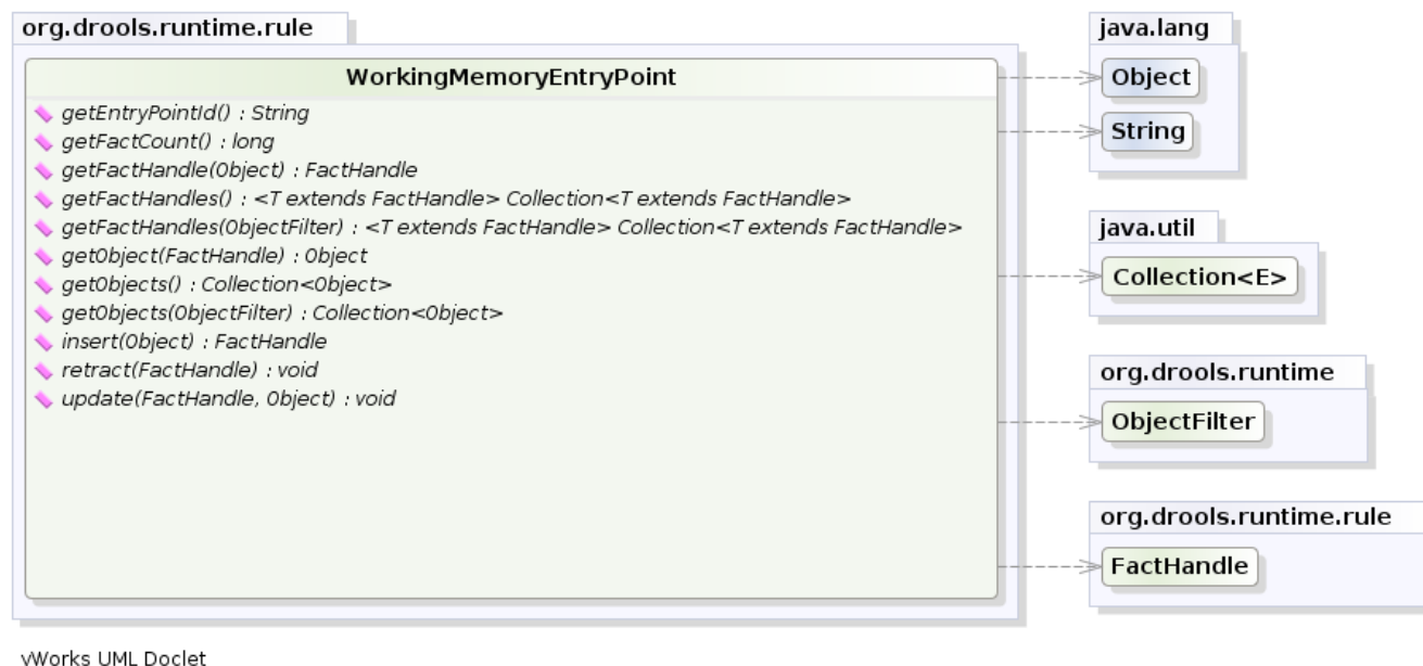
Figure 3.10. WorkingMemoryEntryPoint
