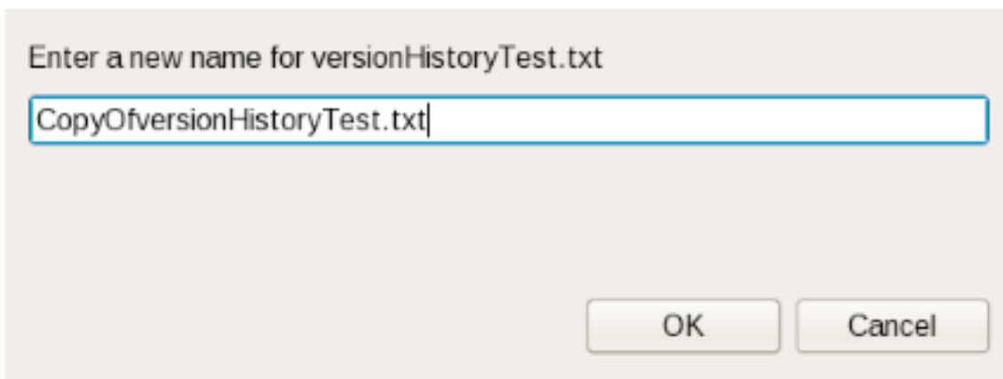
Figure 9.27. Copy
