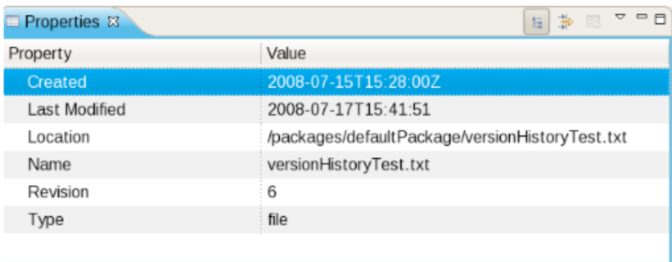
Figure 9.13. Properties
