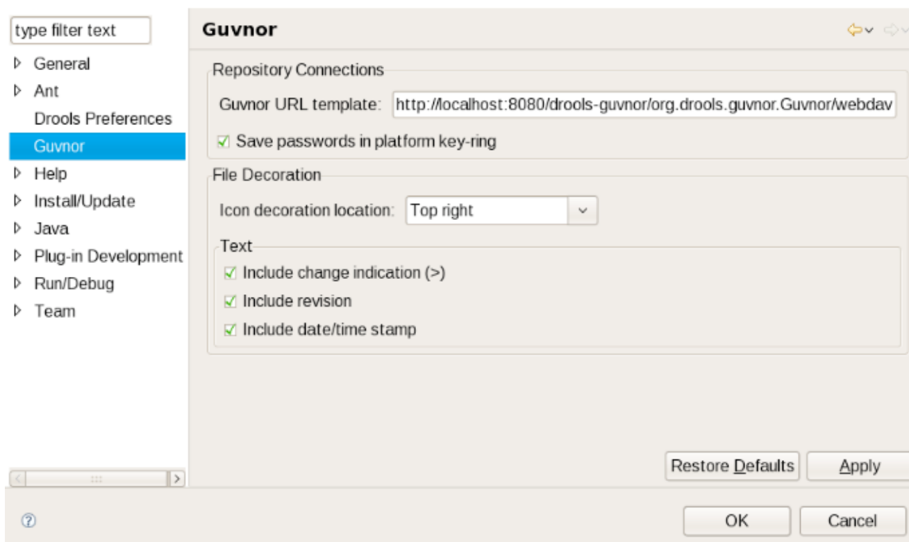
Figure 9.28. Preferences
