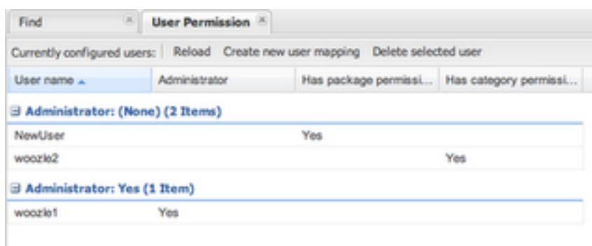
Figure 15.2. User listing
