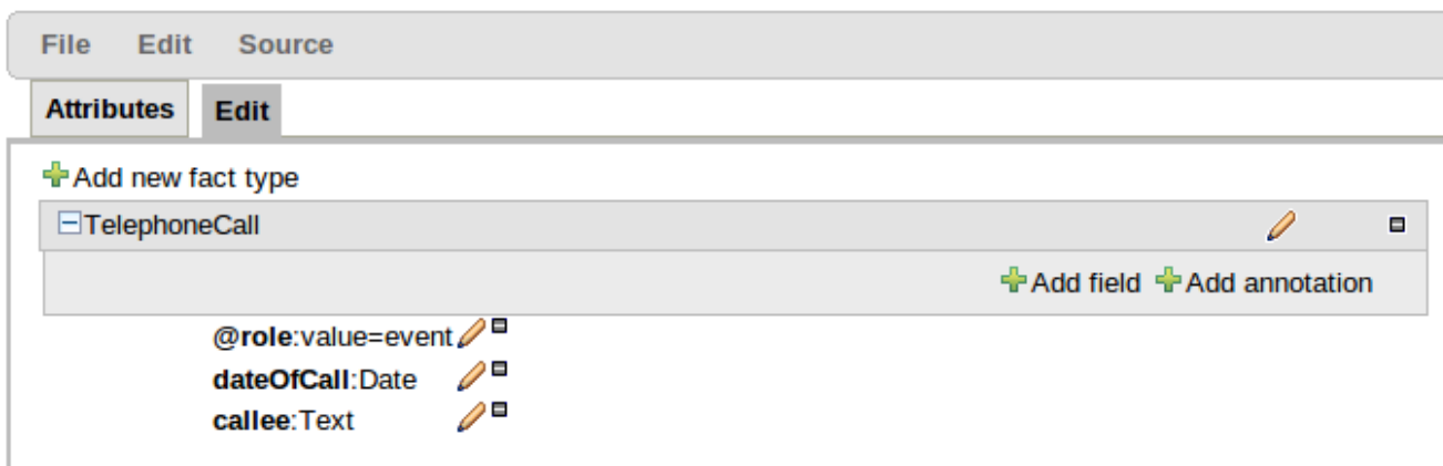
Figure 4.64. Annotations
