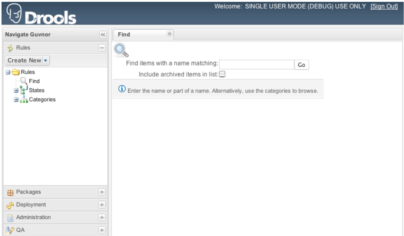
Figure 4.99. New Look
