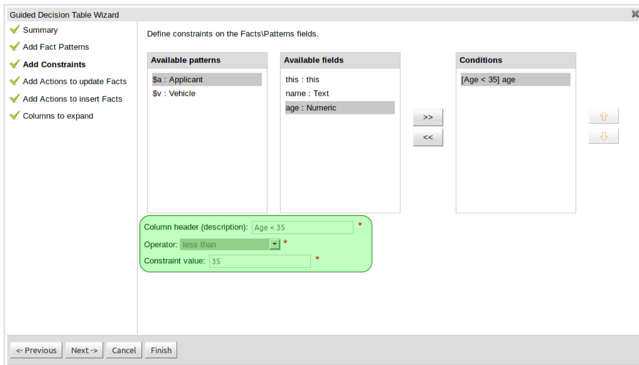
Figure 4.15. Defining Limited Entry constraints with the Wizard
