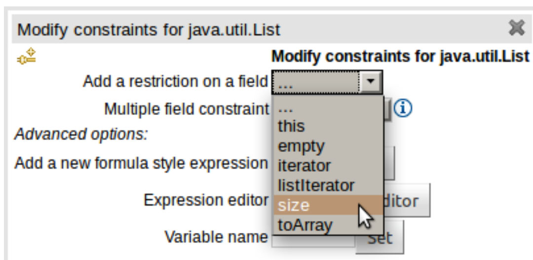
Figure 4.2. Additional members
