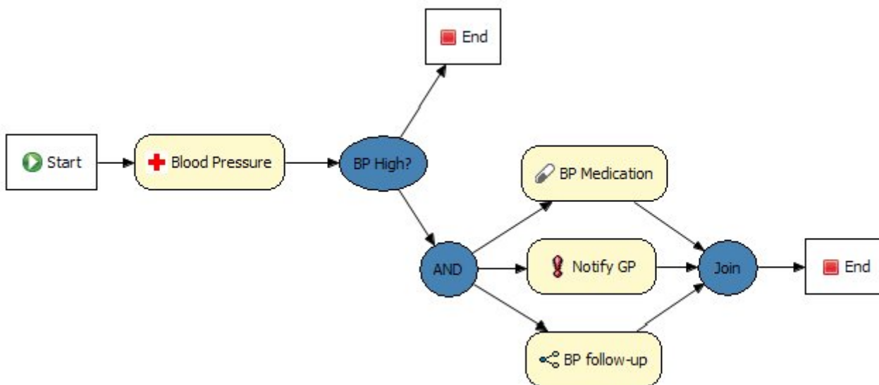
Figure 4.108. Work items
