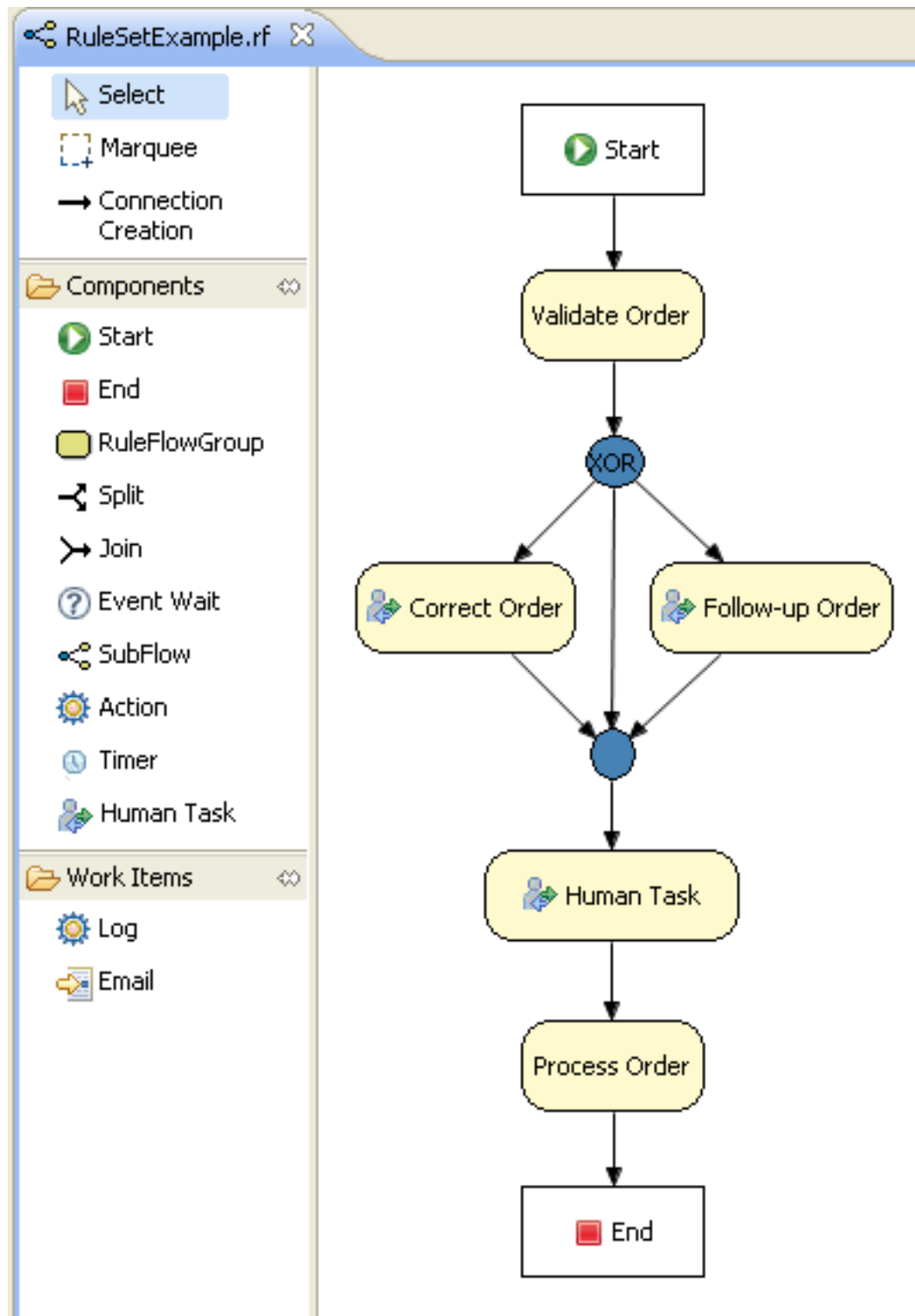
Figure 4.107. Human task
