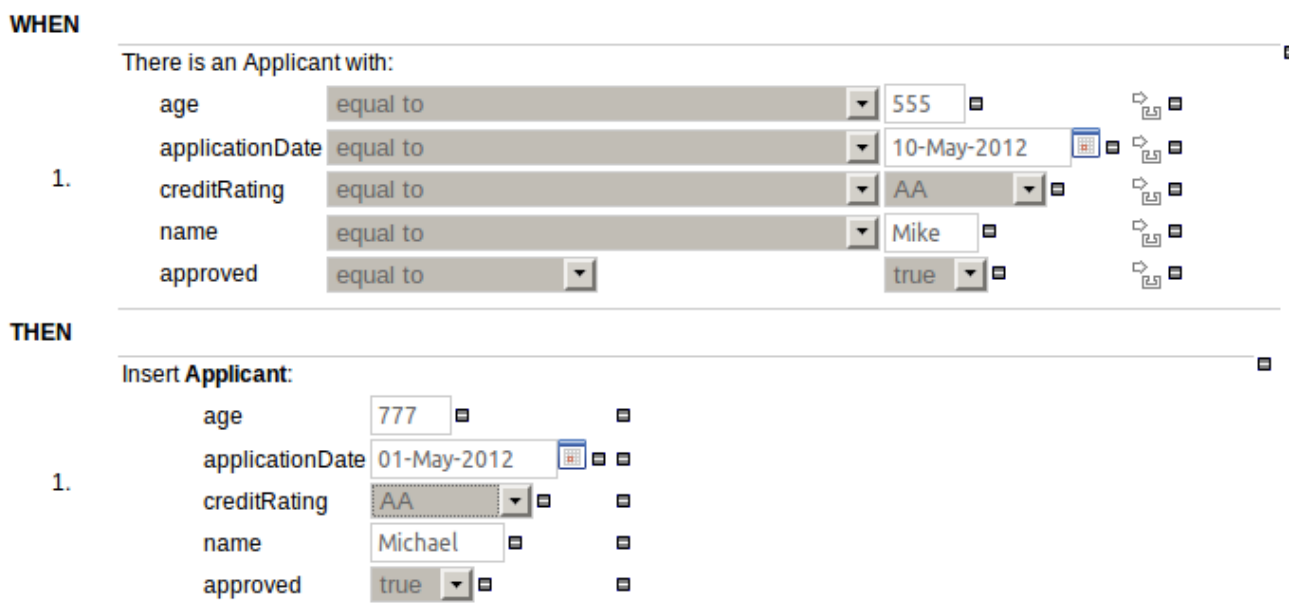
Figure 4.1. Improved consistency
