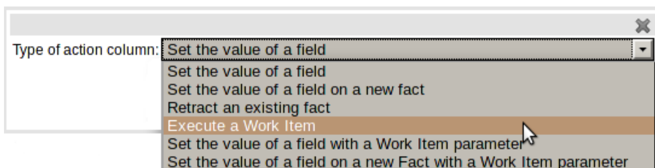
Figure 4.27. New Actions
