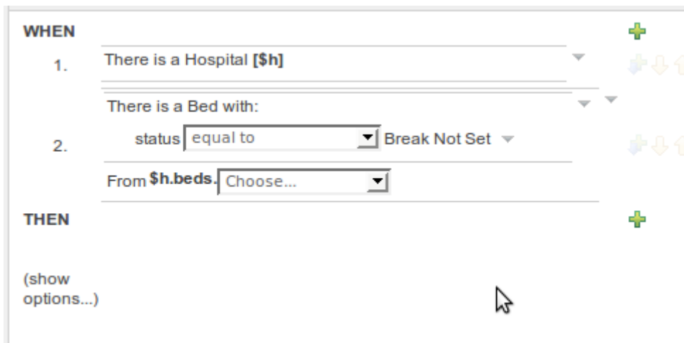
Figure 4.78. From CE Builder
