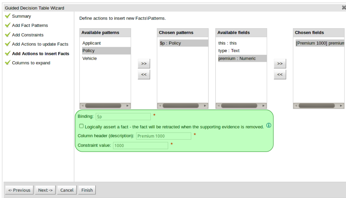
Figure 4.16. Defining Limited Entry actions with the Wizard
