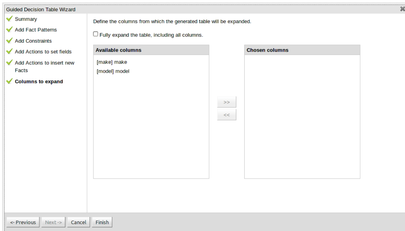
Figure 4.60. Choose how rows are created - select the columns you want to expand upon
