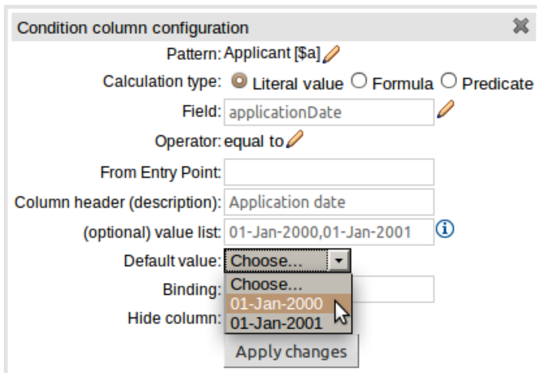
Figure 4.44. Setting the default value of a cell with a Value List
