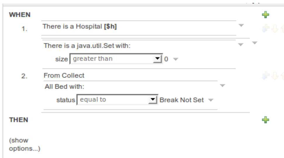
Figure 4.79. From Collect CE Builder
