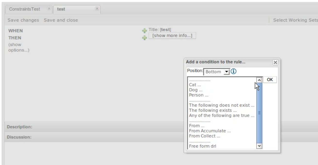
Figure 4.89. The available types are reduced
