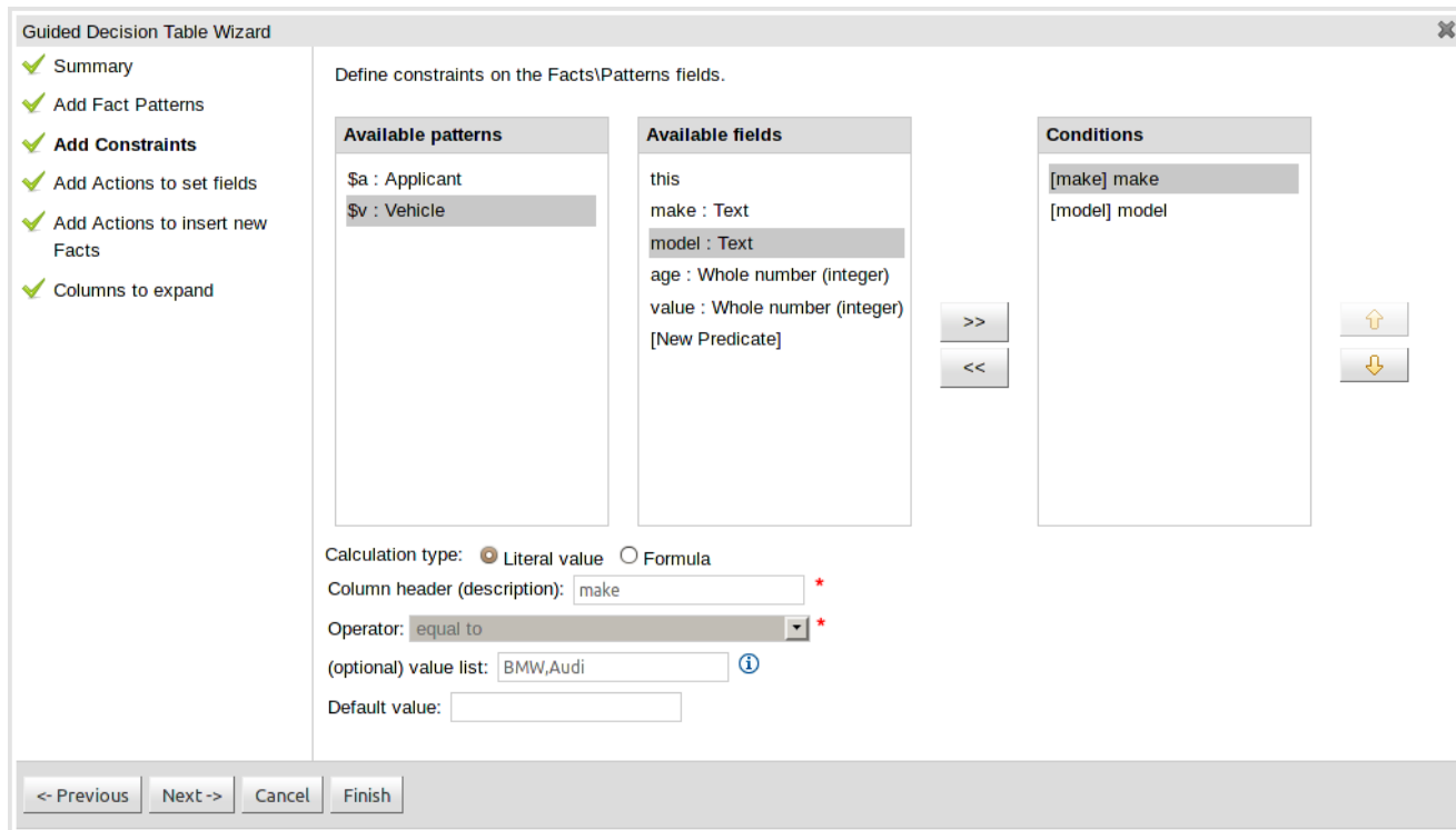
Figure 4.56. Add constraints to facts
