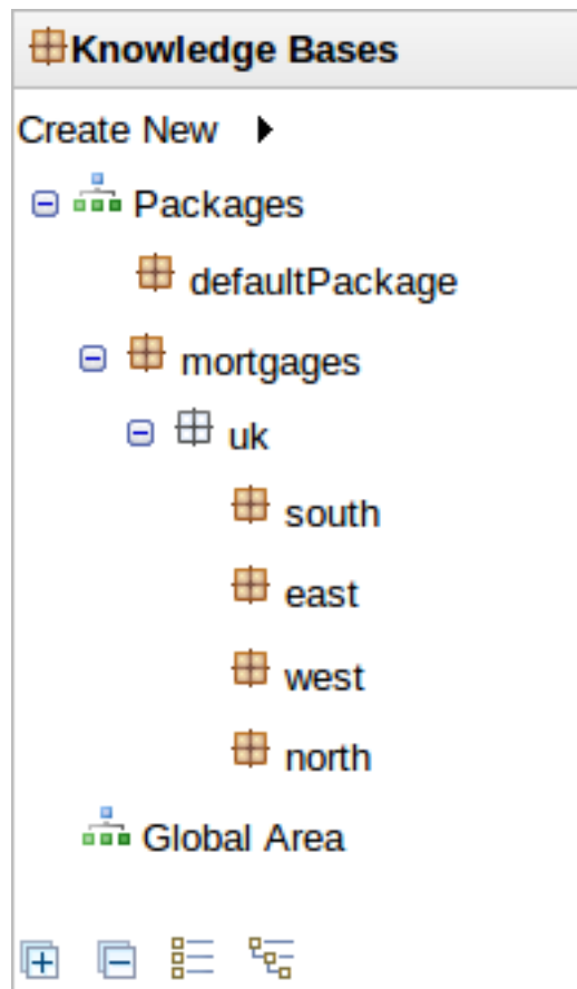
Figure 4.48. Hierarchical view
