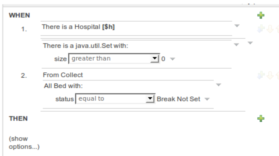
Figure 4.79. From Collect CE Builder
