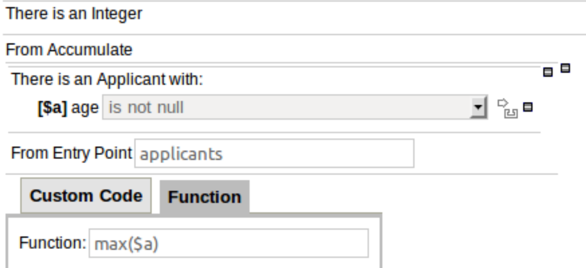
Figure 4.6. Accumulate with entry-point
