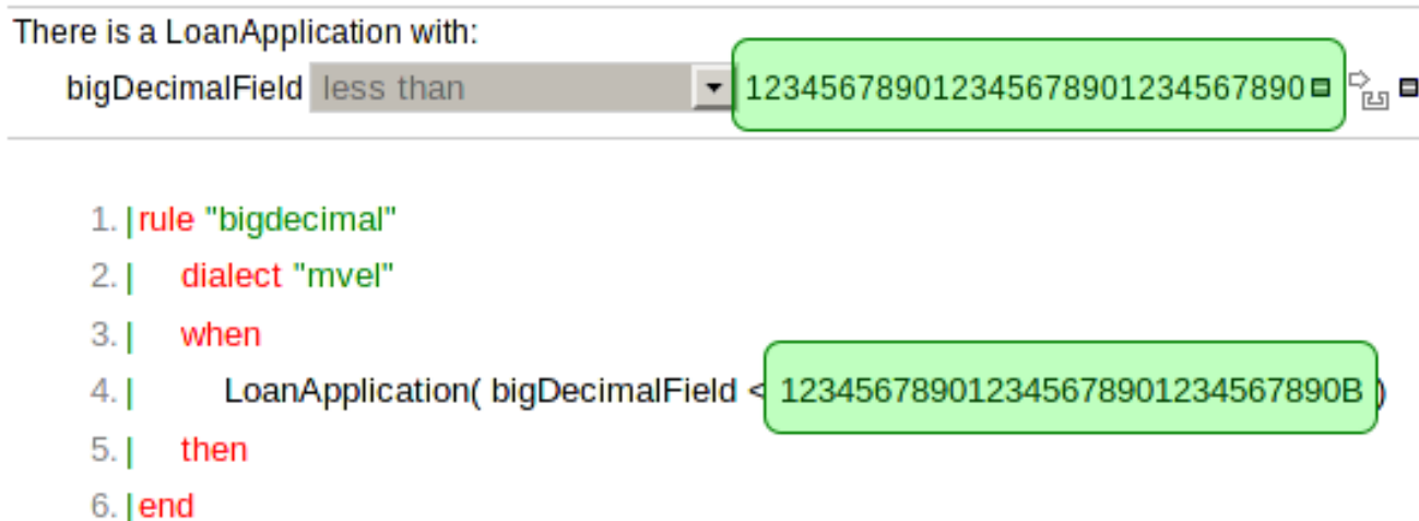
Figure 4.41. Example of using a BigDecimal
