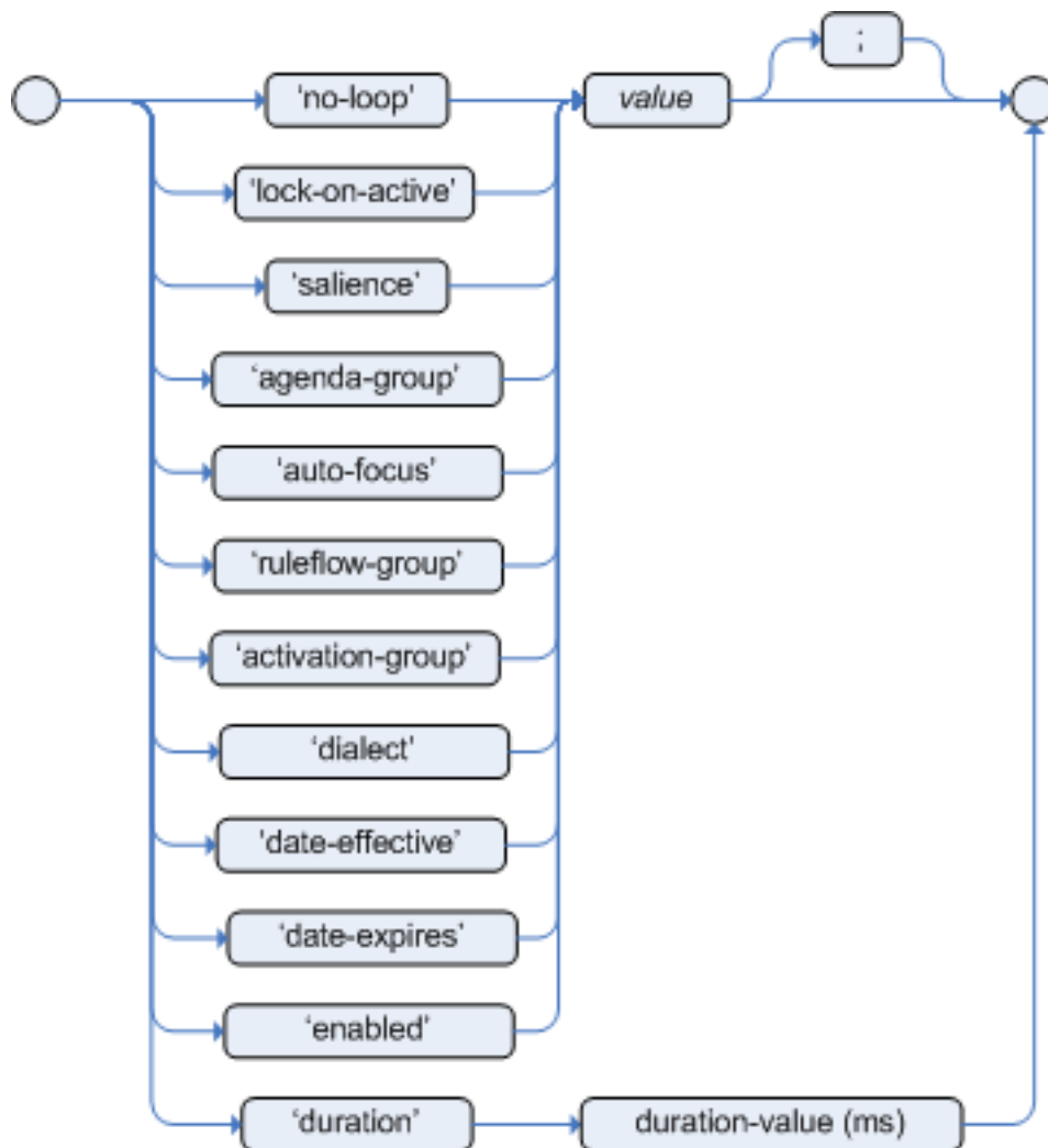
Figure 4.10. rule attributes
