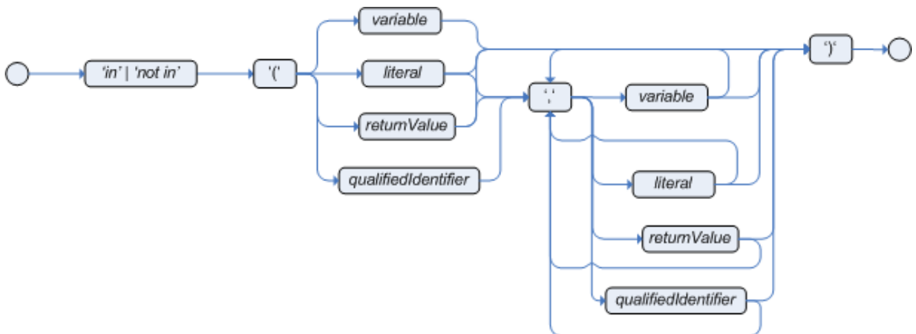
Figure 4.16. compoundValueRestriction
