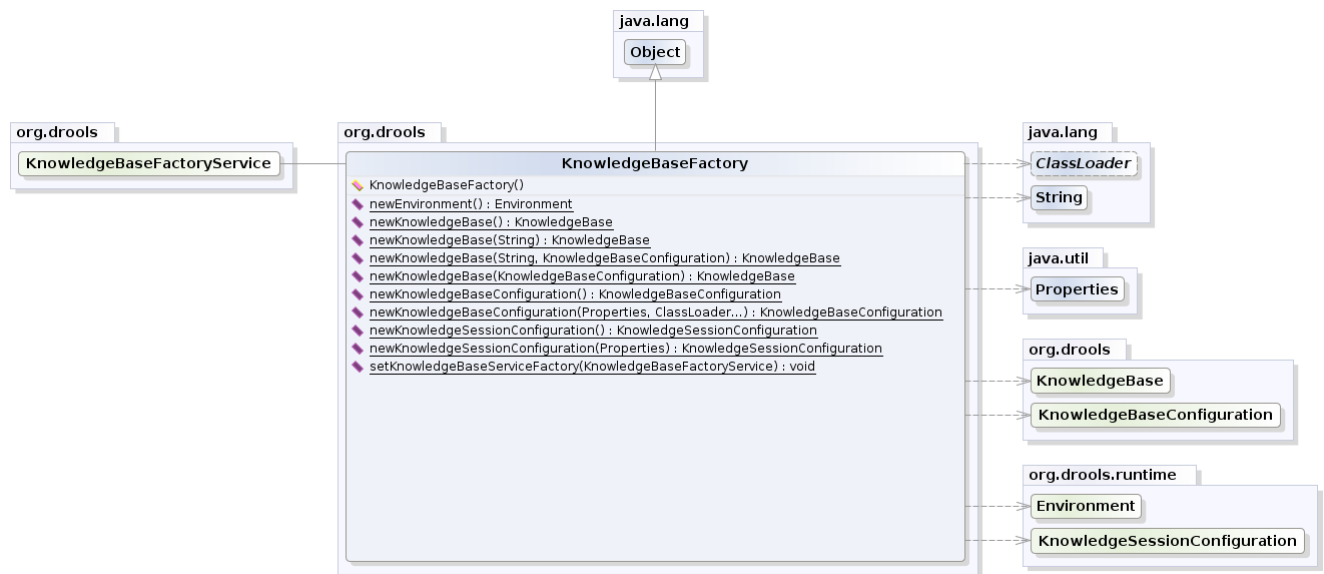
Figure 3.6. KnowledgeBaseFactory
