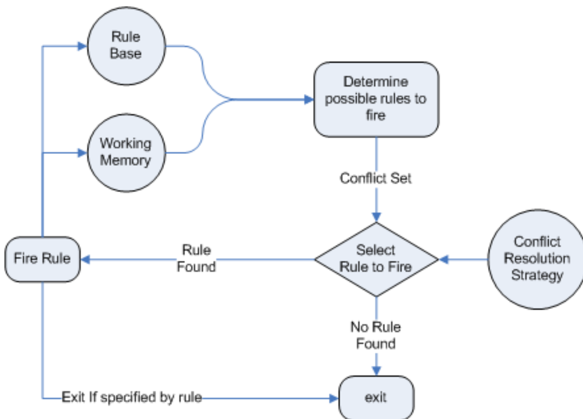
Figure 1.2. Forward Chaining
