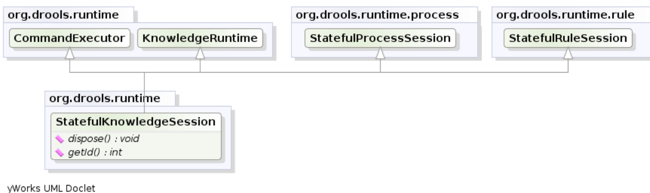
Figure 3.9. StatefulKnowledgeSession
