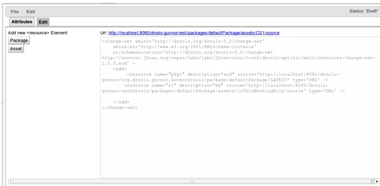
Figure 4.65. Change-Set Editor
