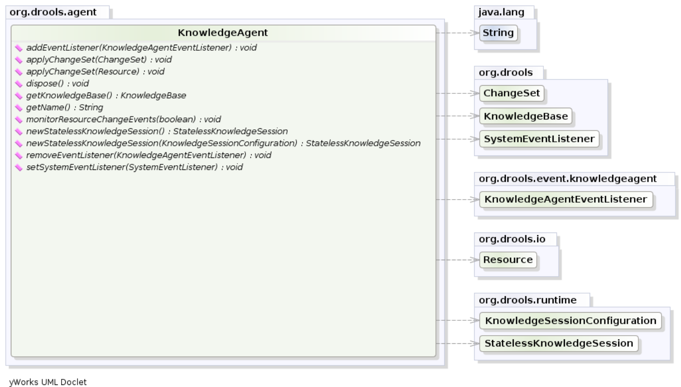
Figure 3.7. KnowledgeAgent
