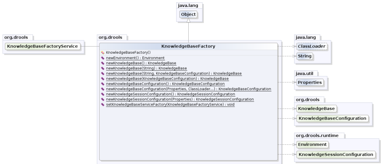
Figure 3.6. KnowledgeBaseFactory
