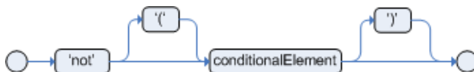
Figure 4.22. not
