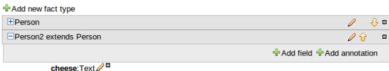
Figure 4.78. Declarative model showing extensions
