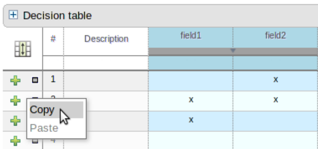
Figure 4.65. Copying a row
