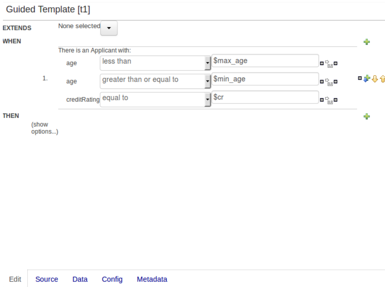
Figure 16.11. Rule template in the guided editor
