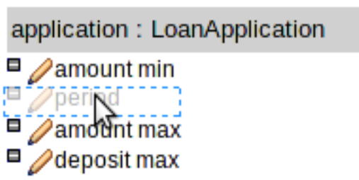
Figure 16.22. Re-arranging columns
