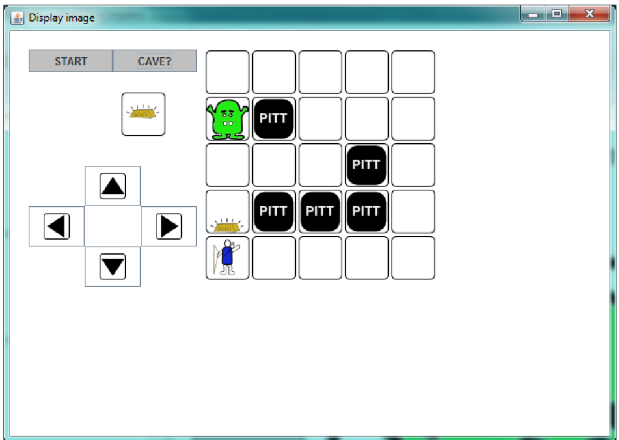
Figure 19.33. Cave Screenshot
