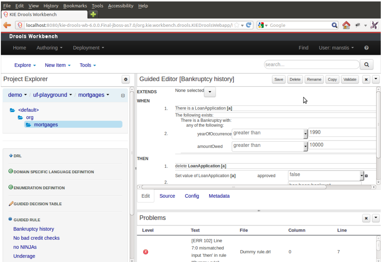
Figure 2.2. Workbench
