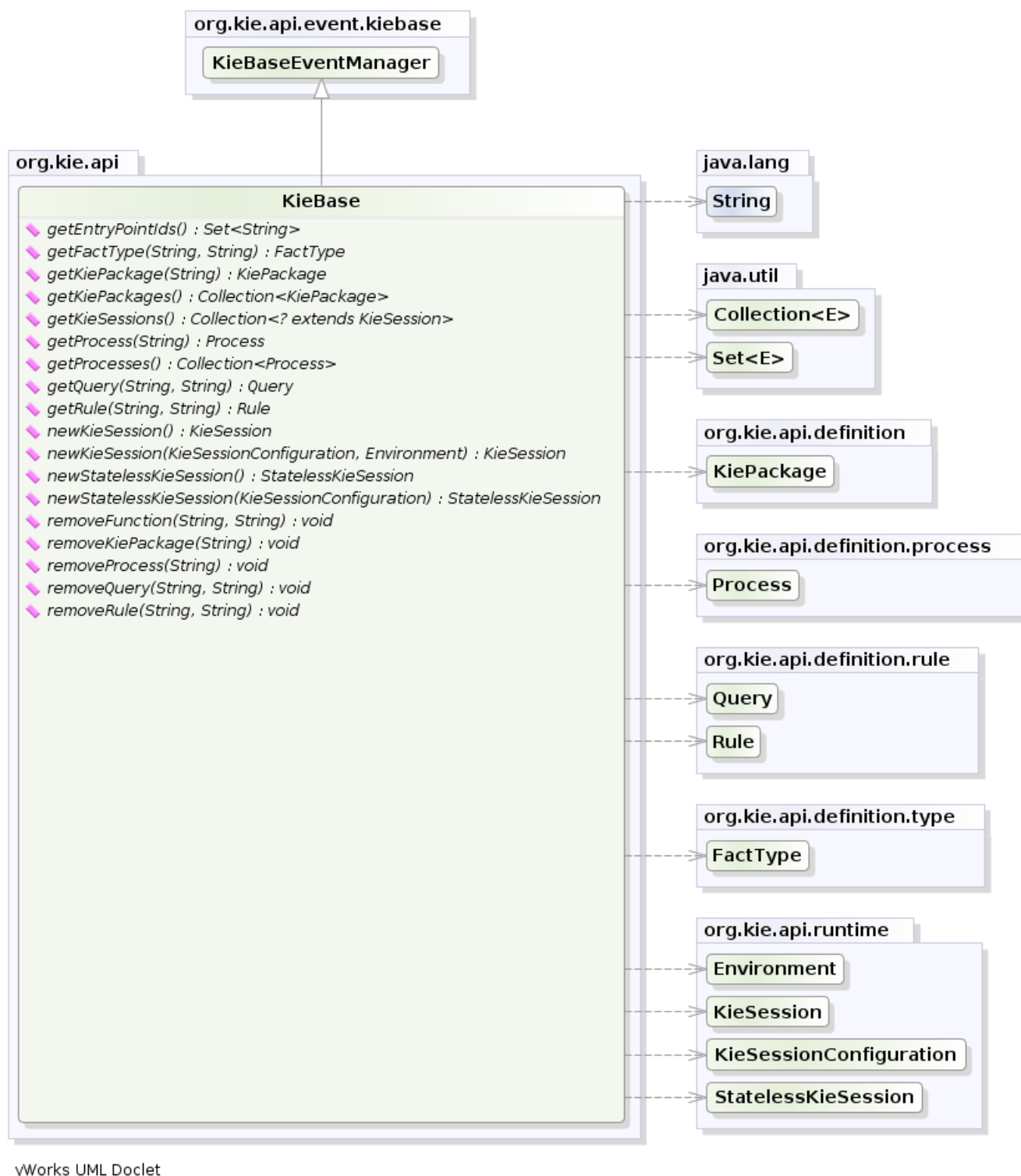
Figure 4.7. KieBase
