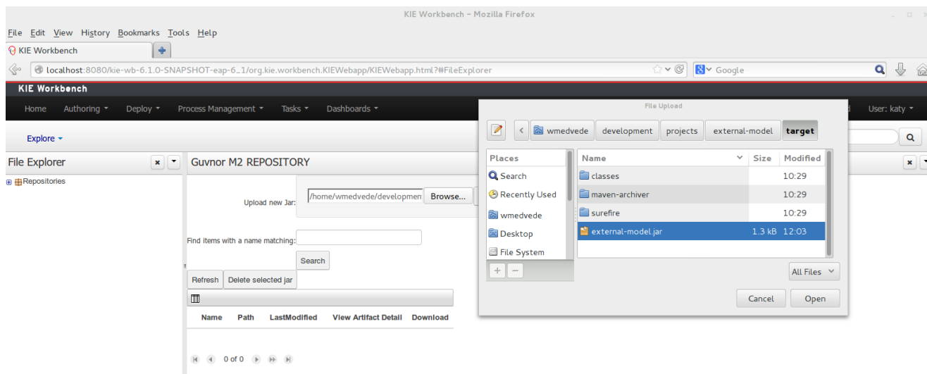
Figure 15.71. File browser.
