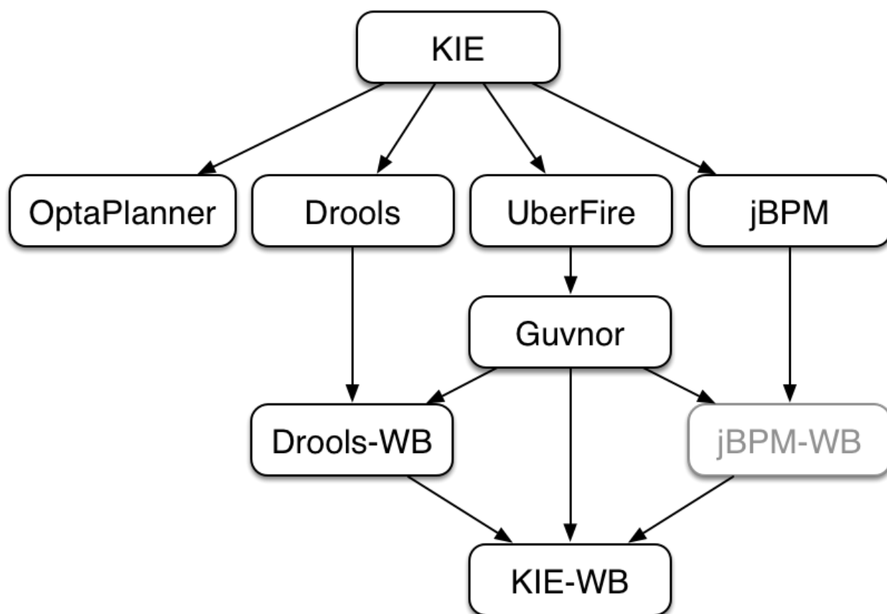
Figure 2.1. KIE Anatomy
