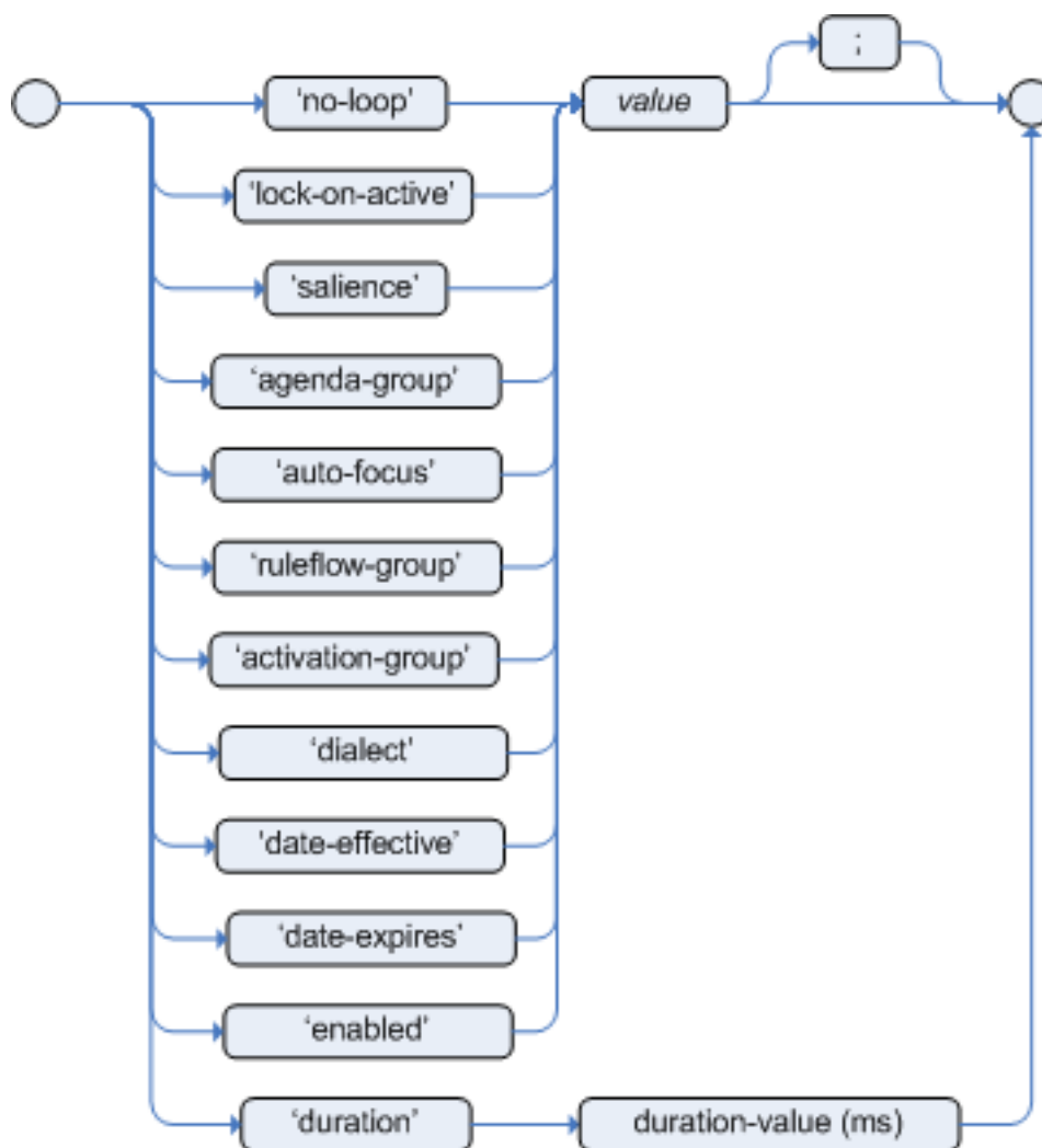
Figure 7.10. rule attributes
