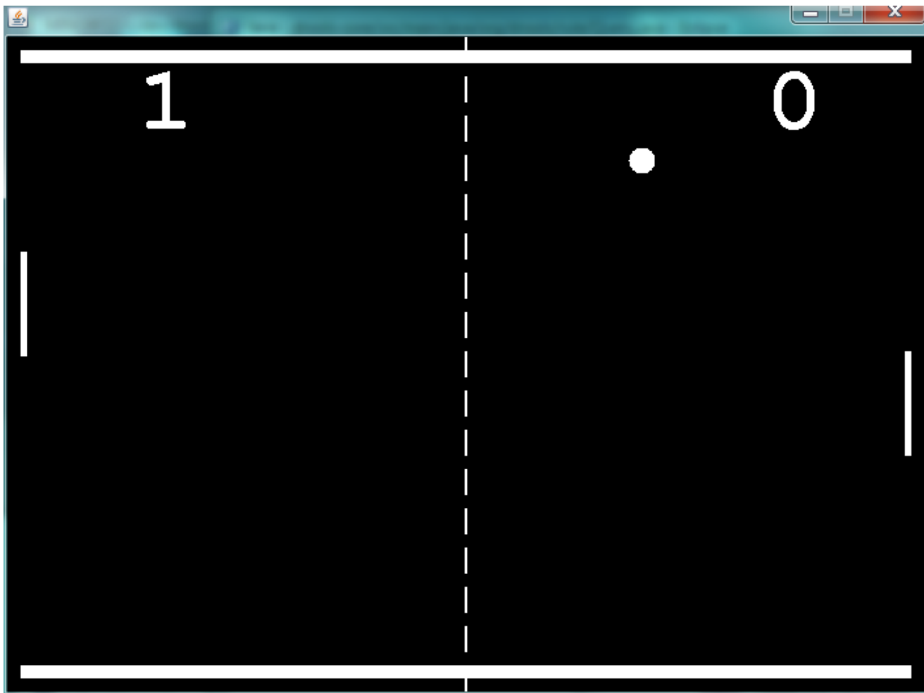
Figure 19.30. Pong Screenshot
