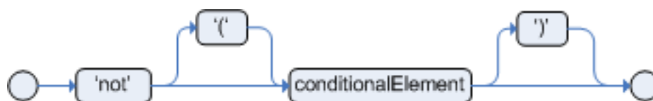
Figure 7.22. not
