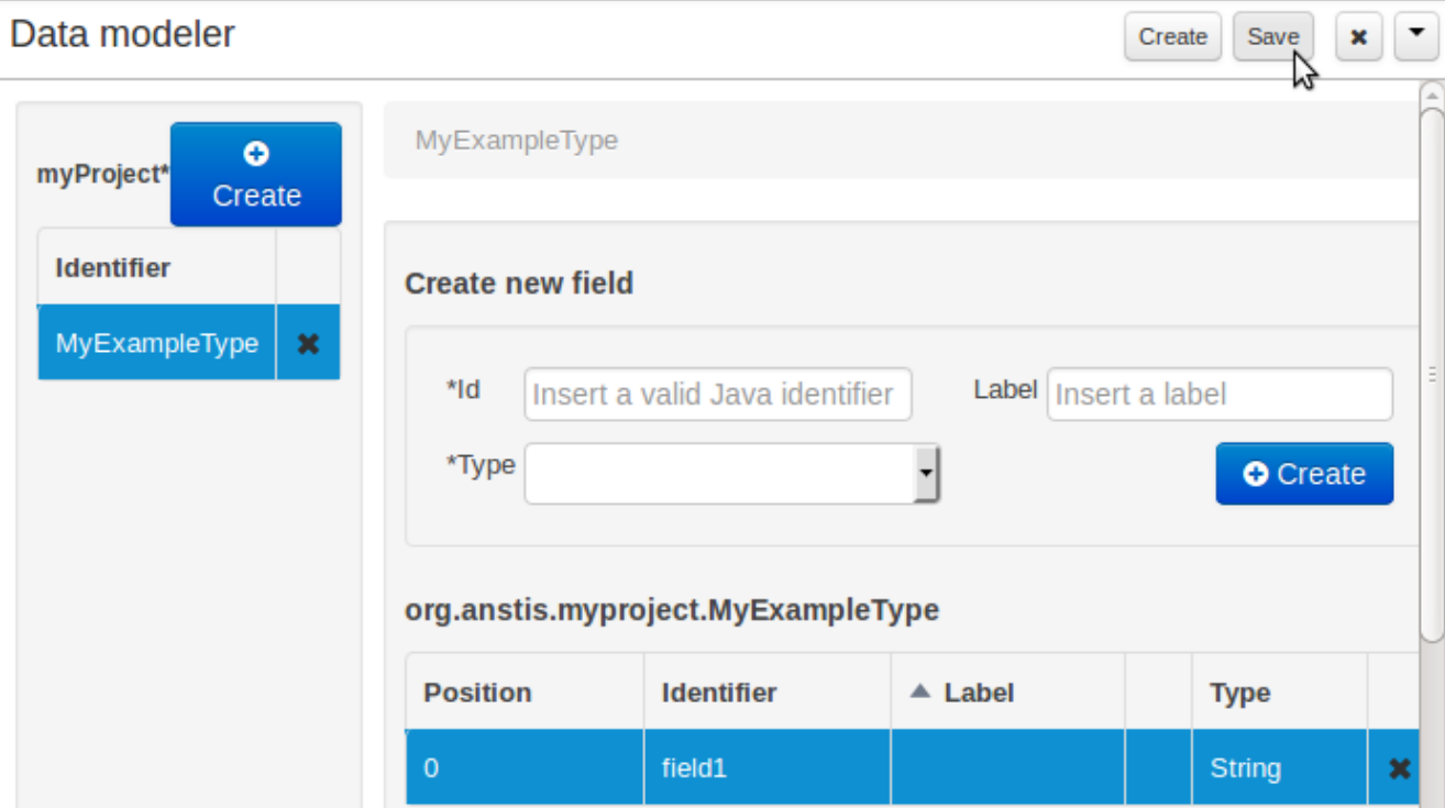
Figure 15.12. Clicking "Save"
