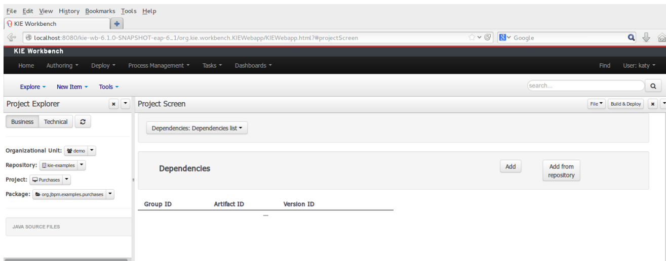
Figure 15.66. Project editor.
