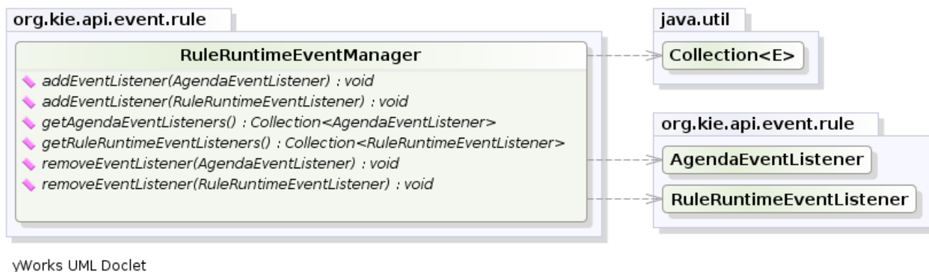
Figure 4.19. RuleRuntimeEventManager
