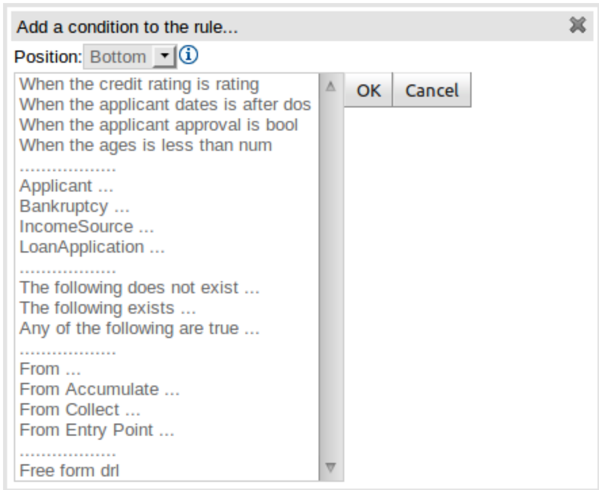
Figure 16.8. Adding Patterns
