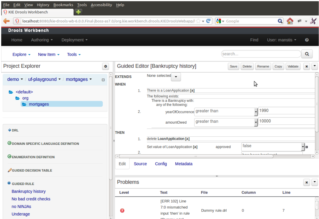
Figure 2.2. Workbench
