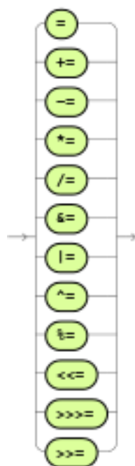
BindingPattern
