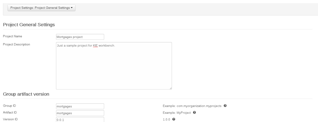
Figure 15.41. Project Settings
