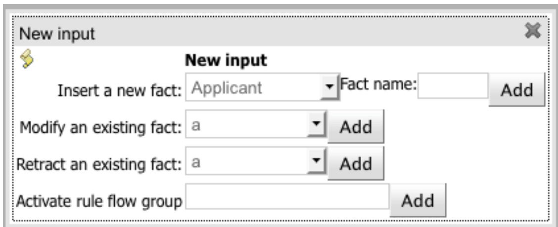
Figure 16.55. Given popup
