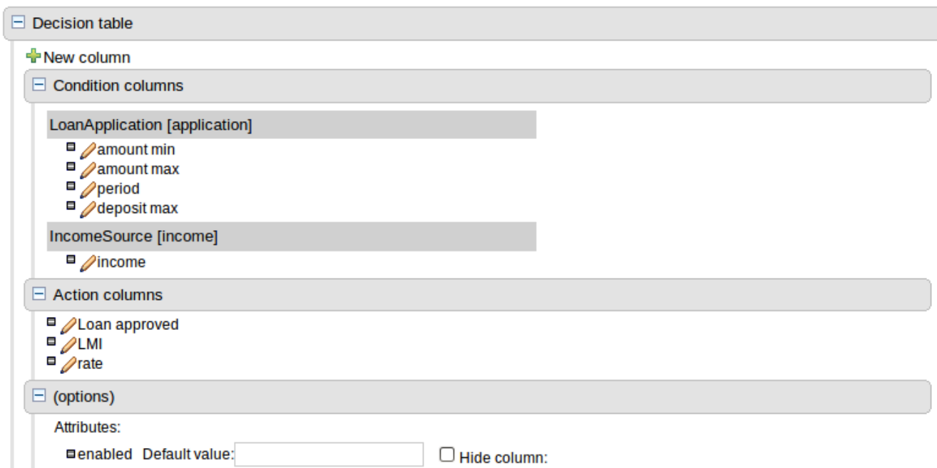
Figure 16.26. Column configuration
