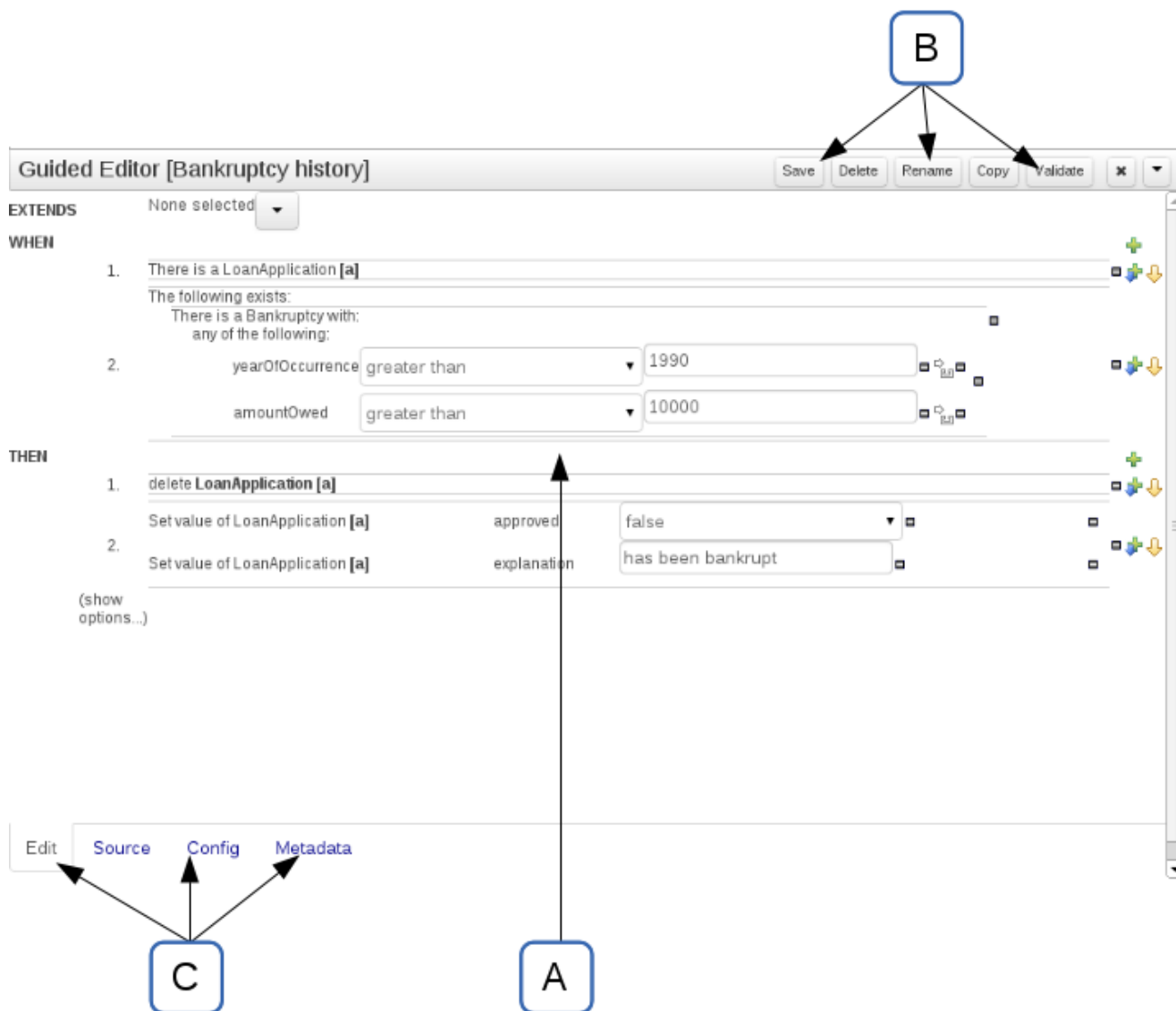
Figure 15.23. The Asset Editor - Edit tab
