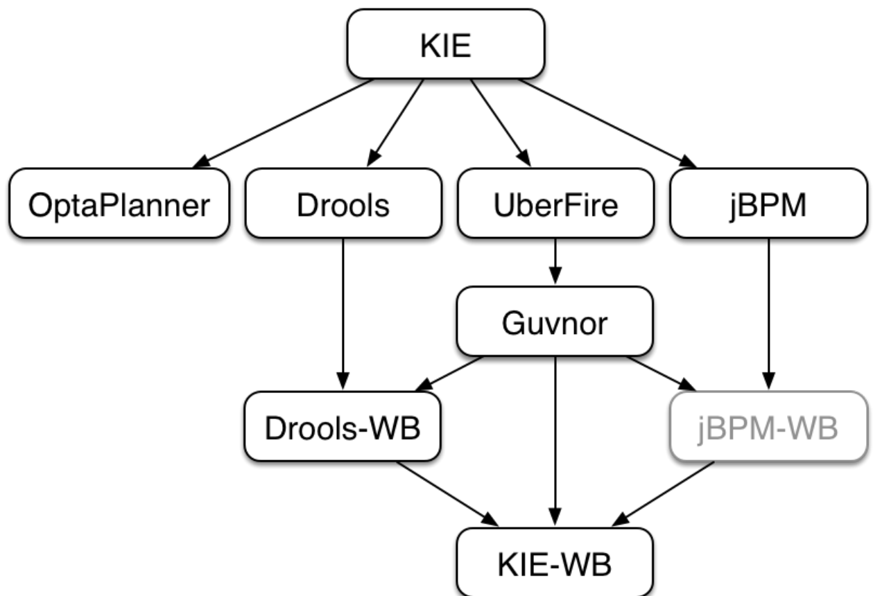
Figure 2.19. KIE Anatomy
