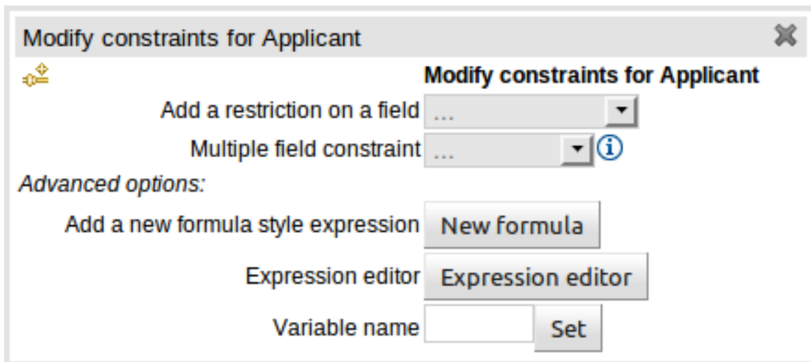
Figure 16.9. Adding constraints
