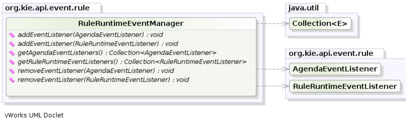
Figure 4.19. RuleRuntimeEventManager
