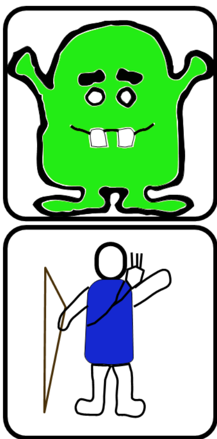
Figure 19.35. Wumpus World
