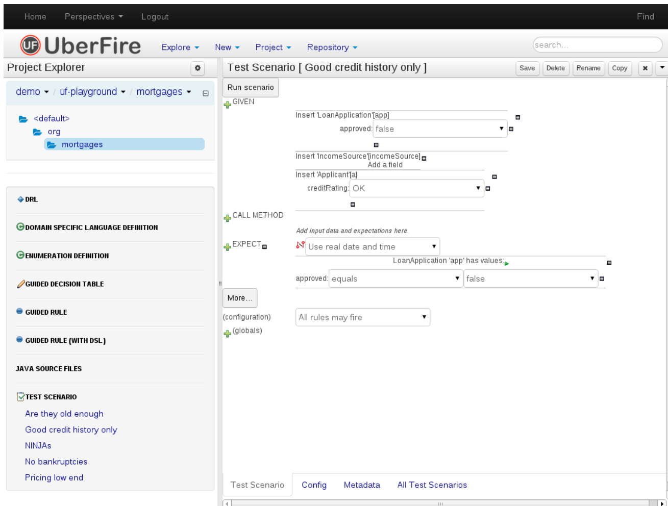
Figure 16.64. Example Test Scenario
