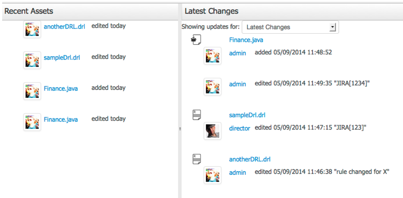
Figure 2.10. Timeline Perspective
