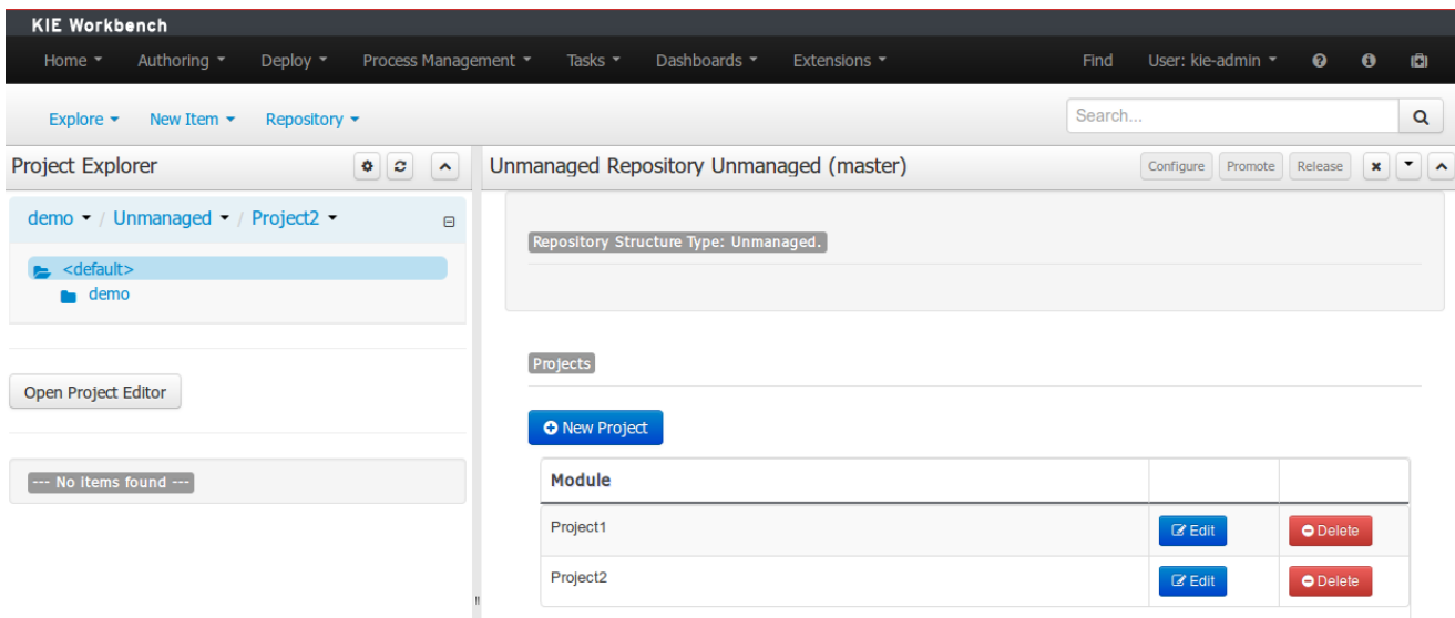
Figure 15.83. Unmanaged Repository
