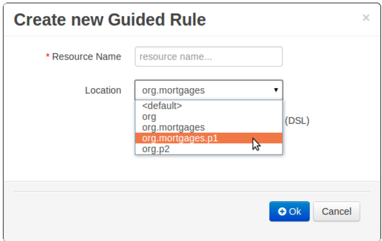
Figure 2.14. Package selector
