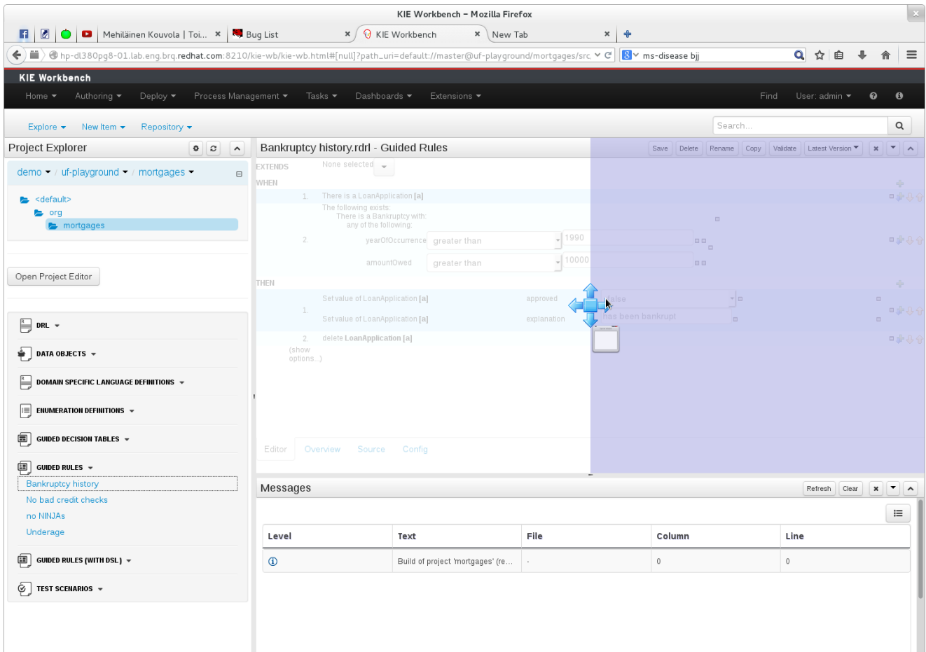
Figure 15.21. Repositioning - dragging
