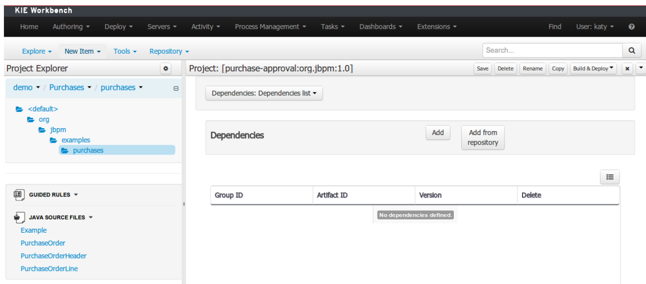
Figure 15.61. Project editor.
