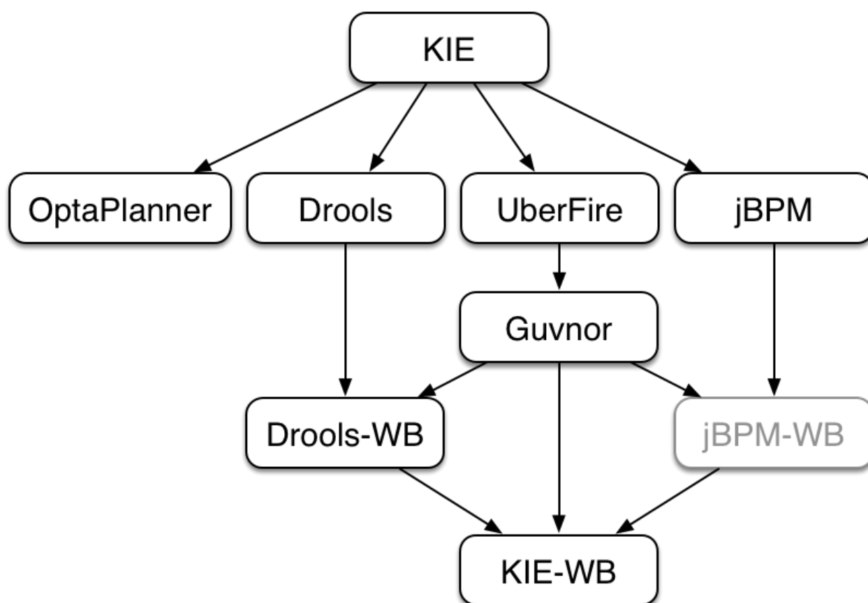
Figure 2.27. KIE Anatomy
