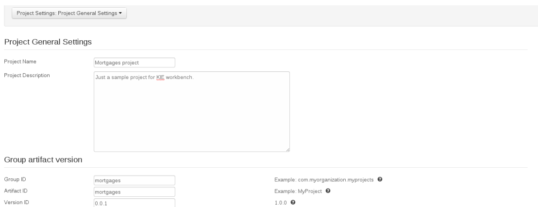
Figure 15.40. Project Settings
