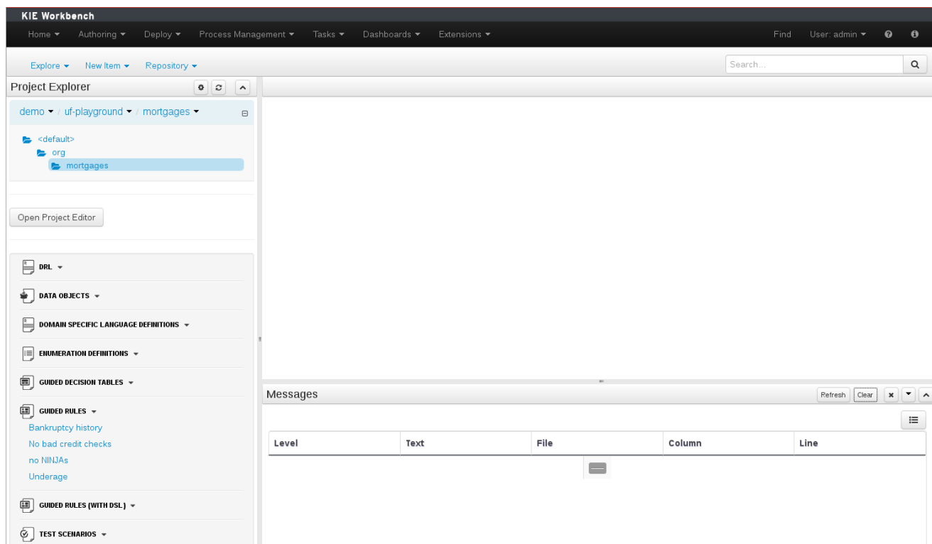
Figure 15.19. The Workbench
