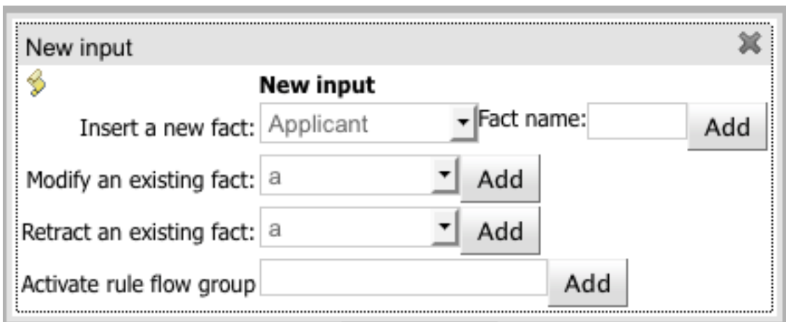
Figure 16.66. Given popup
