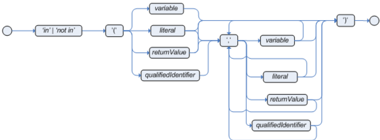
Figure 7.16. compoundValueRestriction
