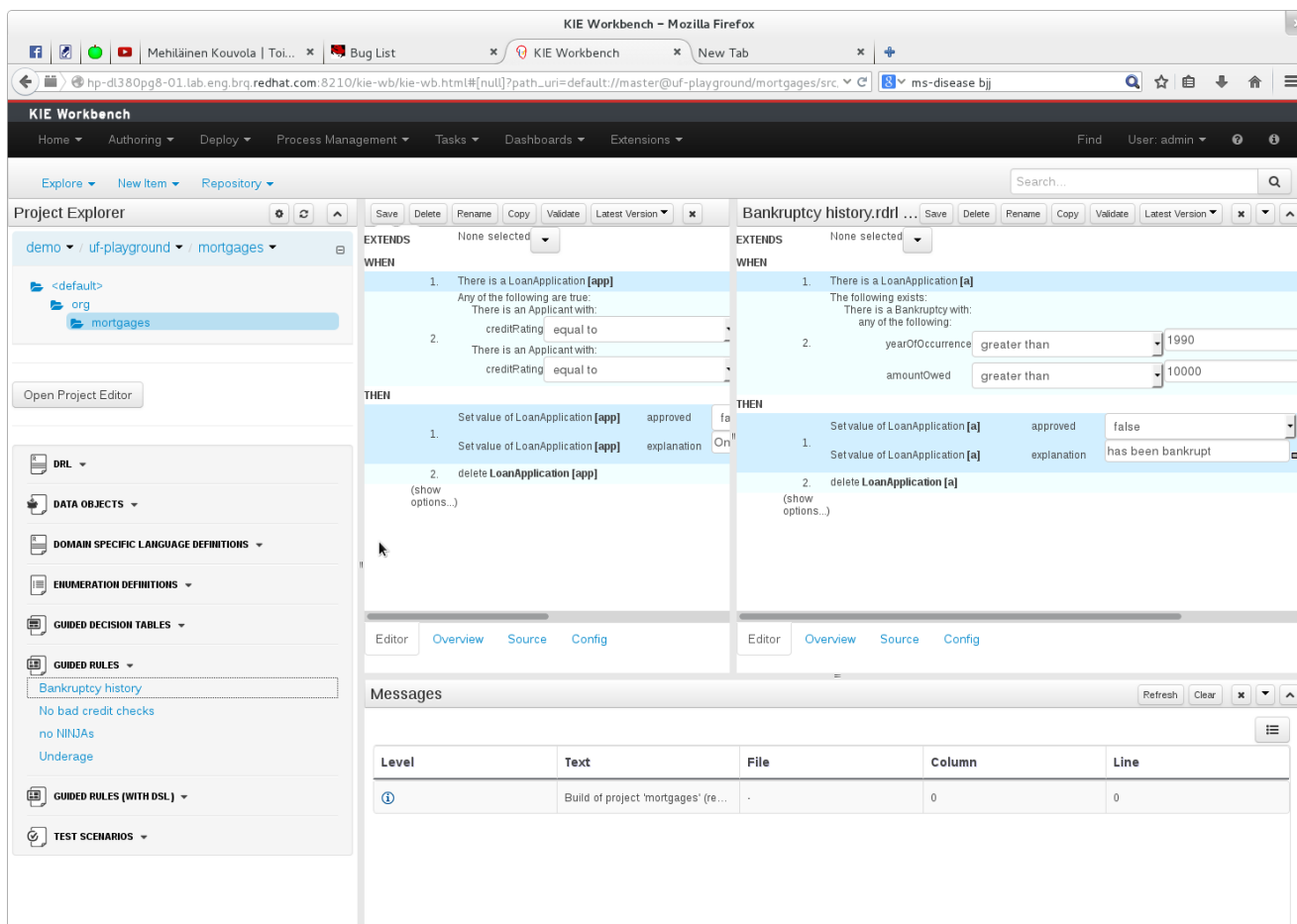
Figure 15.22. Repositioning - complete
