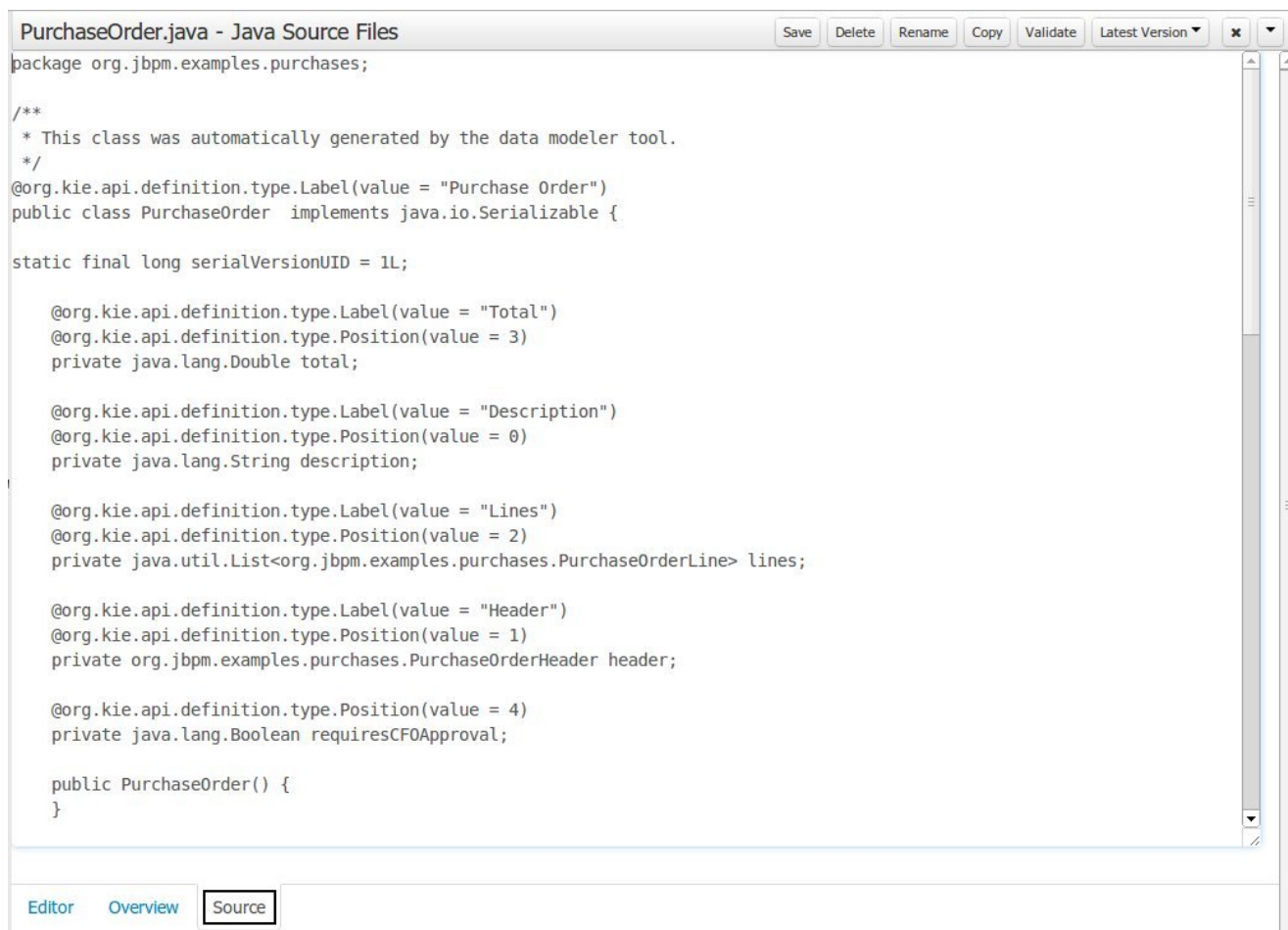
Figure 15.51. Source editor
