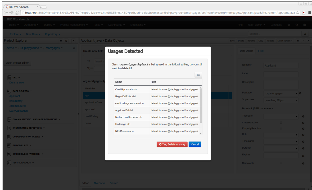
Figure 2.8. Usages detection
