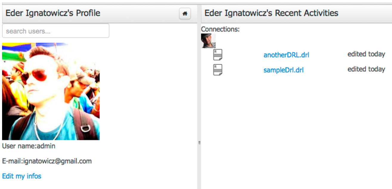
Figure 2.11. People Perspective
