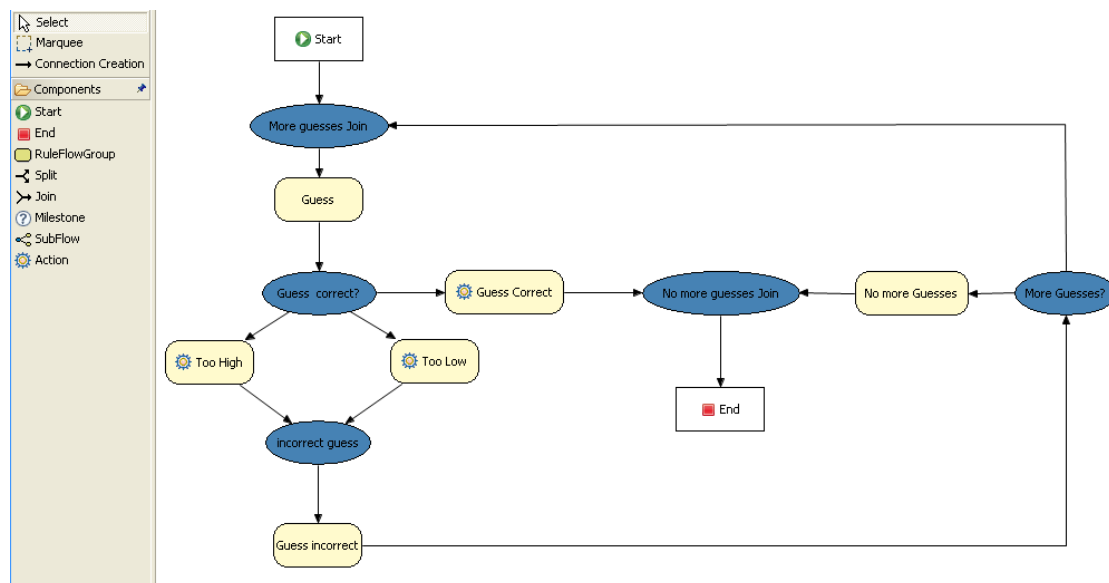
Figure 20.23. RuleFlow for the NumberGuess Example
