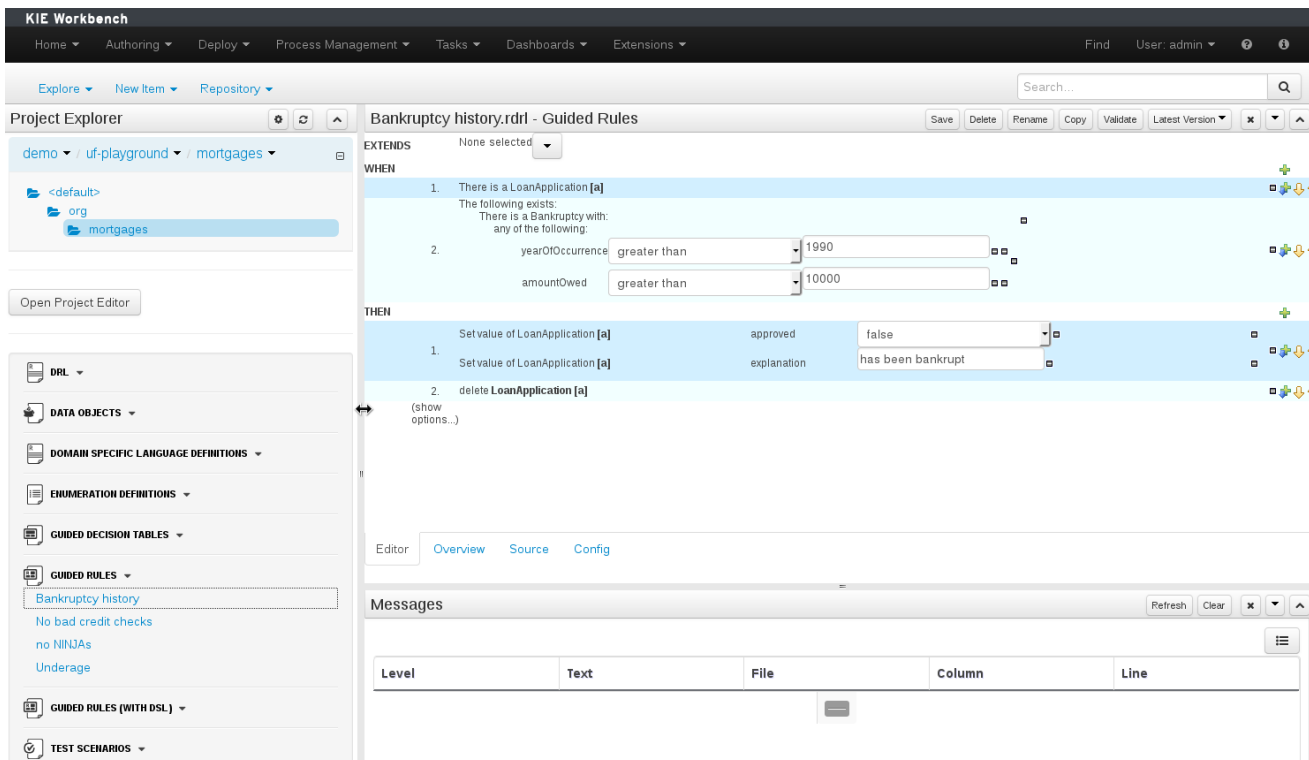
Figure 15.20. Resizing
