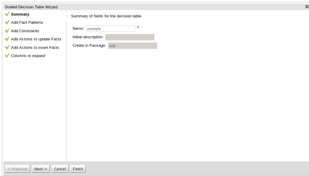
Figure 16.37. Summary page
