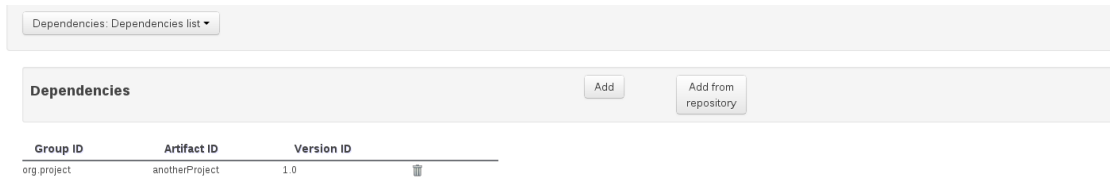
Figure 15.41. Dependencies
