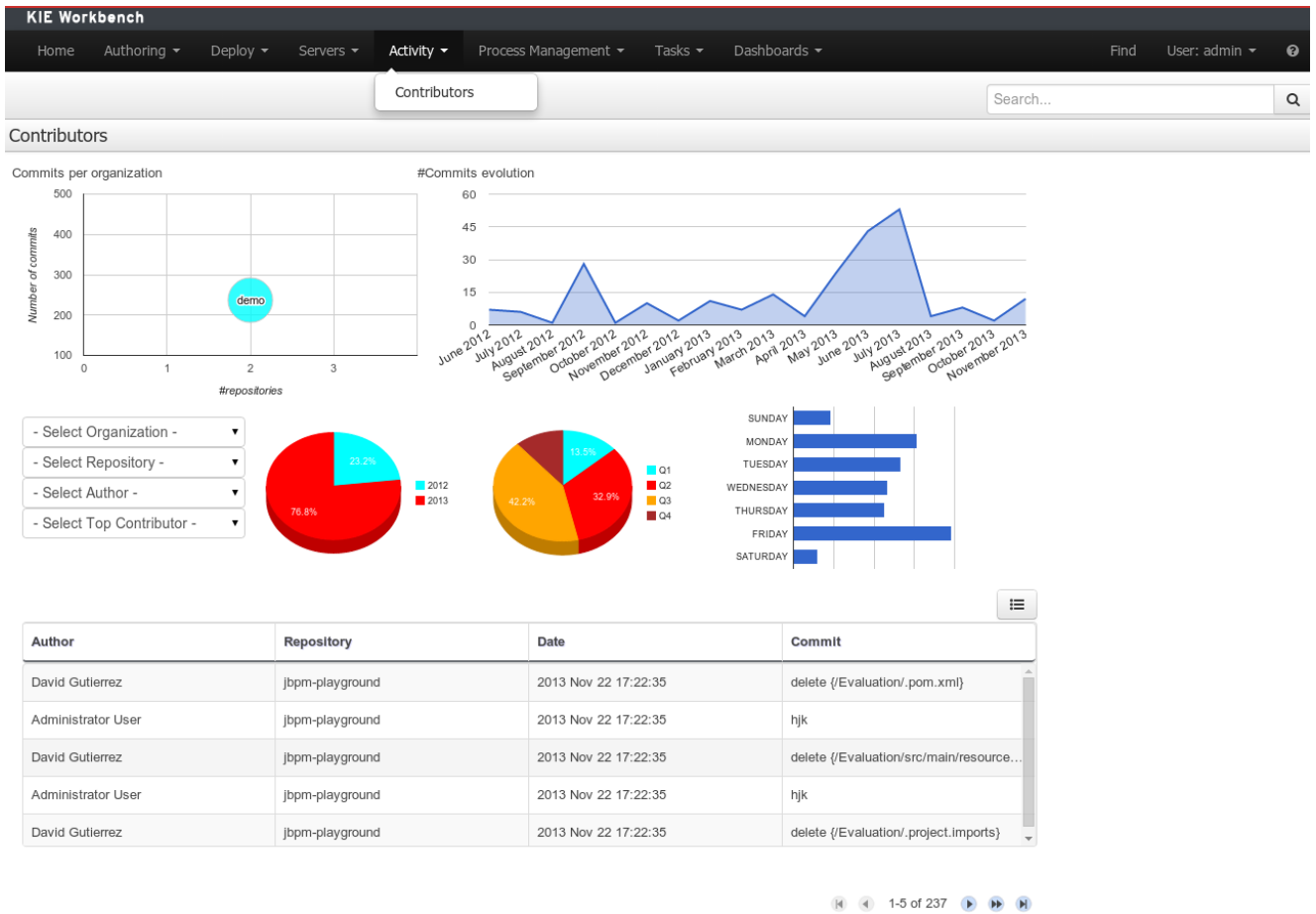
Figure 2.13. Contributors perspective
