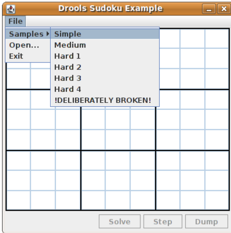
Figure 20.18. Initial screen
