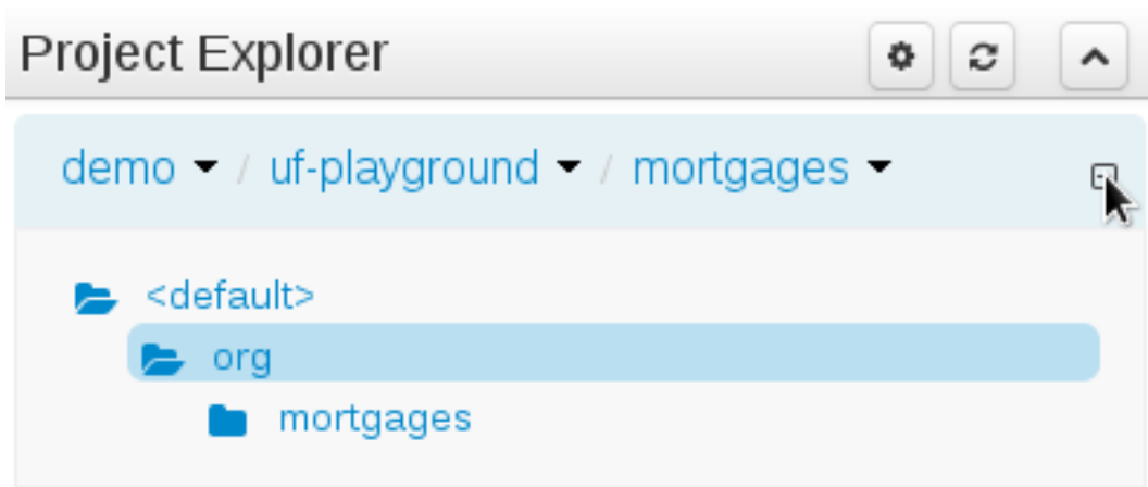
Figure 15.28. Showing packages
