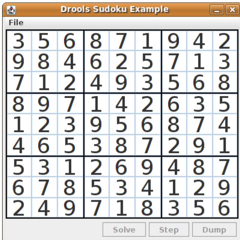
Figure 20.20. "Simple" Solved
