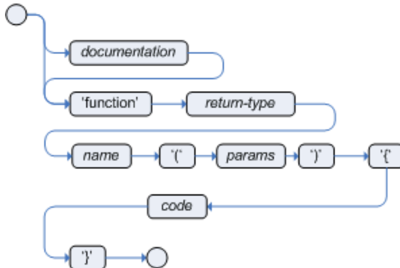
Figure 7.6. function
