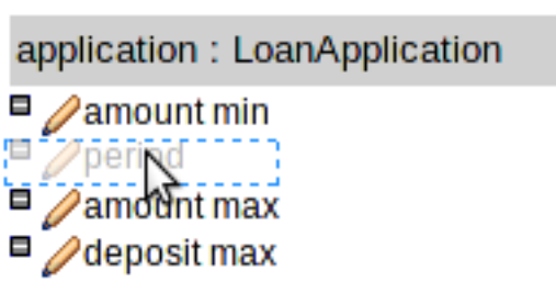
Figure 16.25. Re-arranging columns
