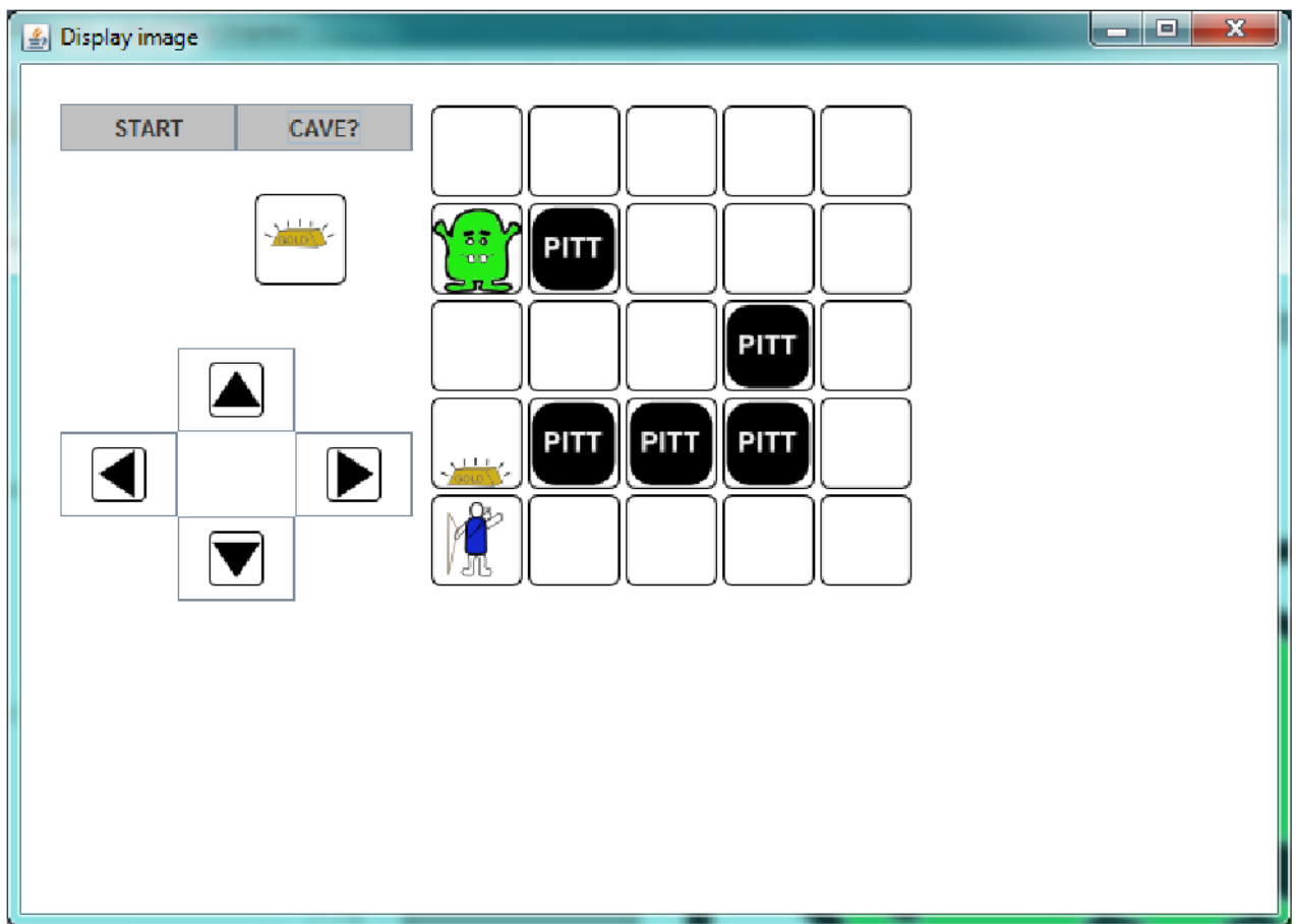
Figure 20.36. Cave Screenshot
