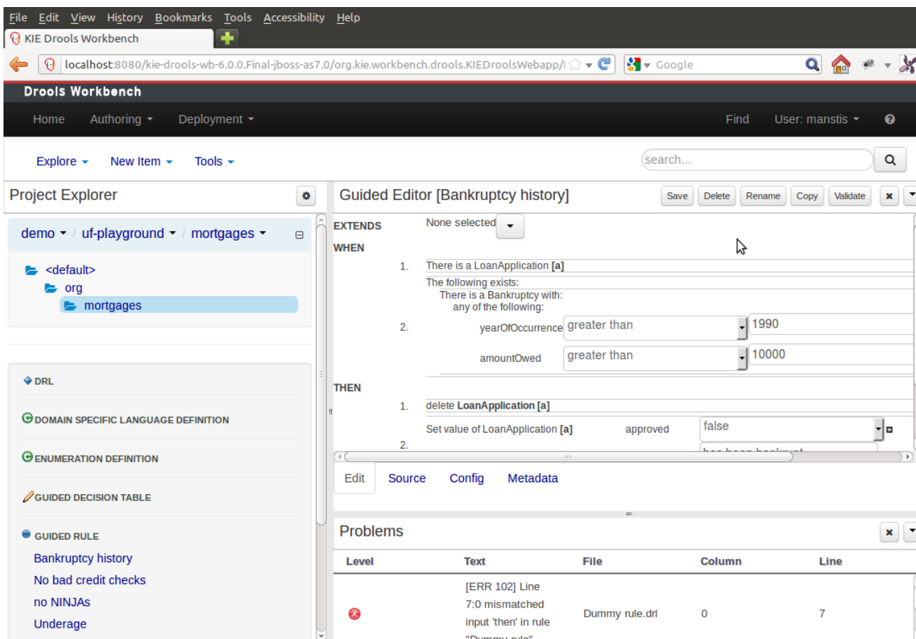
Figure 2.28. Workbench
