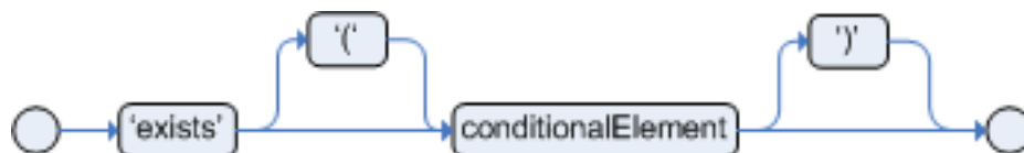
Figure 7.23. exists
