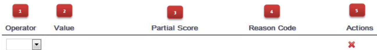
Figure 16.63. New Attribute
