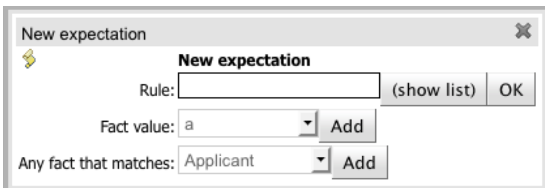
Figure 16.67. Expect popup
