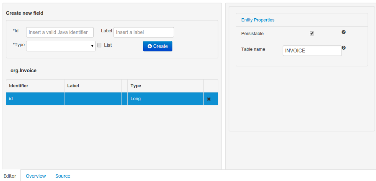
Figure 2.3. Data Object level JPA domain editor
