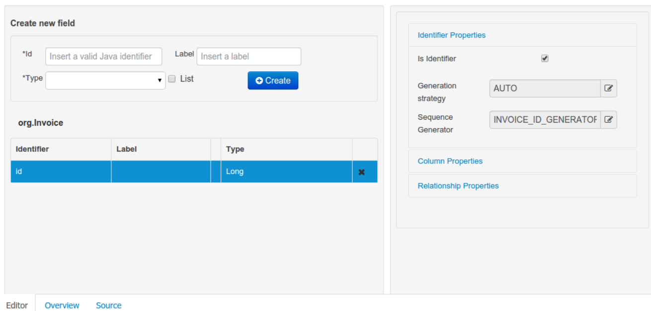
Figure 2.4. Field level JPA domain editor
