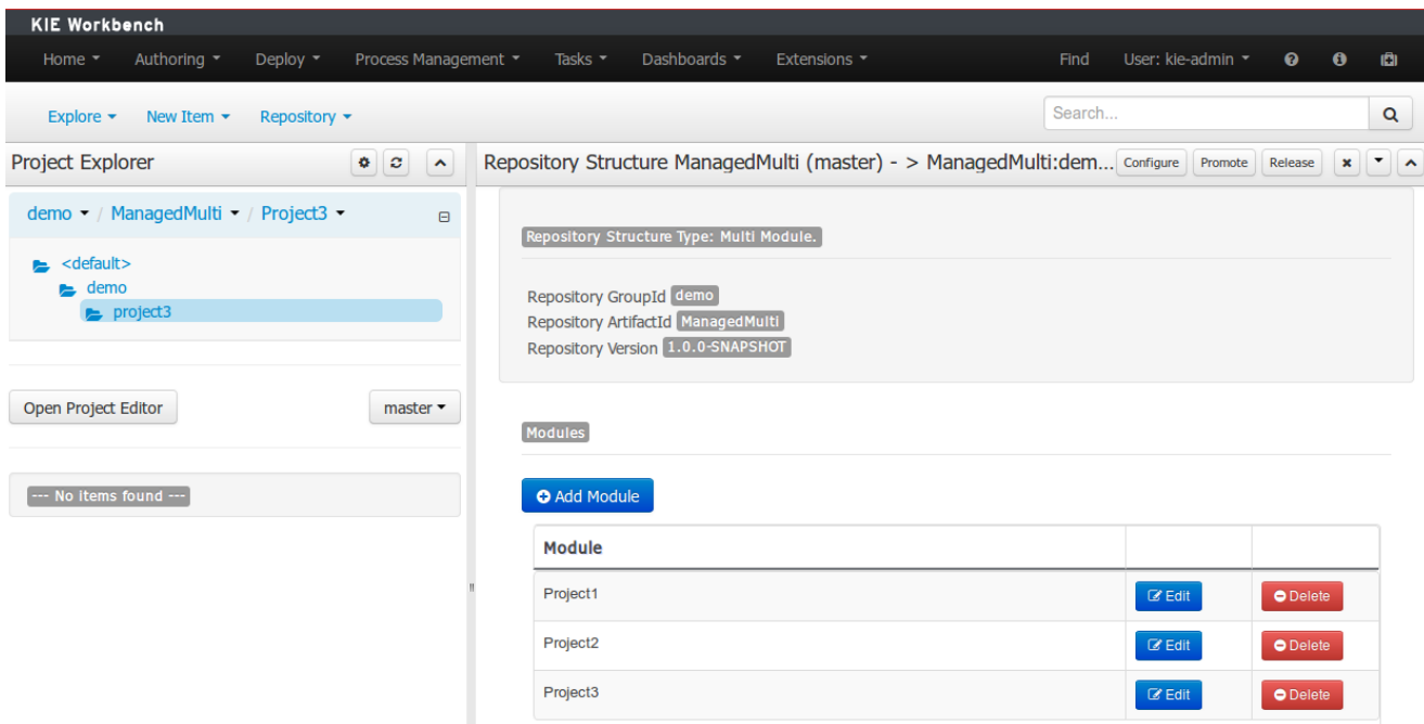
Figure 18.98. Multi Project Managed Repository
