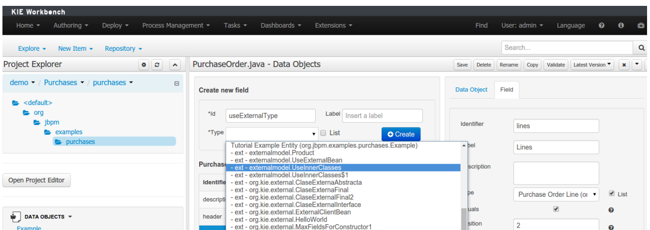
Figure 18.78. Identifying external objects.
