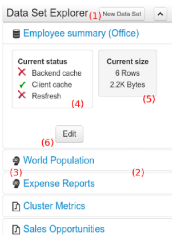
Figure 18.84. Data Set Explorer
