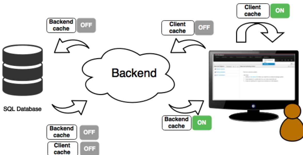
Figure 18.94. Data set caching
