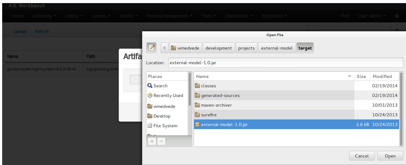
Figure 18.90. File browser.
