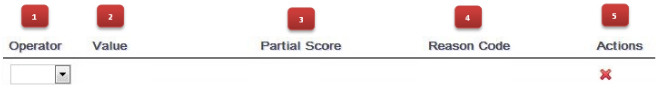
Figure 19.63. New Attribute
