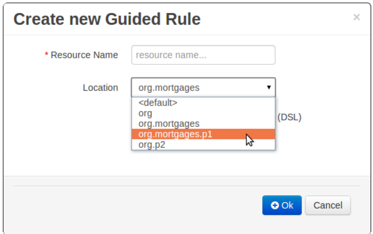
Figure 2.34. Package selector
