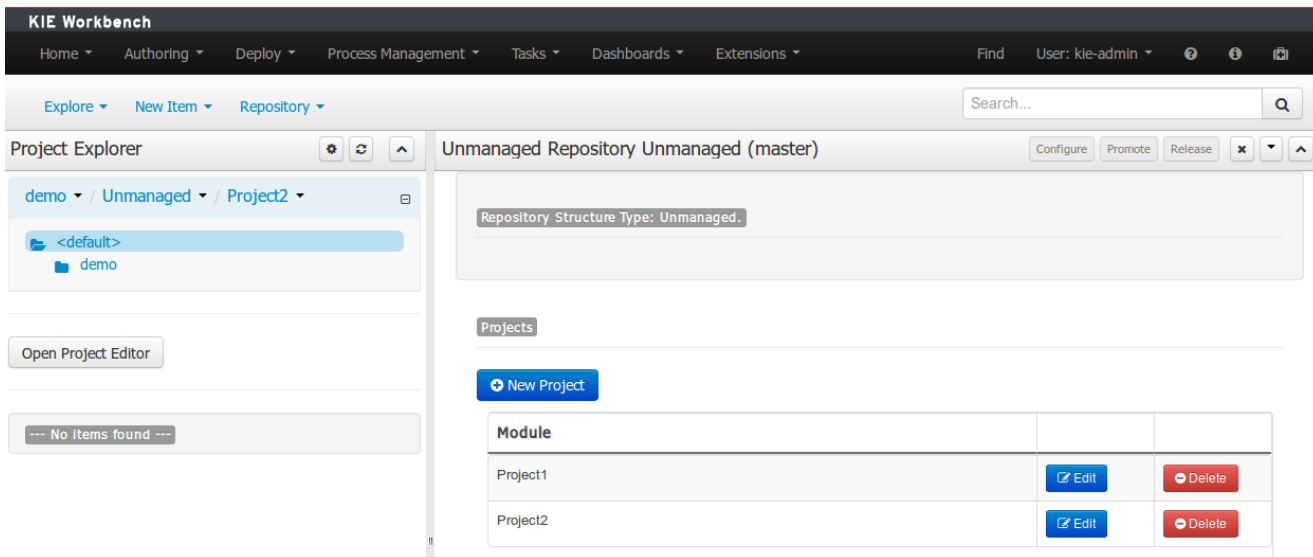
Figure 18.137. Unmanaged Repository
