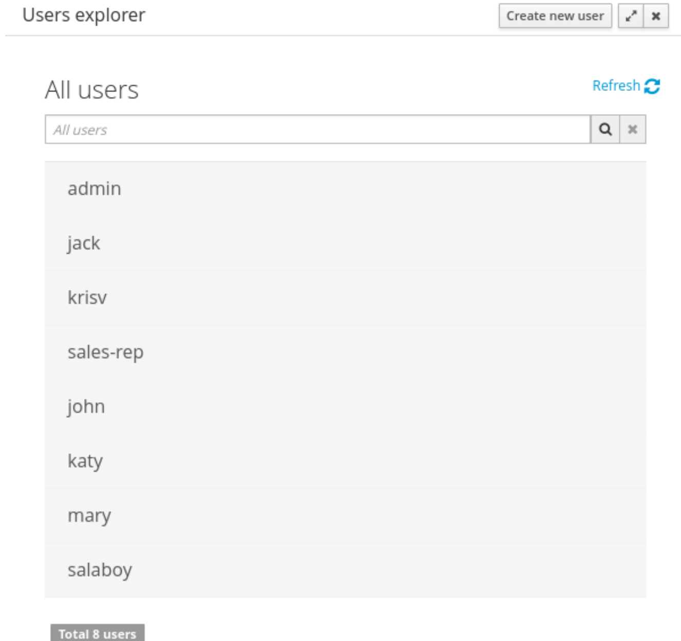
Figure 18.119.
