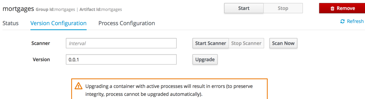
Figure 18.154. Version Configuration
