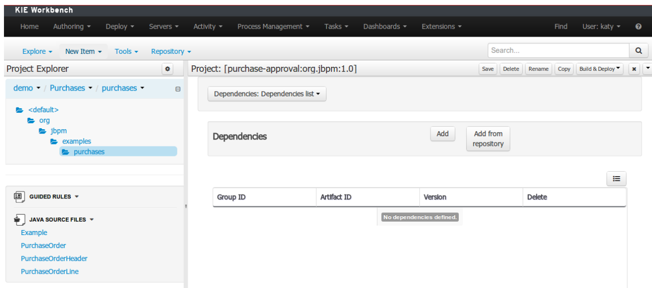
Figure 18.86. Project editor.
