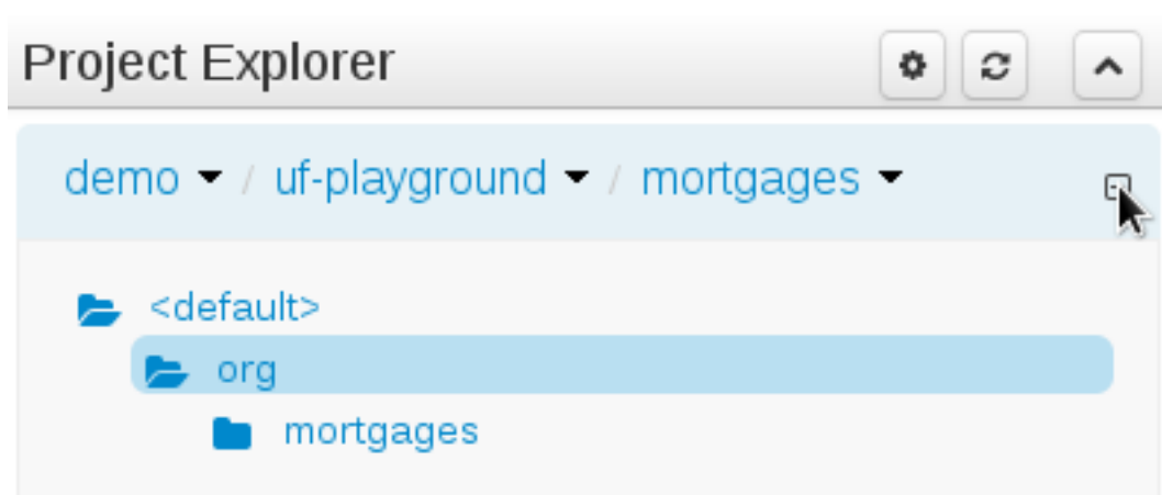
Figure 18.32. Showing packages
