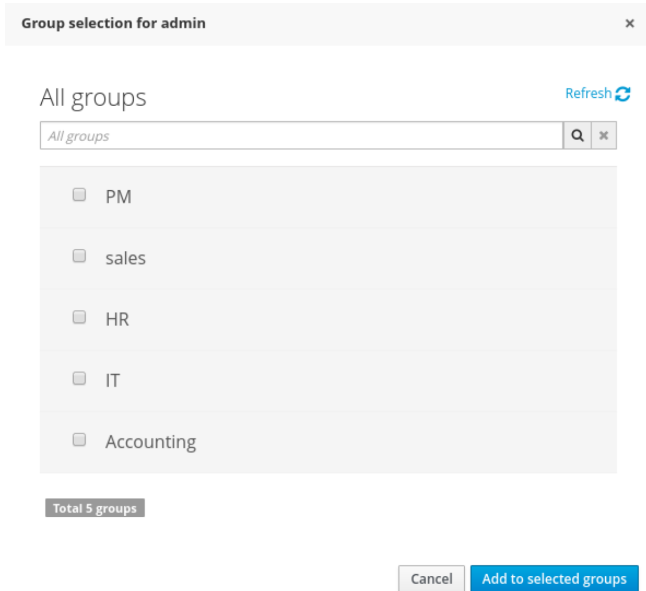
Figure 18.126.
