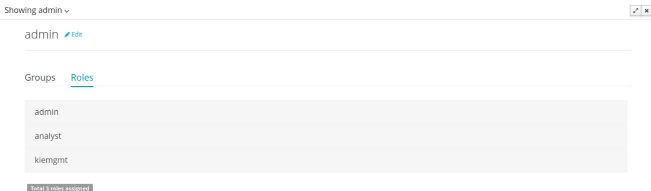
Figure 18.122.
