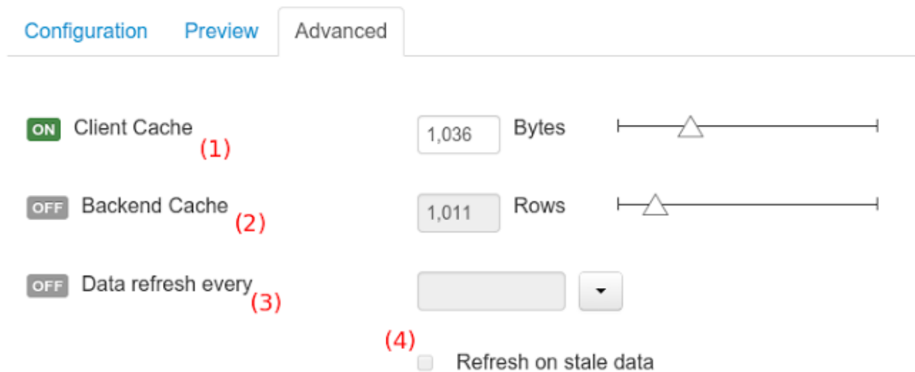
Figure 18.112. Advanced settings
