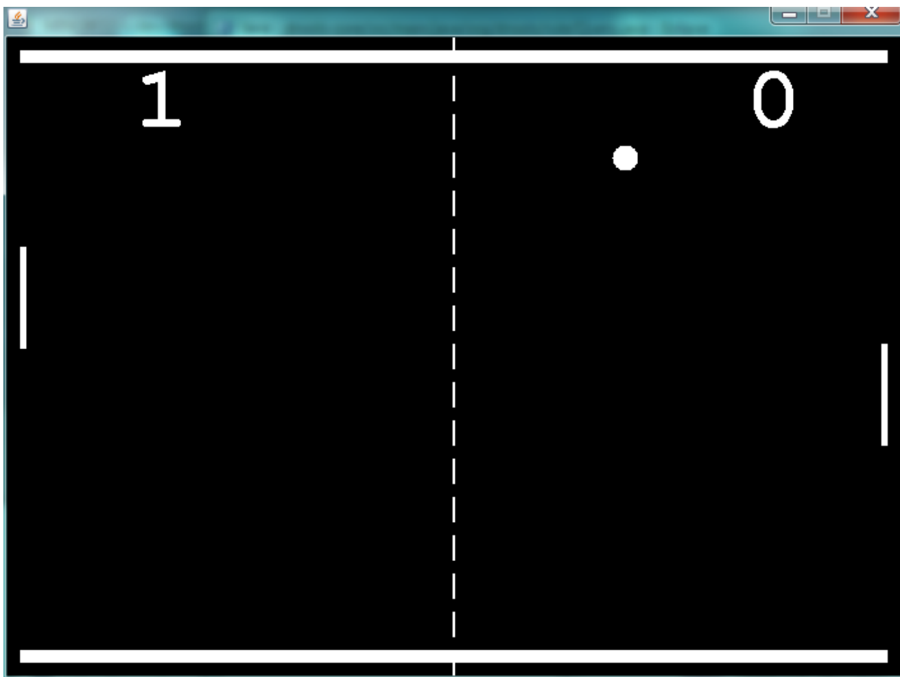
Figure 23.34. Pong Screenshot
