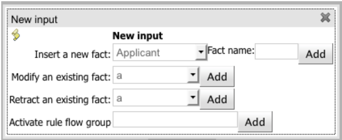
Figure 19.67. Given popup
