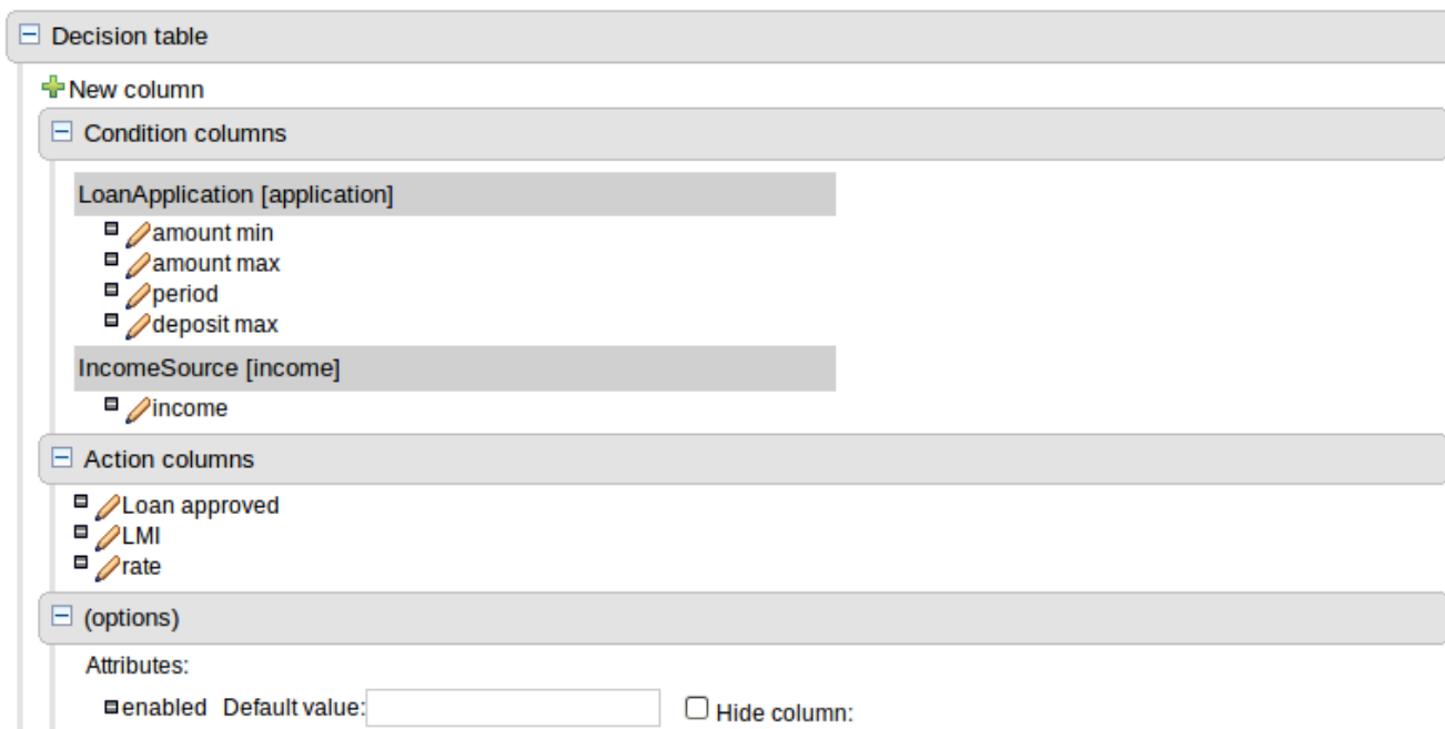
Figure 19.26. Column configuration
