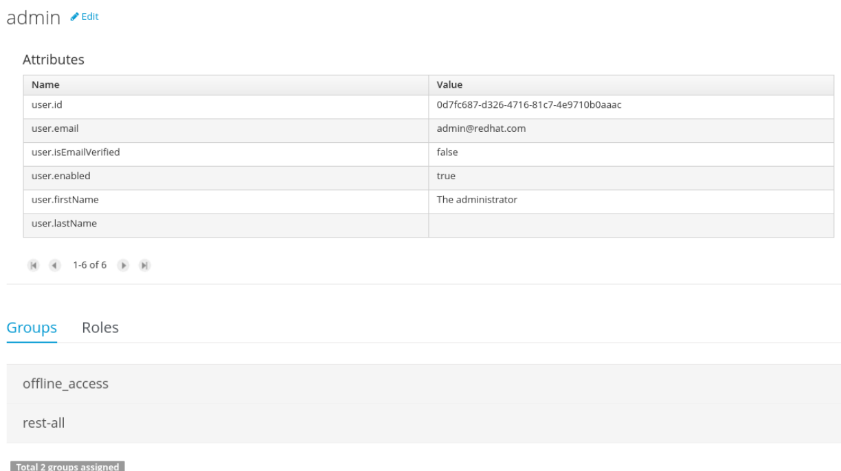
Figure 18.123.
