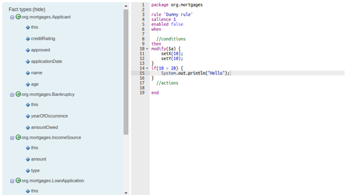
Figure 2.15. ACE Editor
