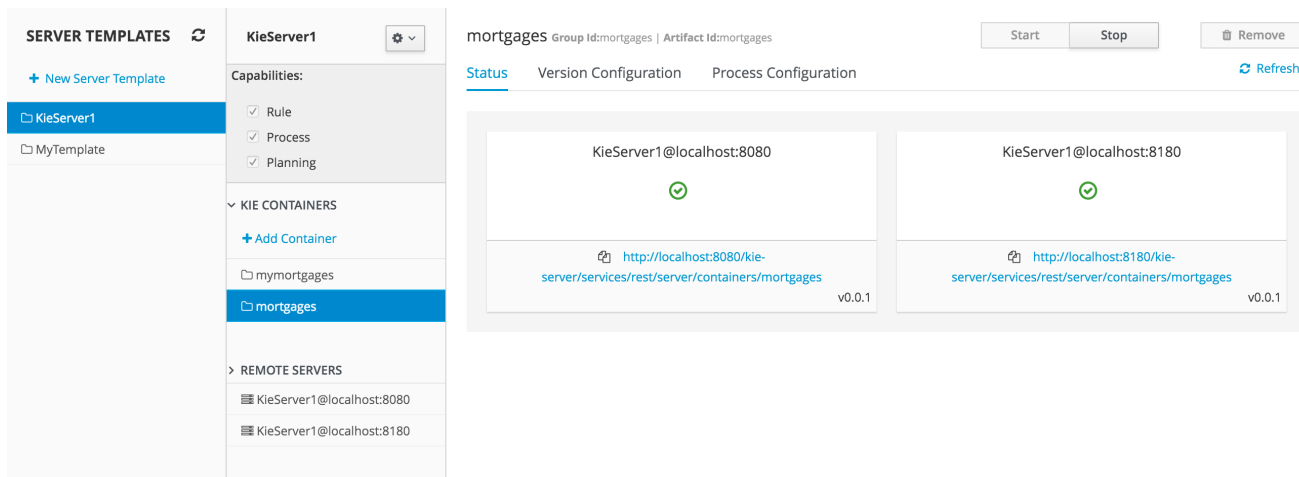
Figure 18.153. Status Container
