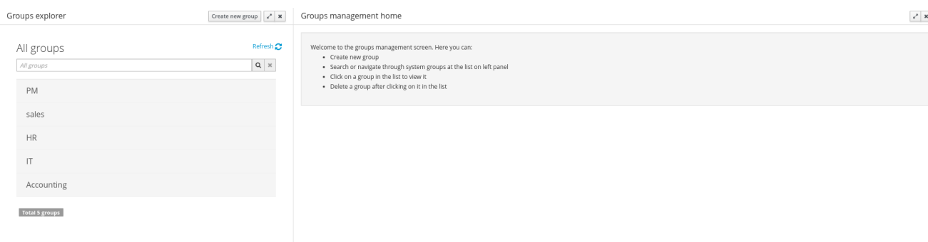
Figure 18.129.
