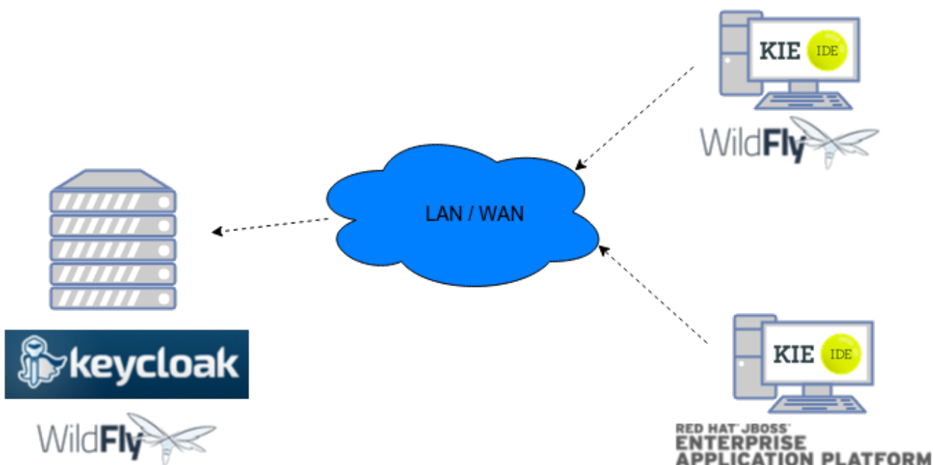
Figure 20.1.
