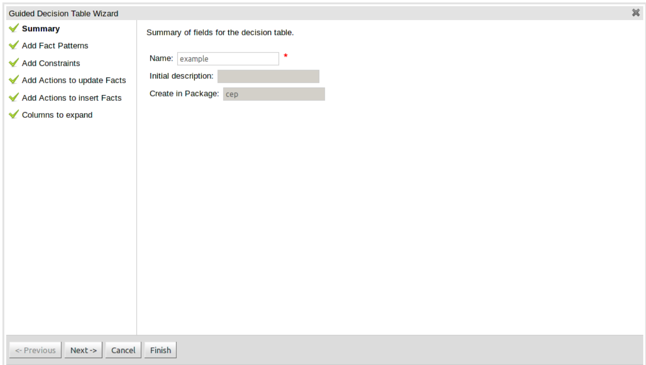
Figure 19.37. Summary page
