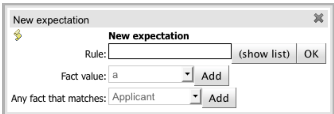
Figure 19.68. Expect popup
