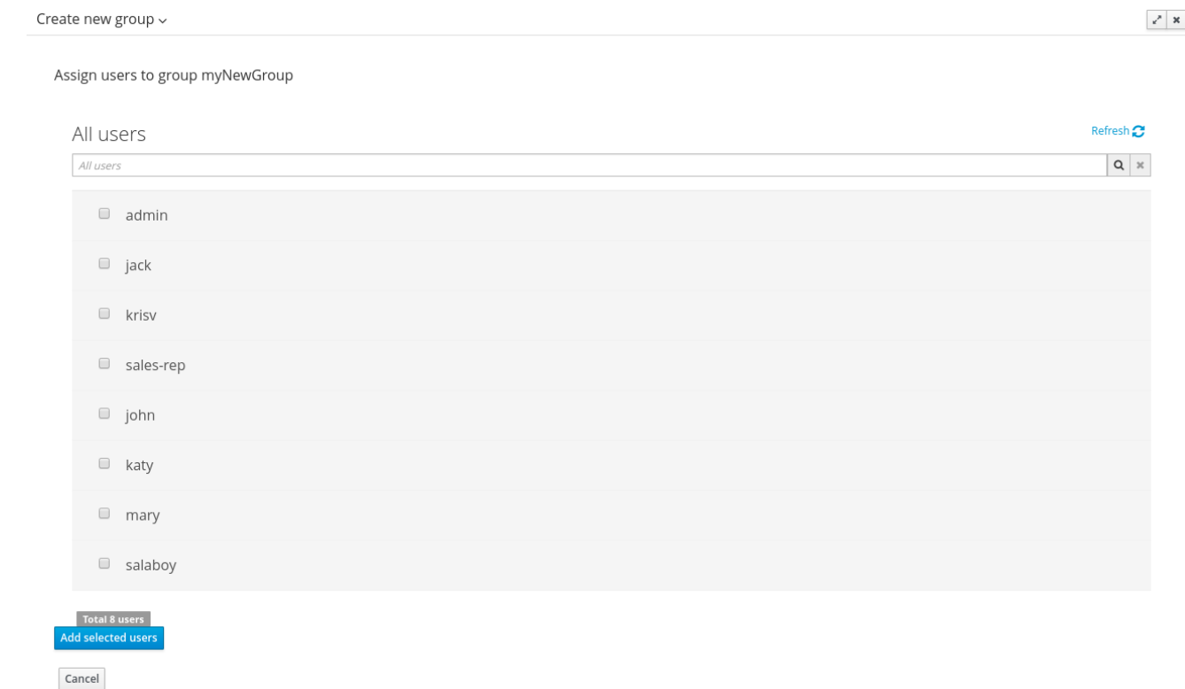
Figure 18.132.
