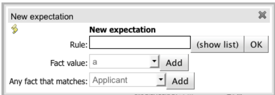
Figure 19.68. Expect popup
