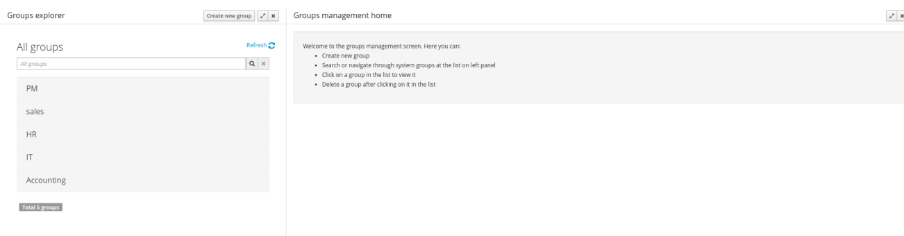
Figure 18.129.
