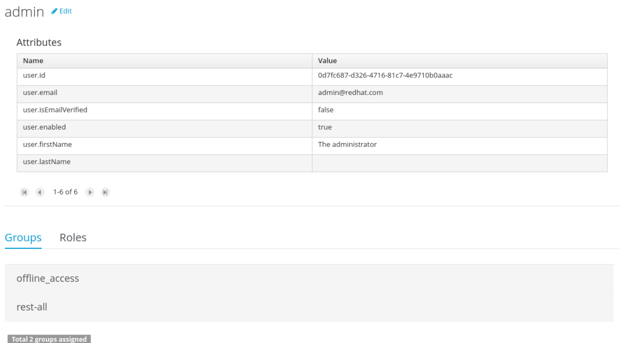
Figure 18.123.
