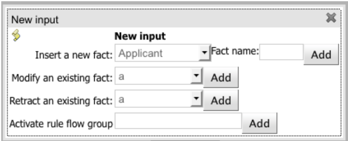
Figure 19.67. Given popup
