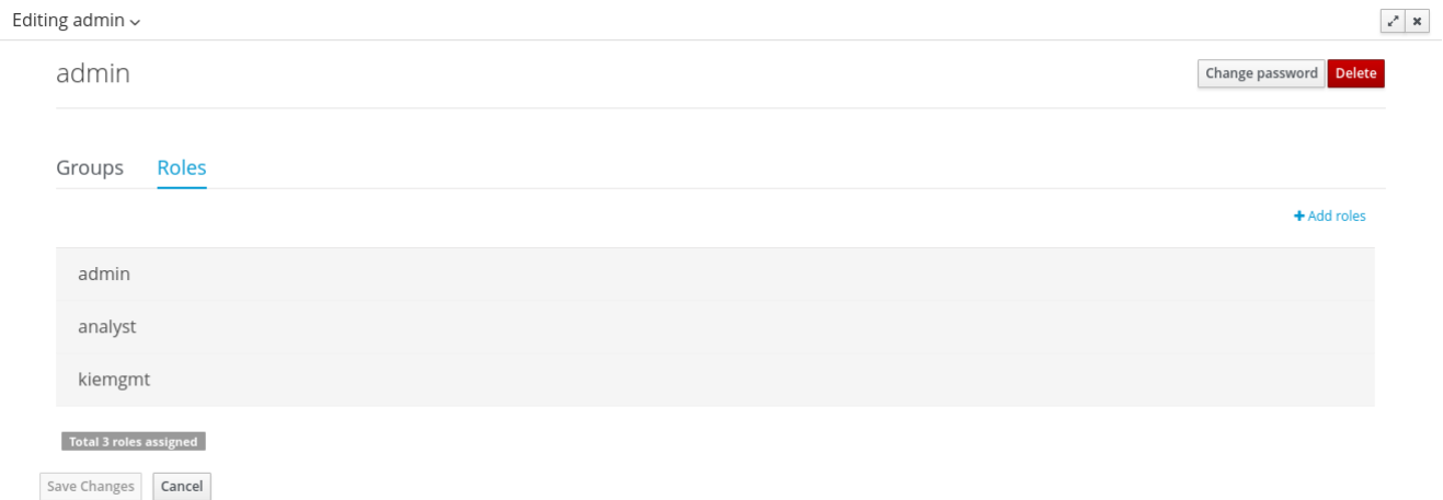
Figure 18.124.
