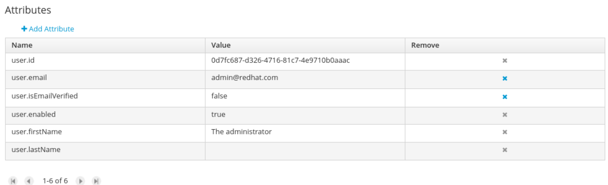
Figure 18.125.
