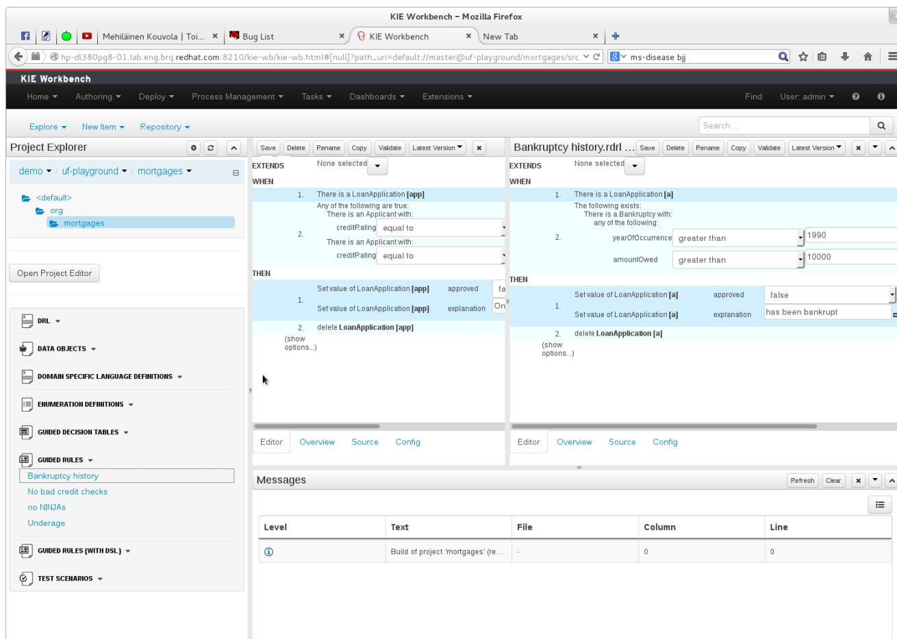
Figure 18.22. Repositioning - complete
