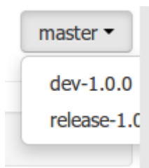
Figure 18.139. Branch Selector
