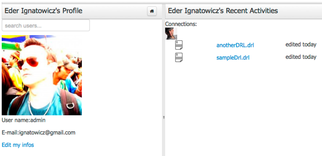
Figure 2.38. People Perspective
