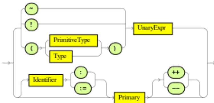
UnaryExpr
