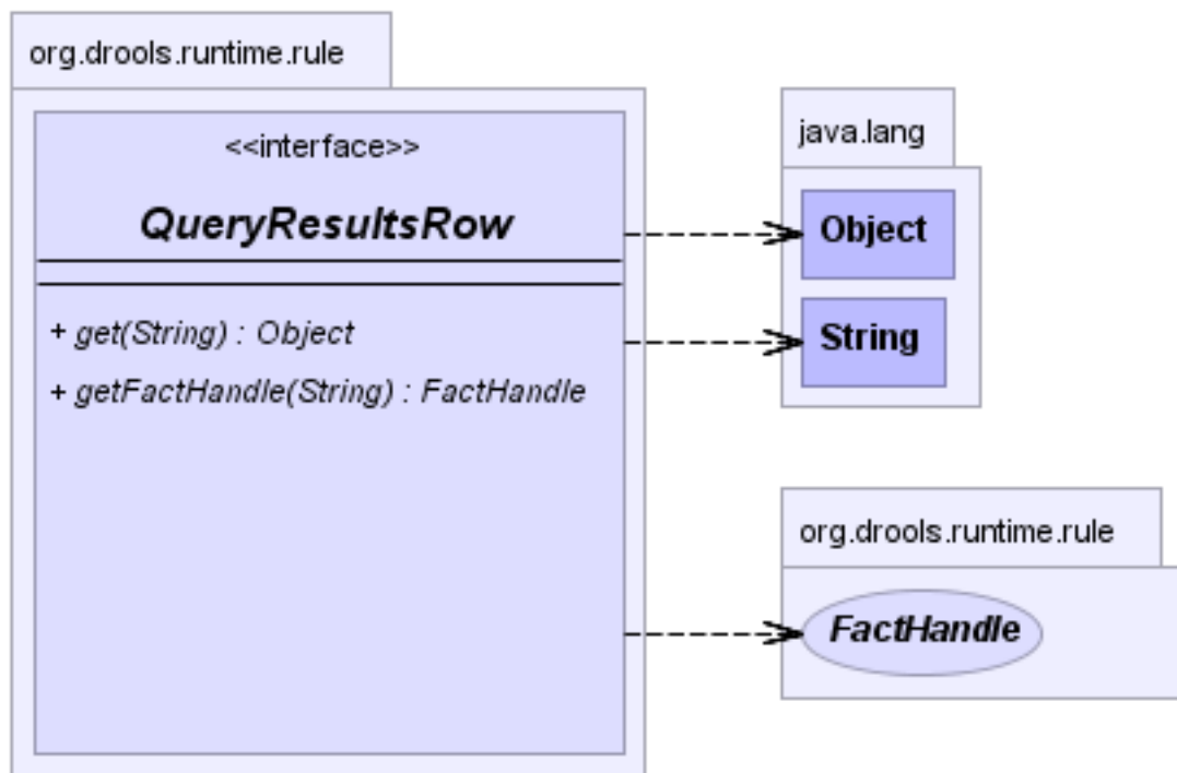
Figure 4.13. QueryResultsRow
