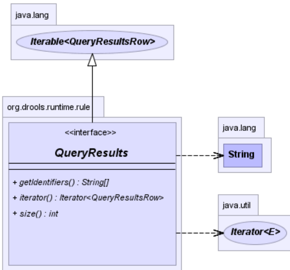
Figure 4.12. QueryResults
