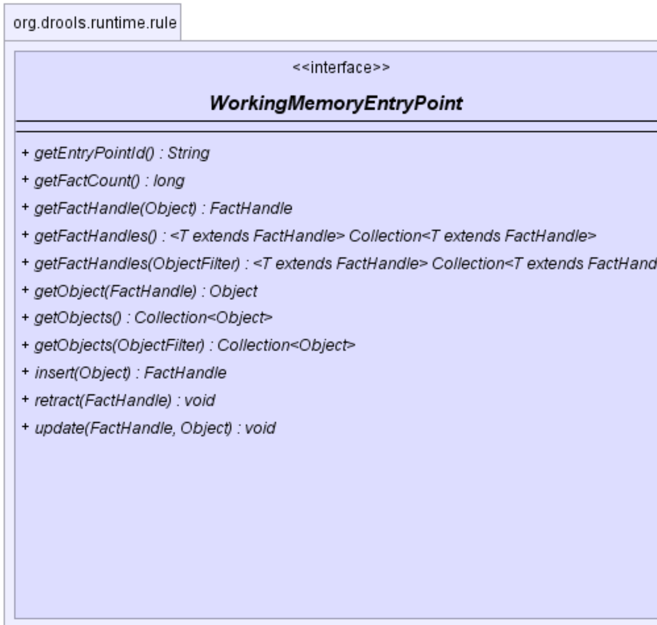
Figure 4.10. WorkingMemoryEntryPoint
