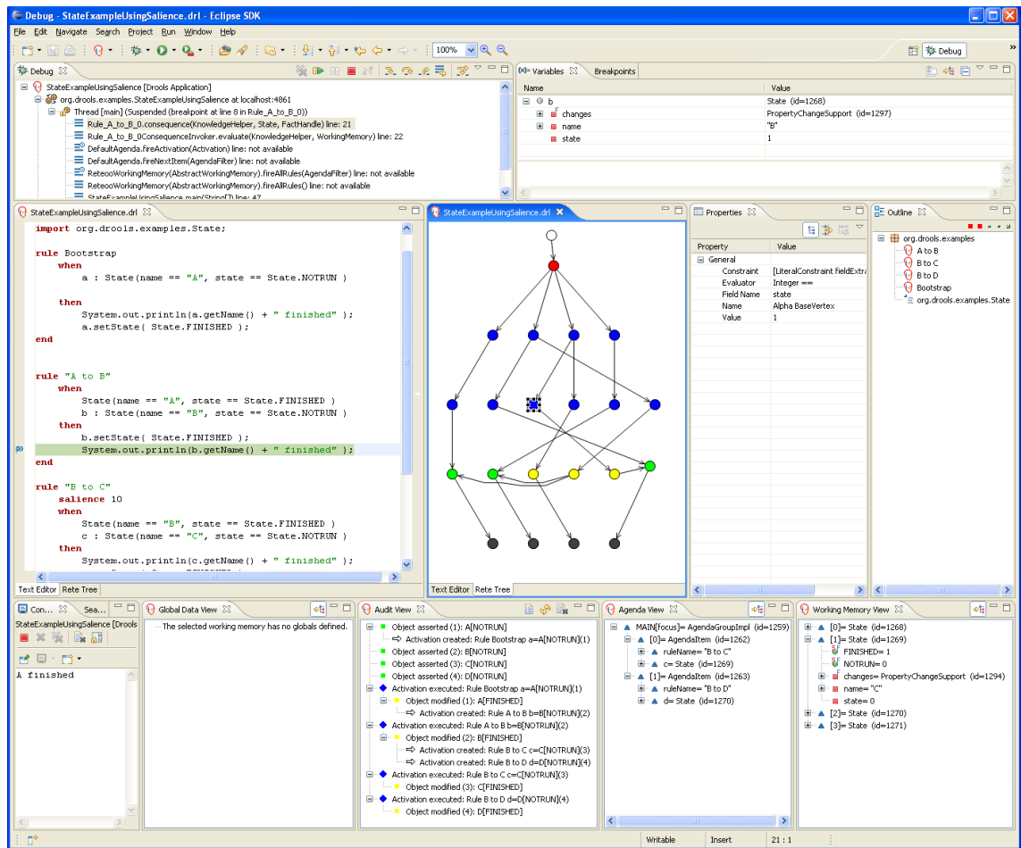
Figure 8.10. Debugging
