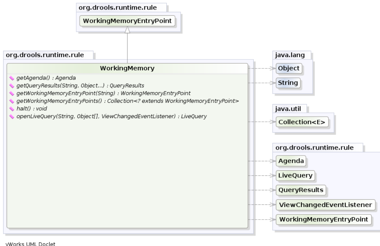
Figure 3.11. WorkingMemory
