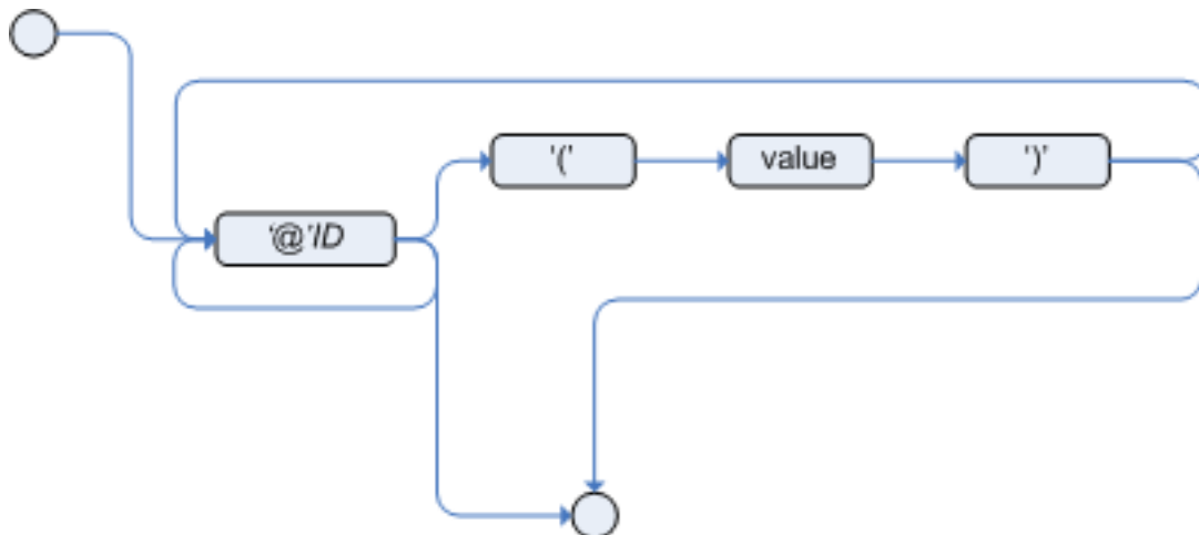
Figure 4.7. meta_data
