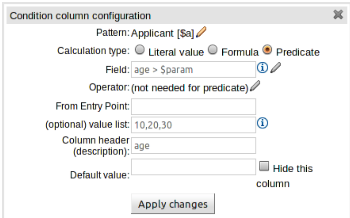
Figure 4.80. Defining a predicate with a value list
