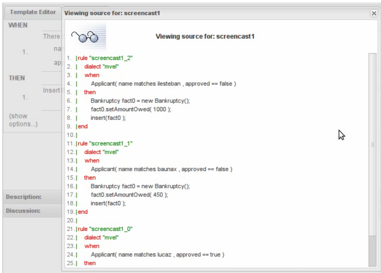
Figure 4.113. Each Row generates a Rule
