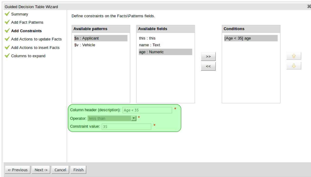
Figure 4.44. Defining Limited Entry constraints with the Wizard
