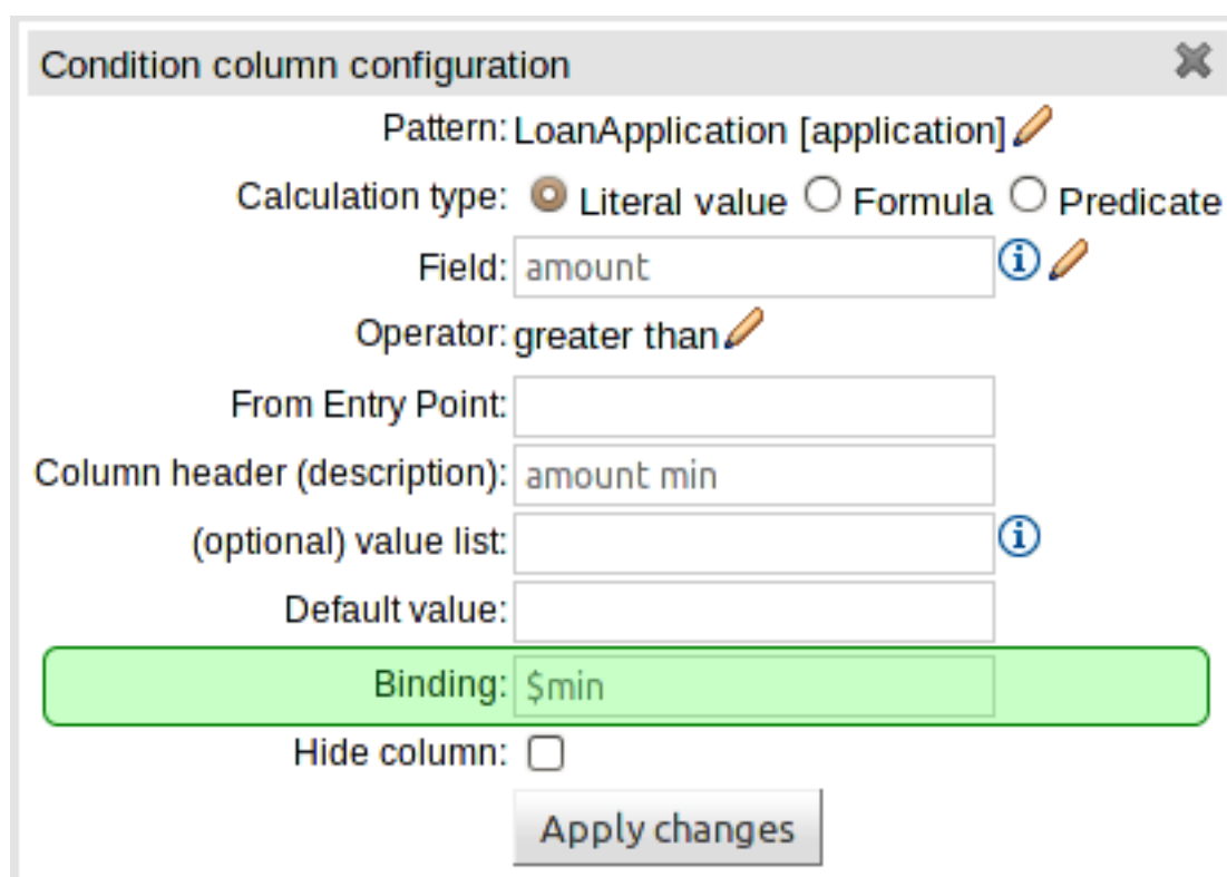
Figure 4.54. Binding a field
