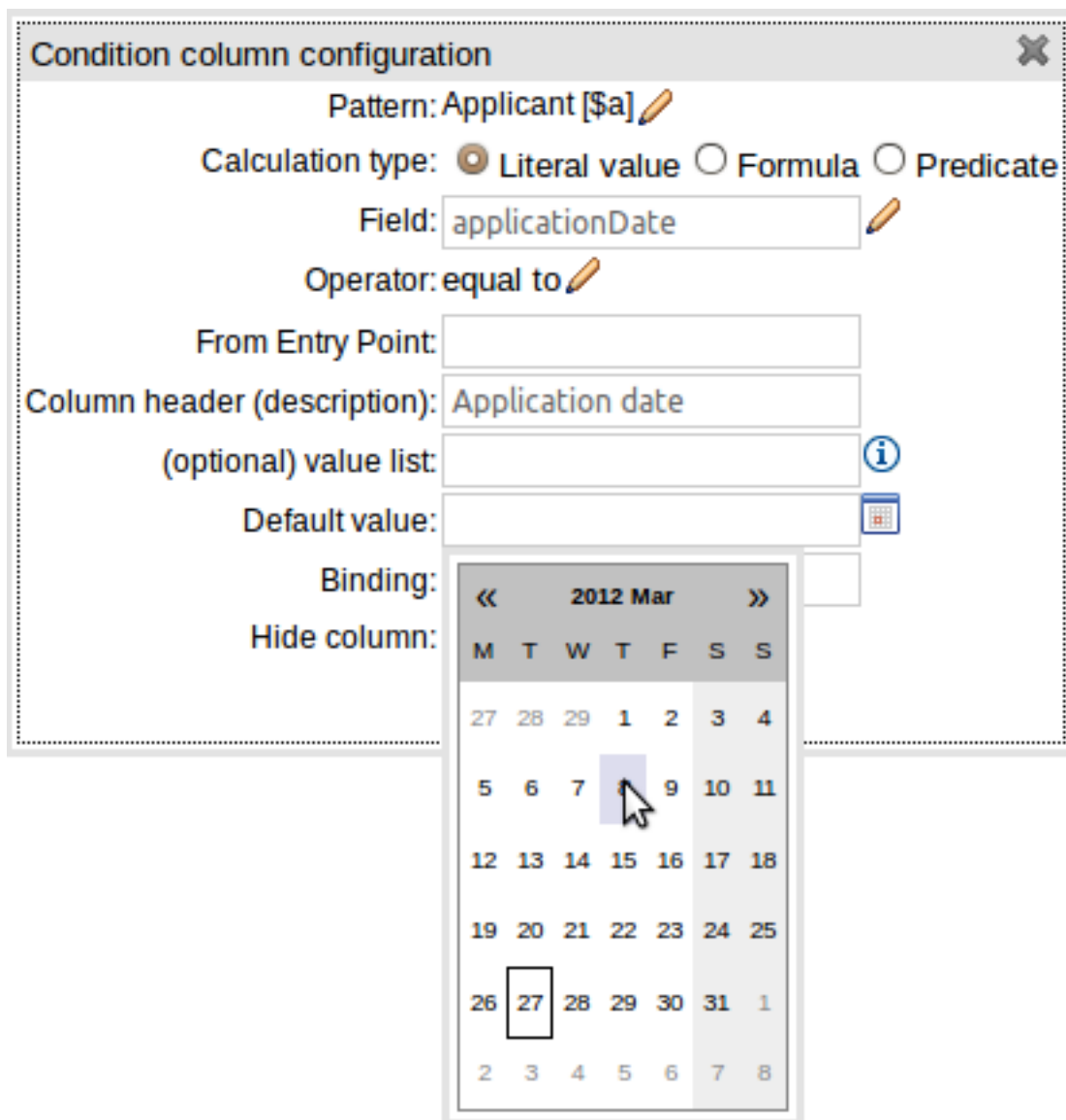
Figure 4.72. Setting the default value of a Date column
