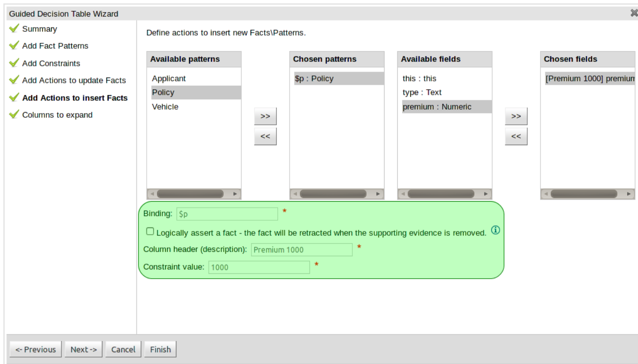
Figure 4.45. Defining Limited Entry actions with the Wizard
