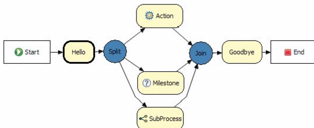
Figure 4.135. Current active nodes in a workflow in a specific breakpoint
