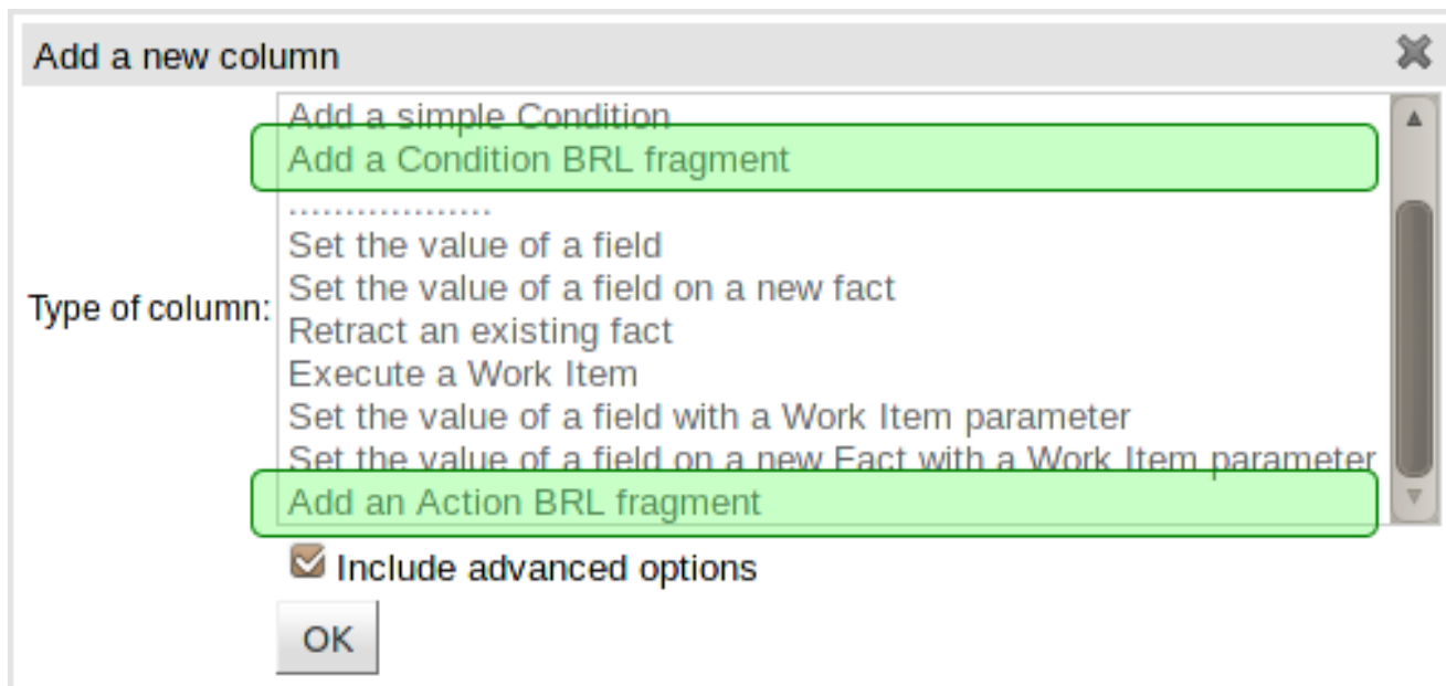
Figure 4.59. Adding a BRL fragment
