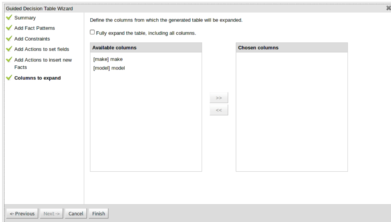
Figure 4.89. Choose how rows are created - select the columns you want to expand upon
