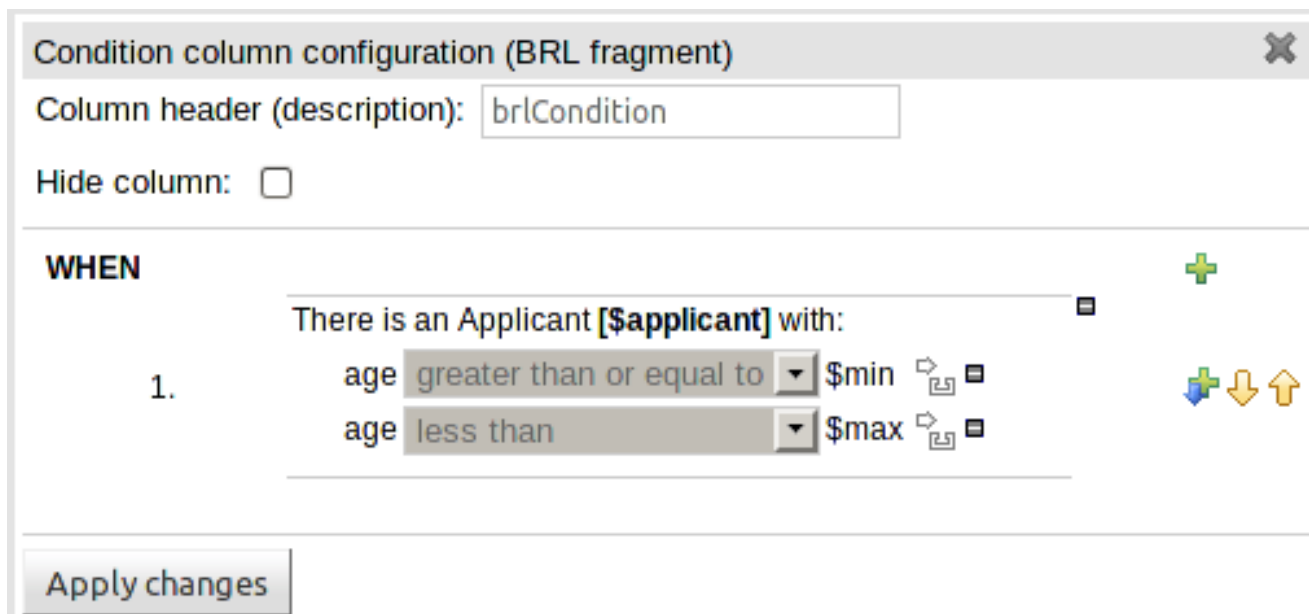
Figure 4.60. A Condition BRL fragment
