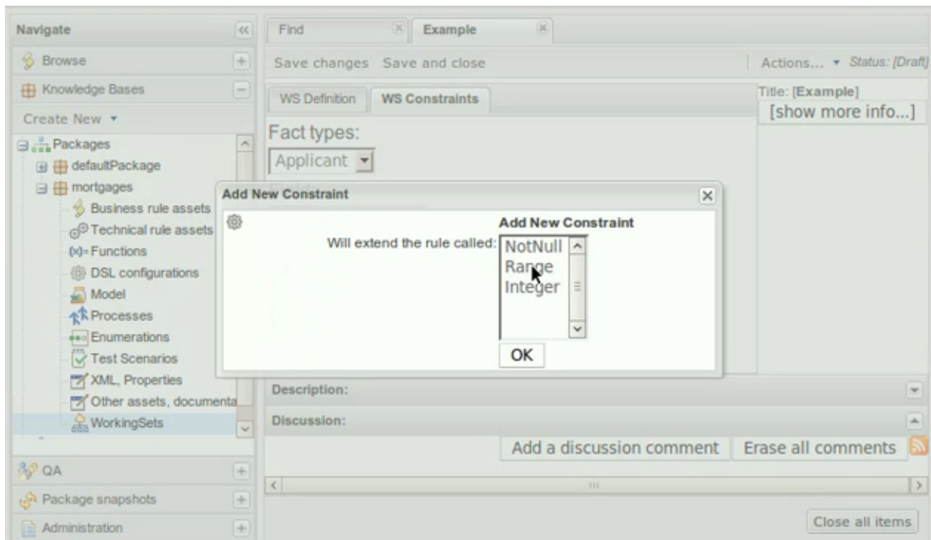
Figure 4.120. Selecting the type of field constraint
