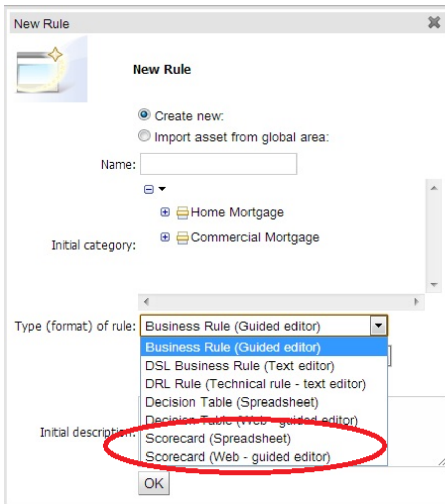
Figure 4.39. New Rule Dialog with New Asset Types
