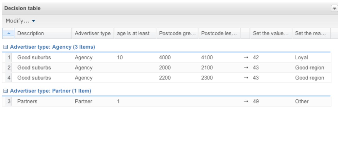
Figure 4.129. Web based decision table editor
