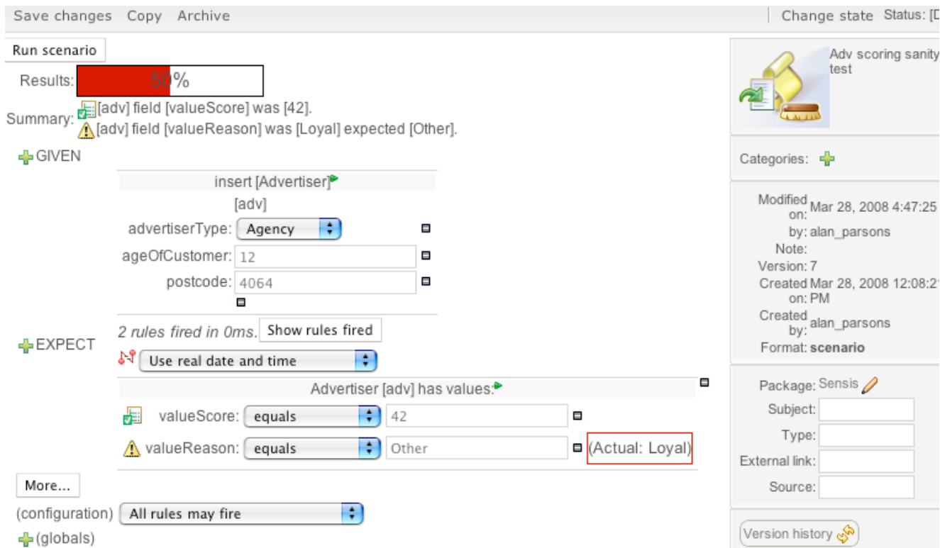
Figure 4.131. Running single scenario
