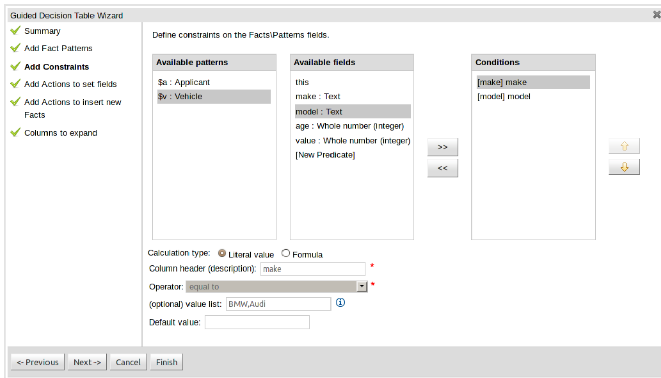
Figure 4.85. Add constraints to facts
