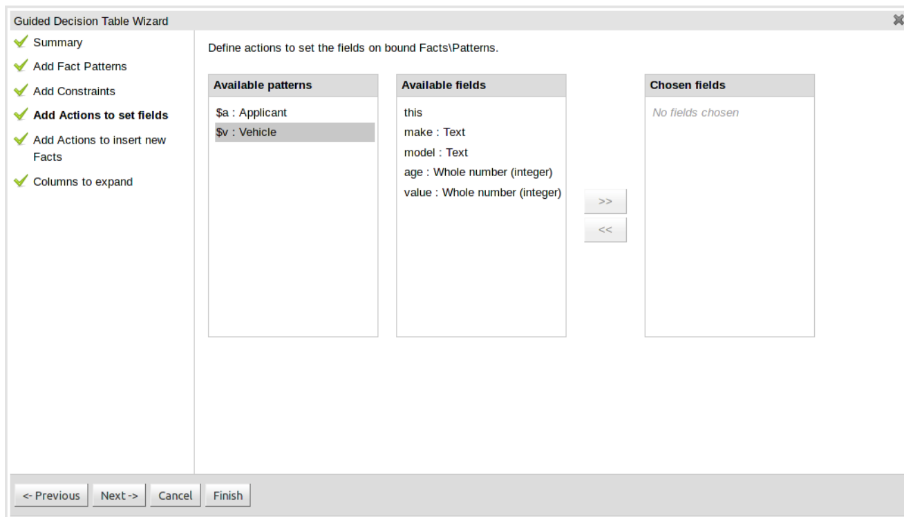
Figure 4.86. Add actions to set fields on bound facts
