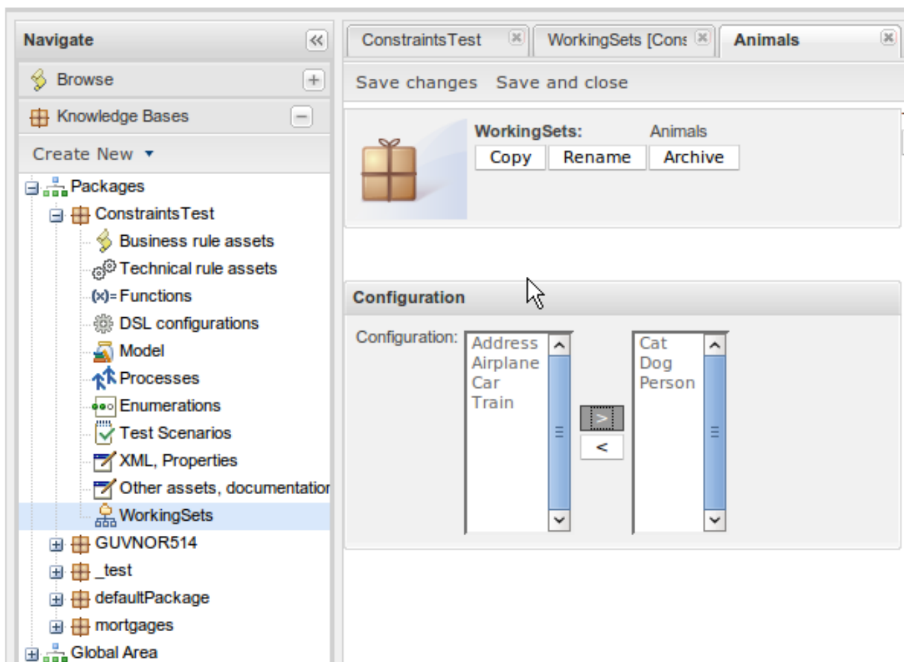
Figure 4.115. Create Animals Working Set
