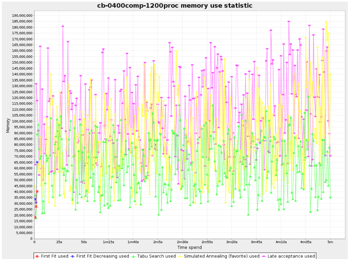
Figure 13.6. Memory use statistic
