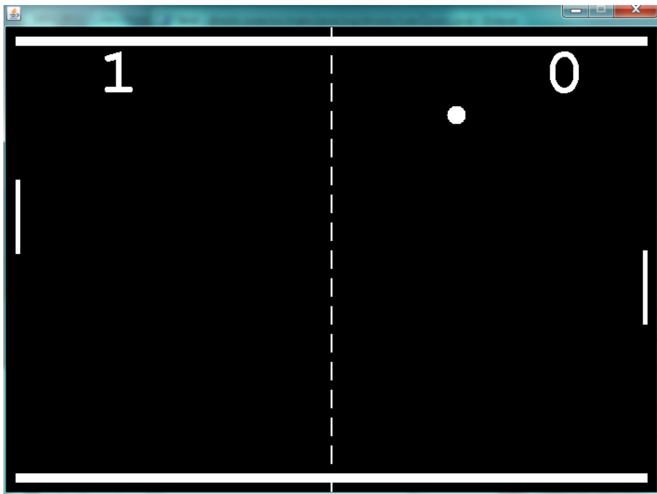
Figure 19.30. Pong Screenshot
