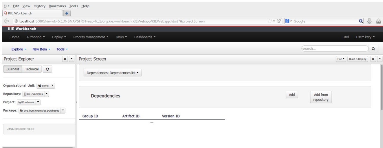
Figure 15.67. Project editor.
