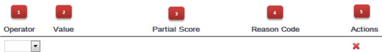
Figure 16.52. New Attribute
