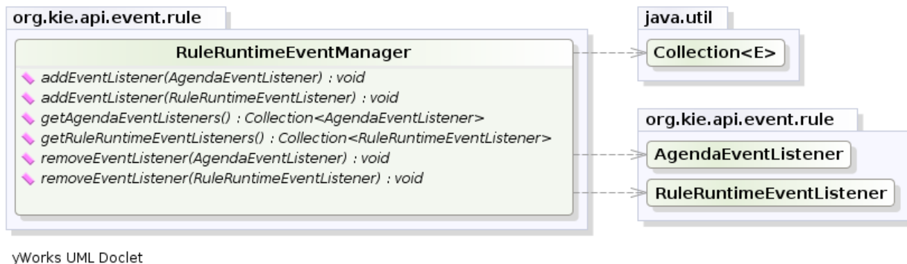
Figure 4.19. RuleRuntimeEventManager
