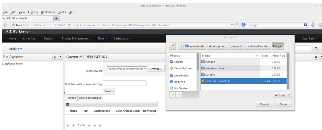
Figure 15.72. File browser.
