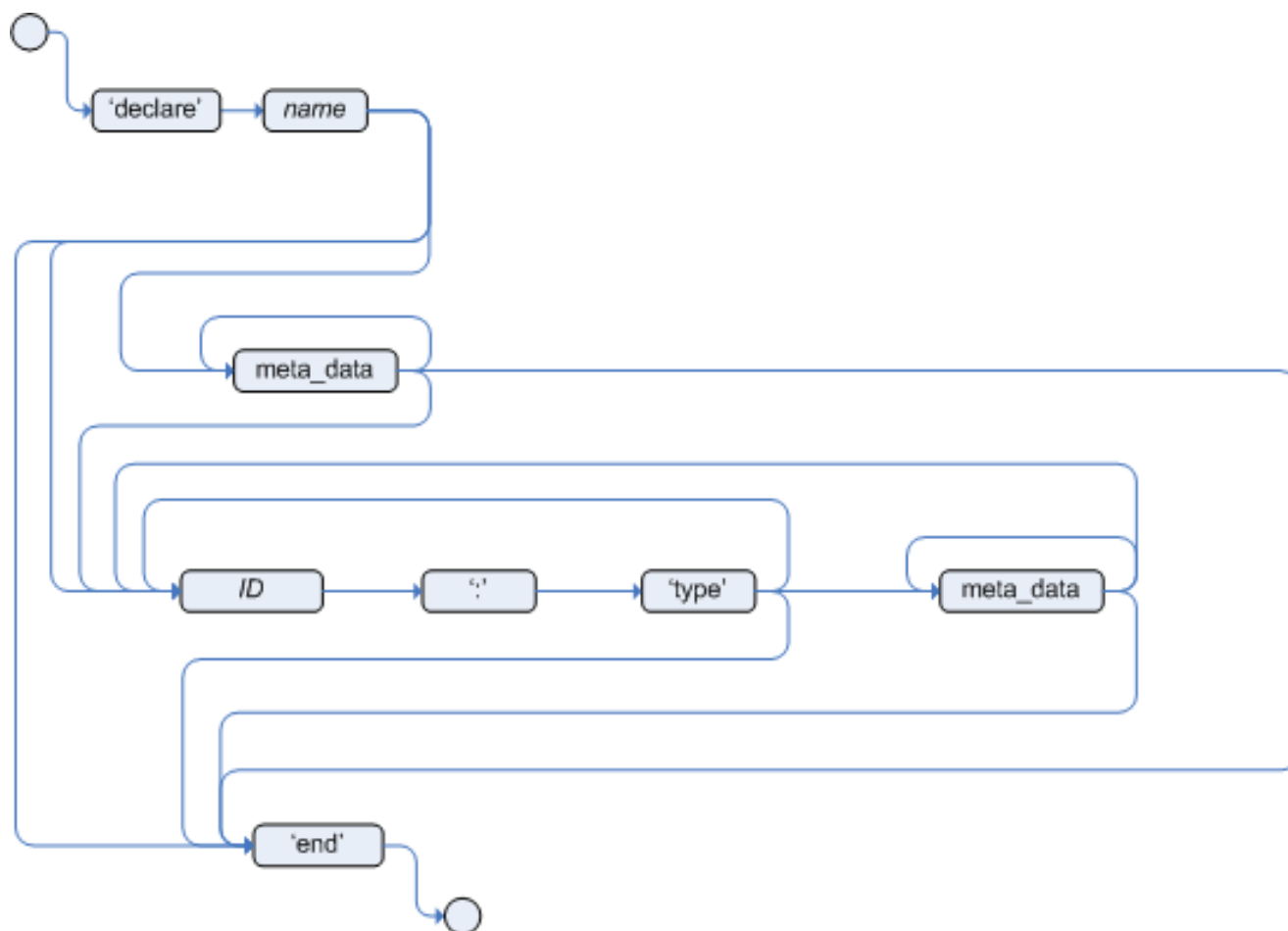
Figure 7.8. type_declaration
