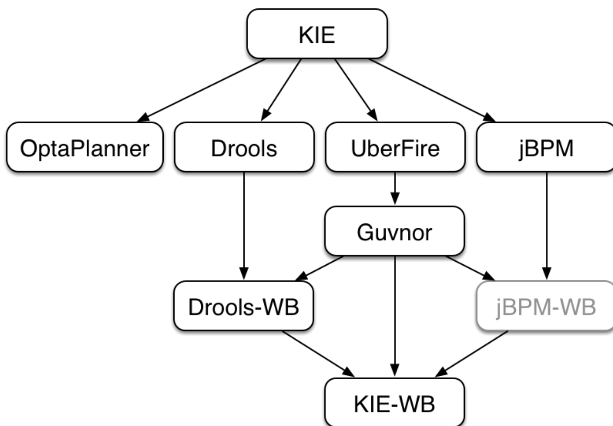
Figure 2.41. KIE Anatomy
