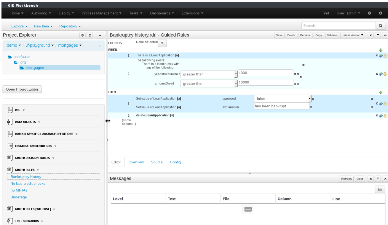
Figure 18.20. Resizing
