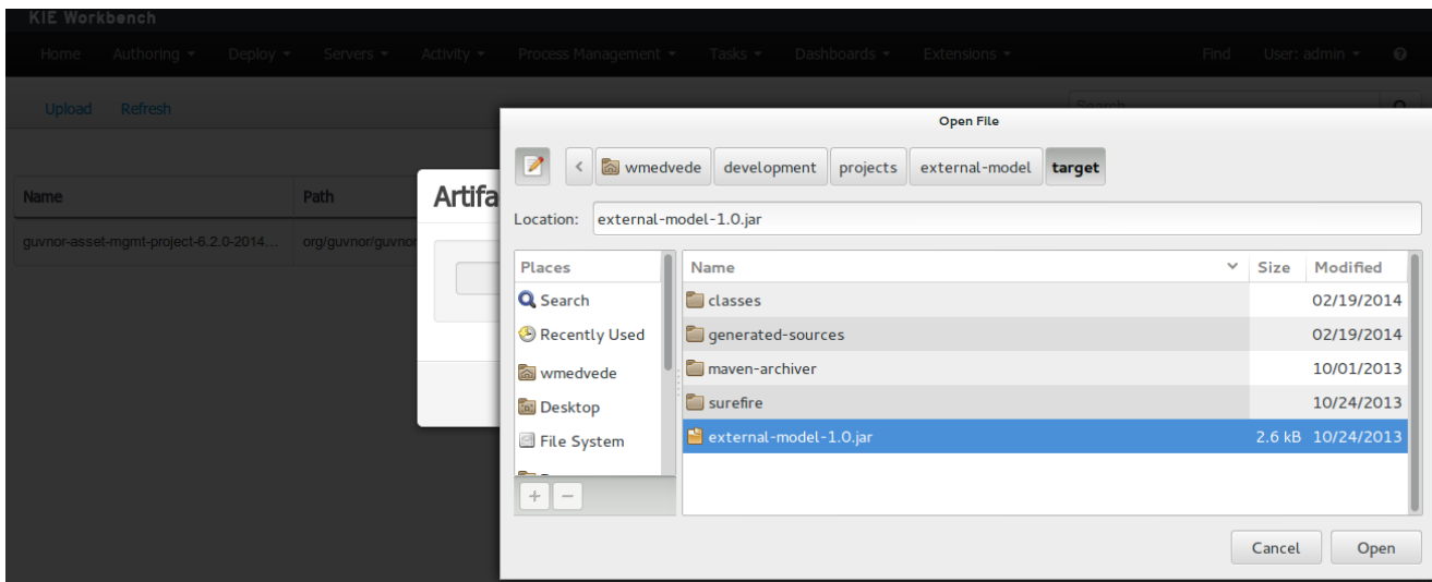
Figure 18.87. File browser.
