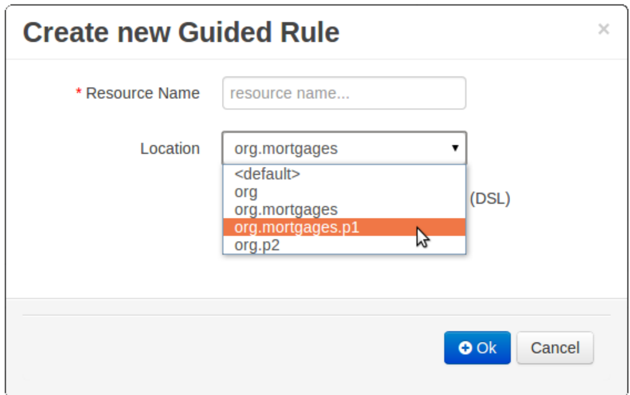
Figure 2.31. Package selector
