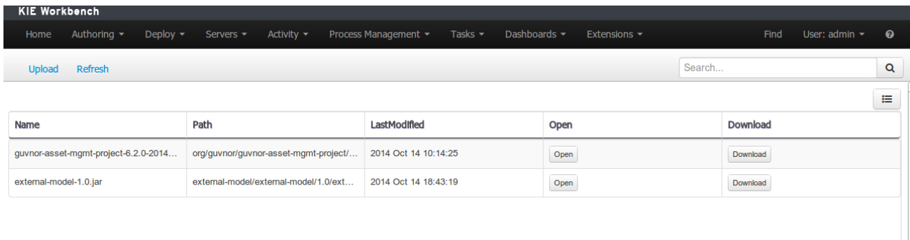
Figure 18.89. Files list.
