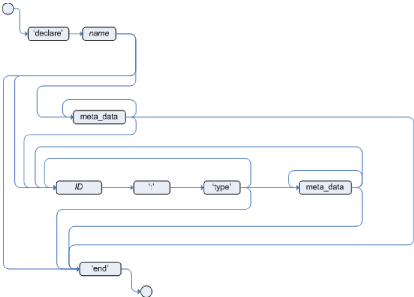
Figure 8.8. type_declaration
