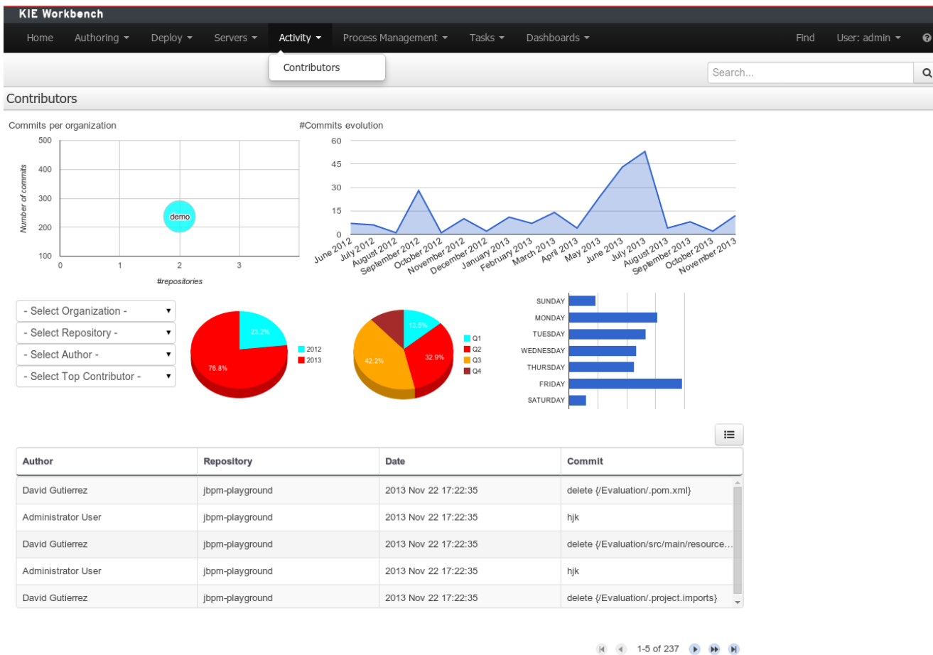
Figure 2.30. Contributors perspective
