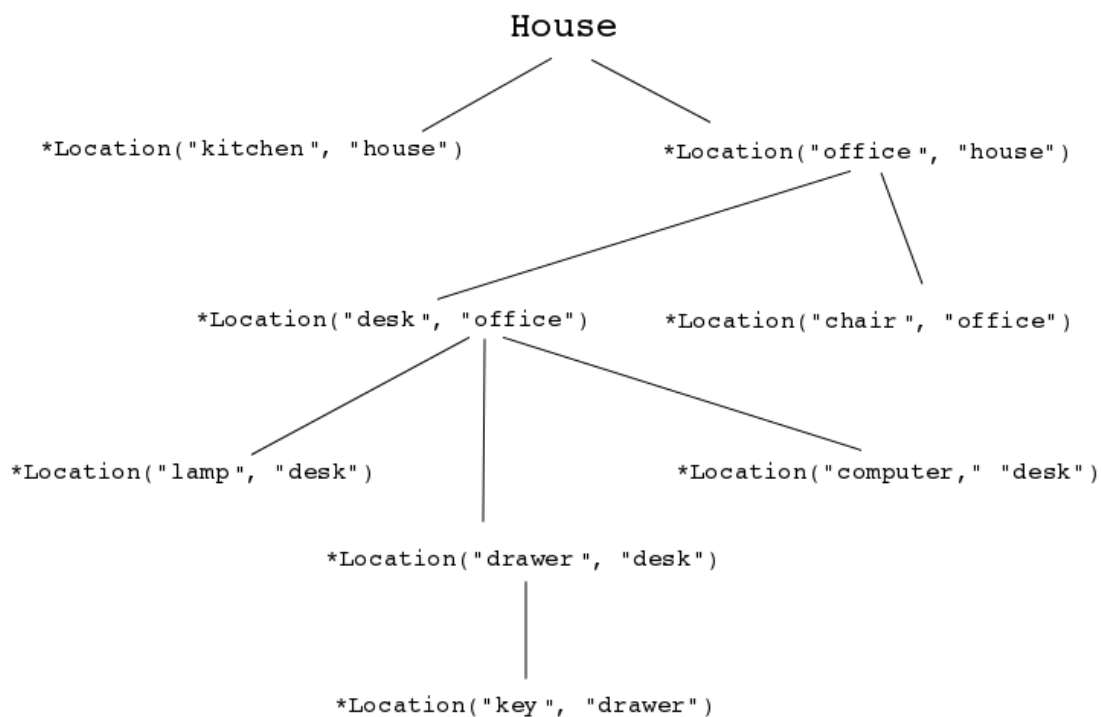
Figure 23.44. Reasoning Graph
