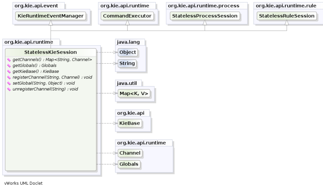
Figure 4.24. StatelessKieSession
