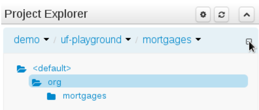
Figure 18.32. Showing packages
