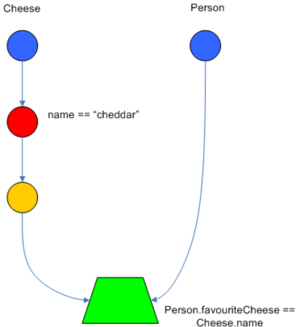
Figure 5.10. JoinNode
