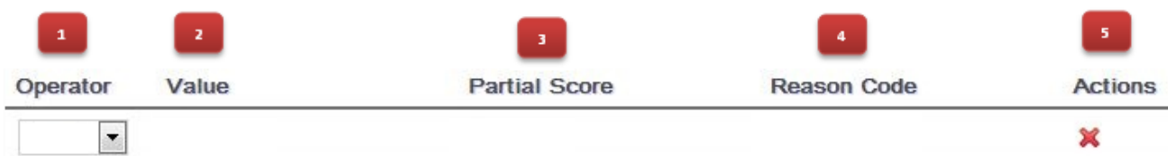
Figure 19.63. New Attribute
