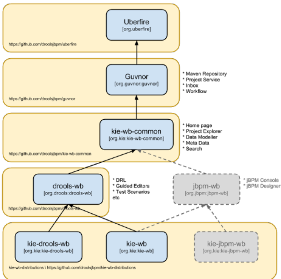
Figure 2.43. Module Structure
