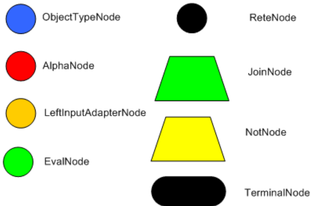
Figure 5.7. Rete Nodes
