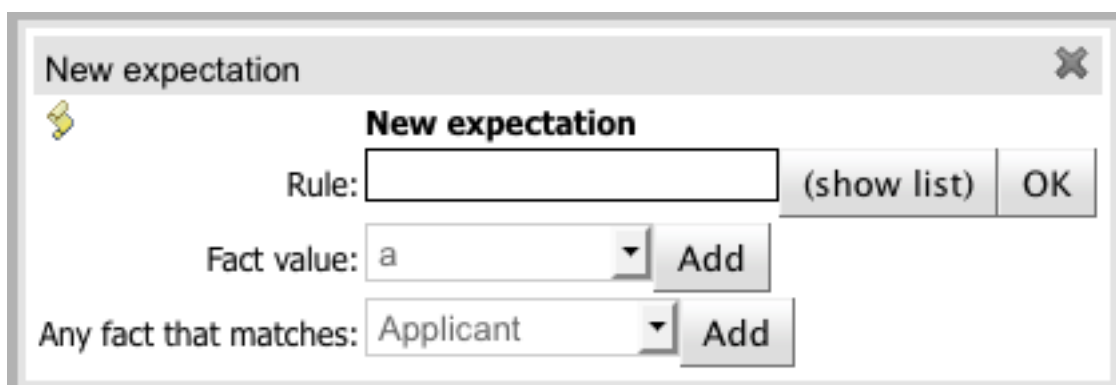
Figure 19.68. Expect popup
