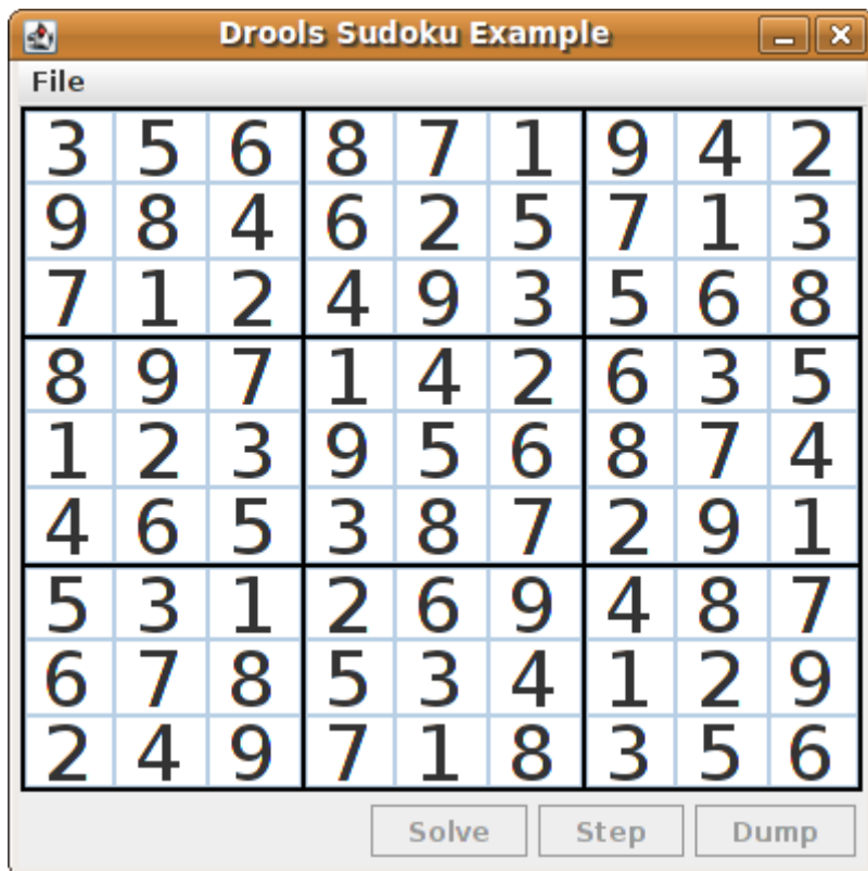
Figure 23.20. "Simple" Solved
