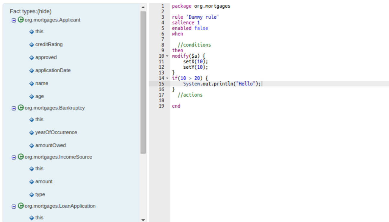
Figure 2.5. ACE Editor
