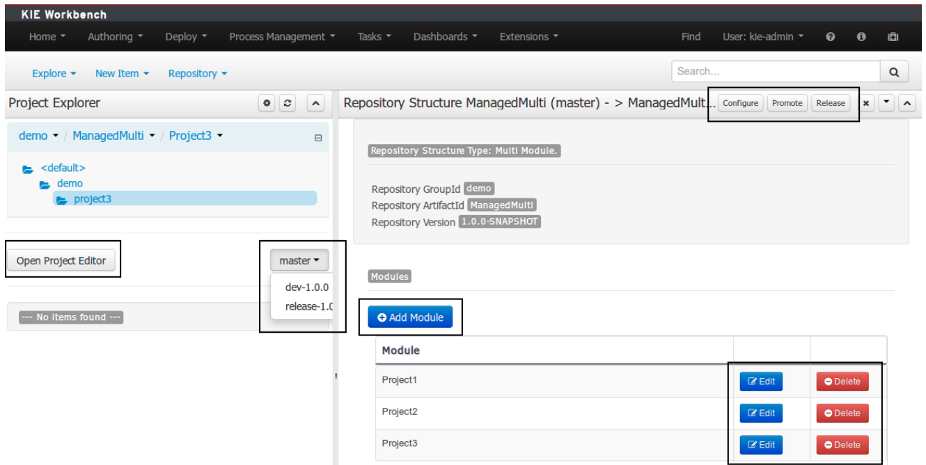
Figure 18.119. Managed Repositories Operations
