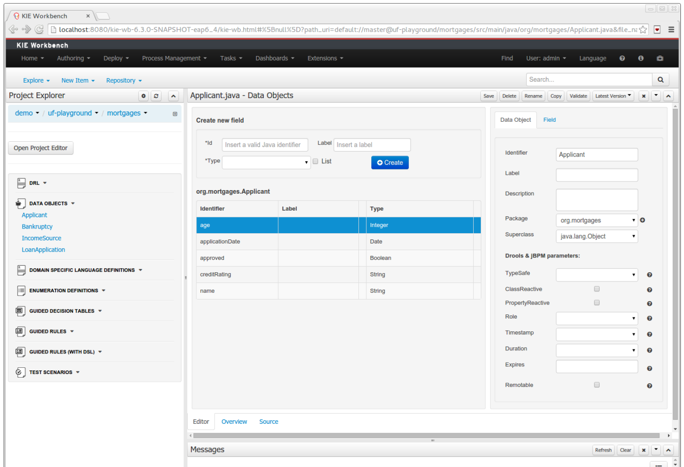
Figure 2.27. Improved Data Object Editor
